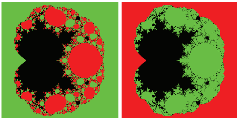
FIGURE 3. V_2 : The image on the left shows the maps whose free critical point is attracted to \infty in red, while the maps with attraction to 0 are colored green. The image on the right shows the type 2 hyperbolic component in red and the type 3 components in green. In both images the free critical point for the maps colored in black is not attracted to the critical cycle.
