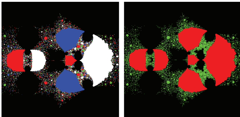
FIGURE 5. V_4 projected from (-1, 0) : The image on the left shows the maps whose free critical point is attracted to \infty , 0, 1, and 1 + b + c in red, green, blue, and white, respectively. The image on the right shows the type 2 components in red, while the green represents the type 3 components. In both images the free critical point for the maps colored in black is not attracted to the critical cycle.
