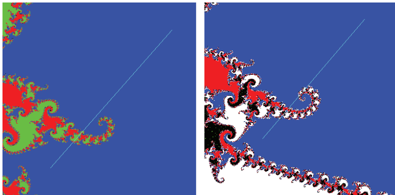
FIGURE 1. The image on the left shows the basins of attraction for the map f(z) = (z - c)(z - 1)/z^2 where c = .16 - 2.2i . The free critical point is attracted to 1 under iteration of f^3 in this case; but, as is illustrated, the line segment joining the free critical point and 1 is not entirely contained in the immediate basin. The image on the right shows a similar situation for a map in V_4 .
