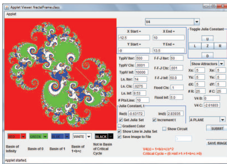
FIGURE 8. Screenshot: The basins of attraction for a type 2 map f in V_4 . The free critical point is attracted to \infty under iteration of f^4 . The line segment fails to connect the free critical point with \infty .
