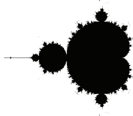
FIGURE 2. V_1 : The single type 1 component is in white. Since \infty is a fixed critical point there are no maps of types 2 or 3. The free critical point, for the maps colored in black, is not attracted to \infty .
