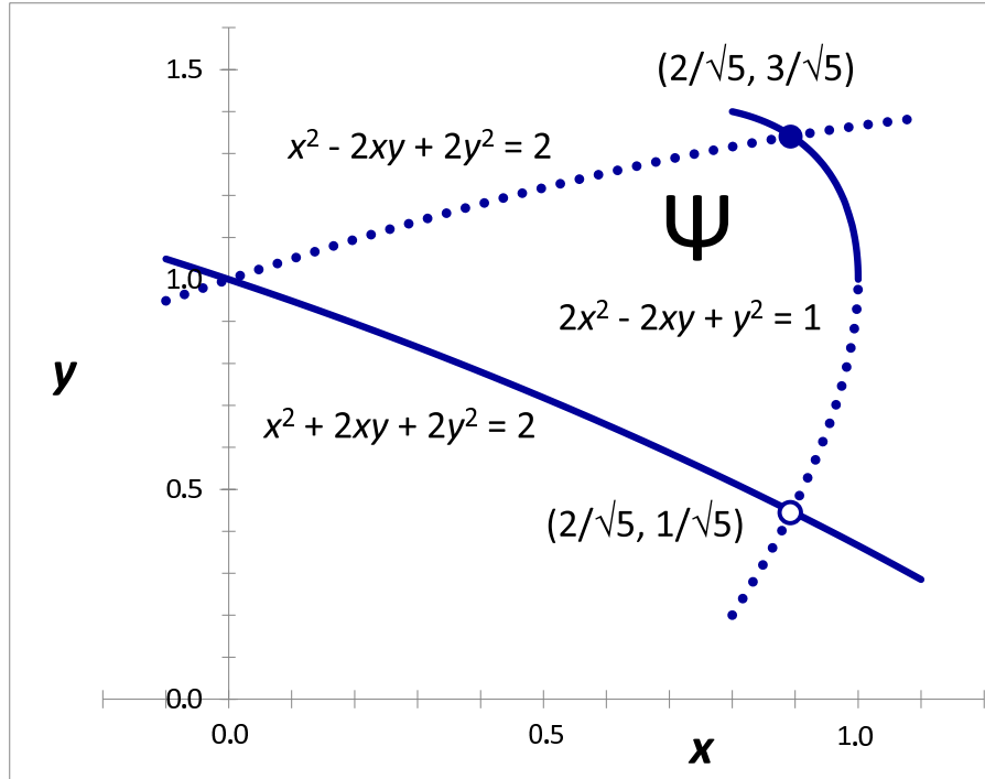
FIGURE 2. The region \Psi
