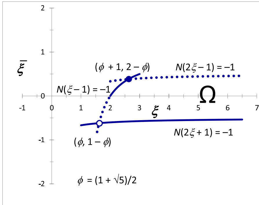
FIGURE 1. The region \Omega
