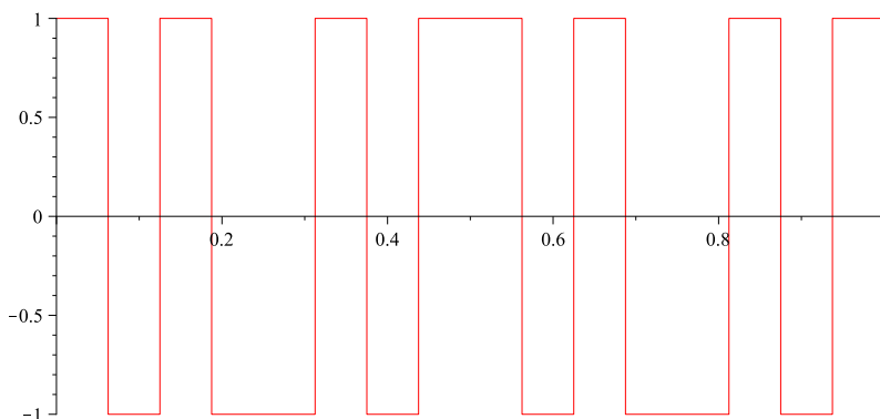
FIGURE 1. The Walsh-Paley function \omega_{10}
