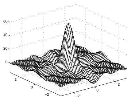
(a) The trigonometric Dirichlet kernel
