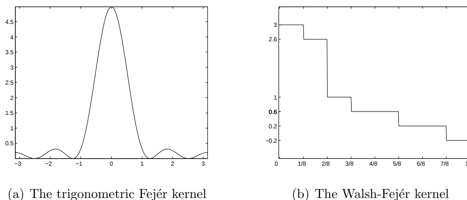
FIGURE 3. The Fejér kernels K_n with n = 5 .
