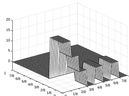
(b) The Walsh-Dirichlet kernel
