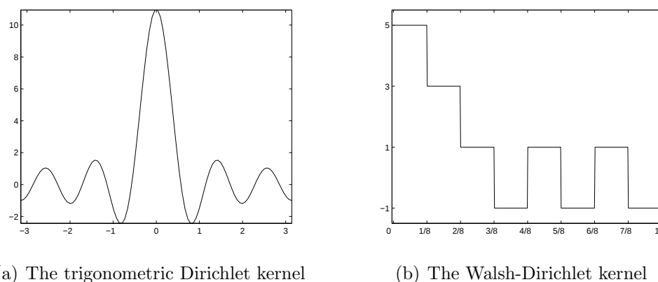
FIGURE 2. The Dirichlet kernels D_n with n = 5 .
