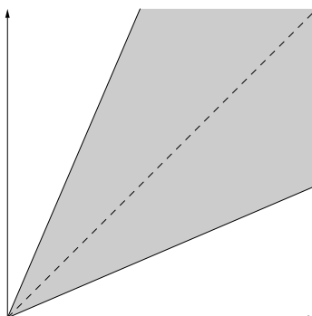
FIGURE 6. The cone for d = 2 .
