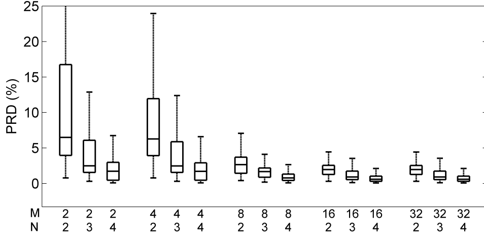
FIGURE 2. Box plot of PRD approximation errors with respect to the parameters M (top) and N (bottom). The outliers are not shown.
