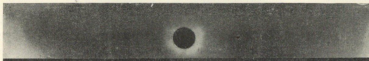
10/c ábra. \gamma\text{-Al}_2\text{O}_3 + 1\% \text{MoO}_3
