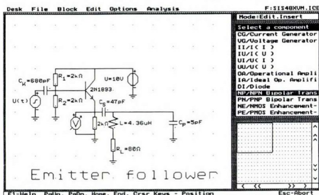
Fig. 4.1. Emitter follower
