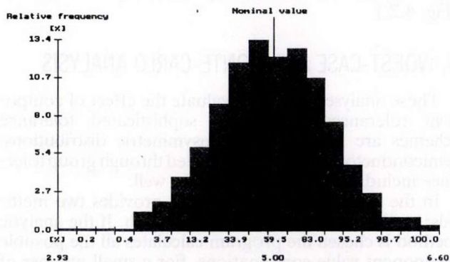
Fig. 5.2. Monte-Carlo analysis with 5% group tolerance
