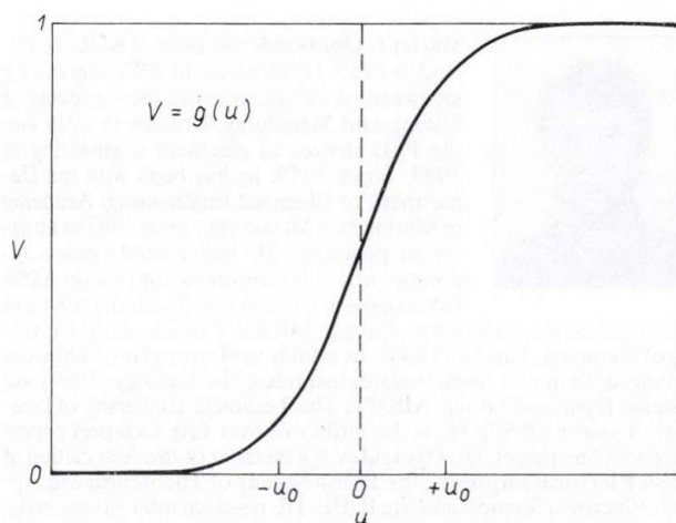
Fig. 1.b. The nonlinear monotonic input-output relation of the amplifiers [2]
