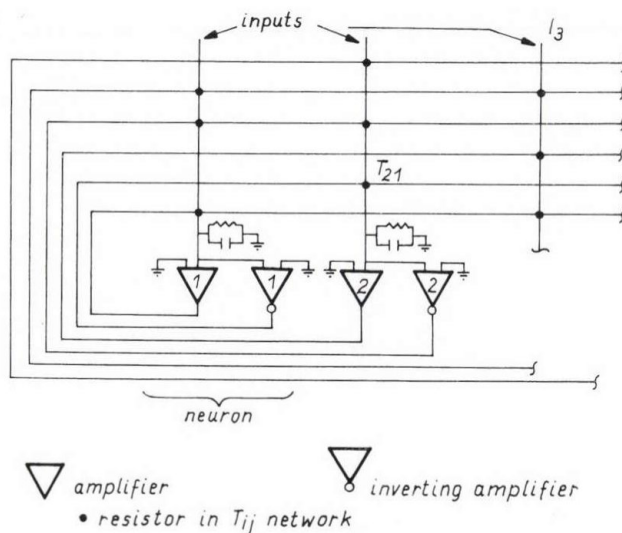
Fig. 1.a. The Hopfield-network. The circles at intersections correspond to resistive connections ( T'_{ij} 's). Connections between inverted outputs and inputs represent negative (inhibitory) feedback
