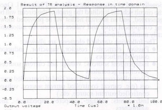
Fig. 3.4. Transient response of a differential amplifier
