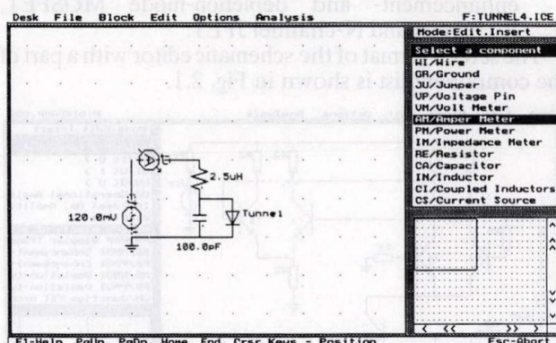
Fig. 3.5. Tunnel diode oscillator
