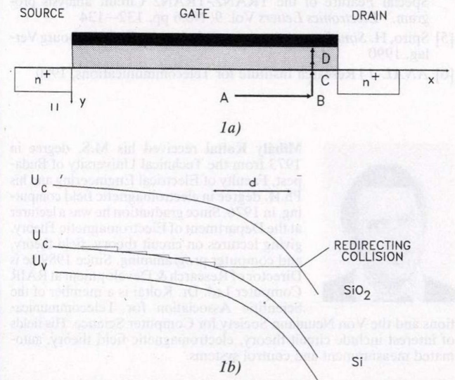
Fig. 1. (a) cross-sectional view of the MOSFET illustrating the scattering probabilities in the model.
