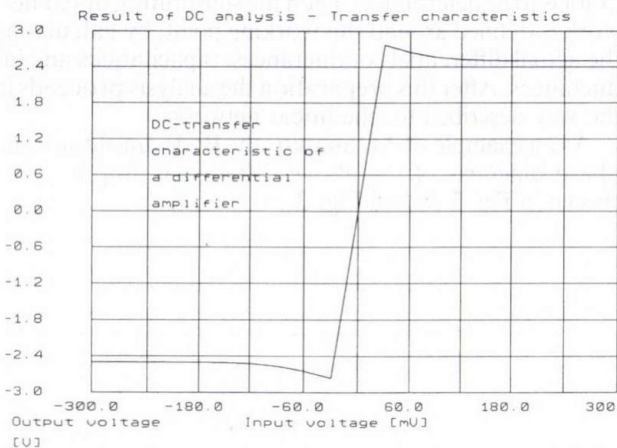
Fig. 3.1. DC transfer characteristic of the differential amplifier in Fig. 2.1.
