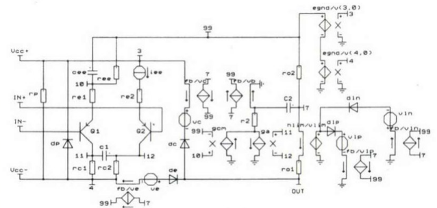
Fig. 6.7. The macromodel of OPAMP
