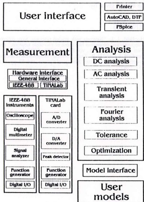
Fig. 1.1. The block diagram of TINA
