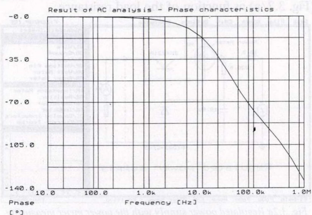
Fig. 3.3b Phase diagram
