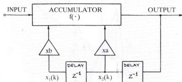
Fig. 6. Second order digital filter
