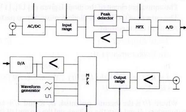
Fig. 8.1. Block Diagram of the TINA-Lab1 measurement card
