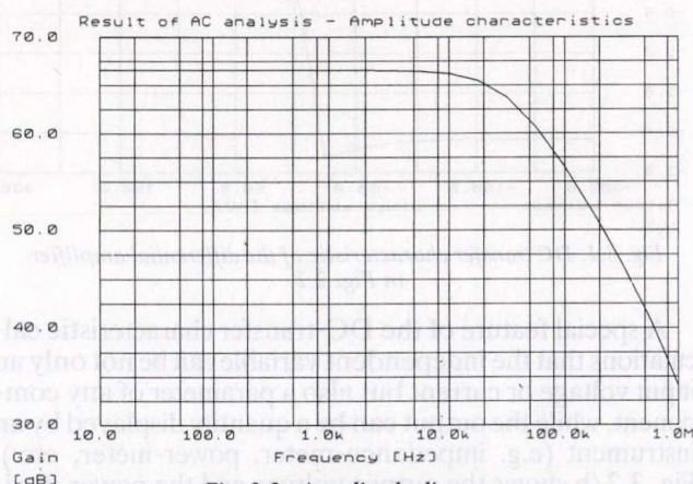
Fig. 3.3a Amplitude diagram
