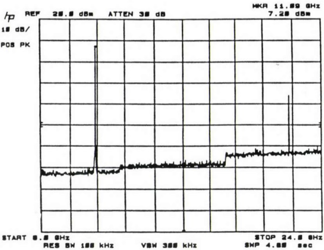
Fig. 24. Measured spectrum of an investigated oscillator
