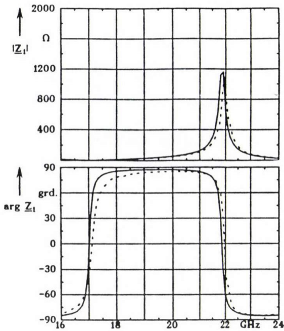
Fig. 13. Magnitude and phase of the impedance of a slot line resonator versus frequency (the third parallel resonance is visible in the upper part). w_{slot}=100\text{ }\mu\text{m} , l_{slot}=8711\text{ }\mu\text{m} , thickness of dielectric: 250\text{ }\mu\text{m} , \epsilon=9.8 (solid line-calculated, dotted line-measured)
