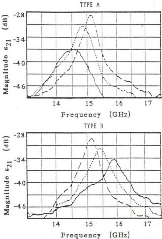
Fig. 14. Resonant frequency shift due to the total length of each air bridge of 10 \mu\text{m} (dotted line) and 50 \mu\text{m} (solid line) compared to a reference CPW resonator without air bridges (dashed line)
