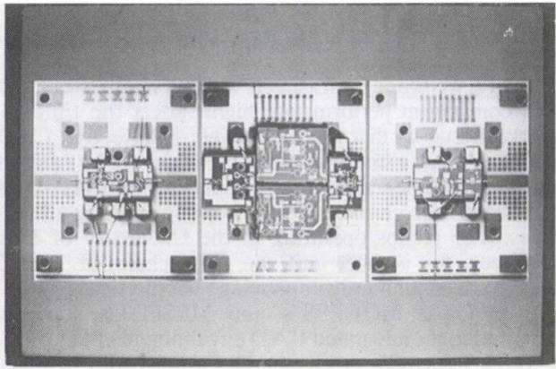
Fig. 23. THOMSON 5.9 to 8.5 GHz direct demodulation front-end receiver
