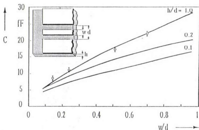
Fig. 7. Calculated equivalent capacitances of an open-ended coplanar waveguide ( \epsilon_r = 9.8 , h = 635 \mu\text{m} , t = 0 ) together with measured values for h/d = 1.0
