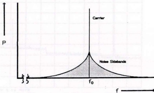
Fig. 25. Spectrum of an oscillator near carrier
