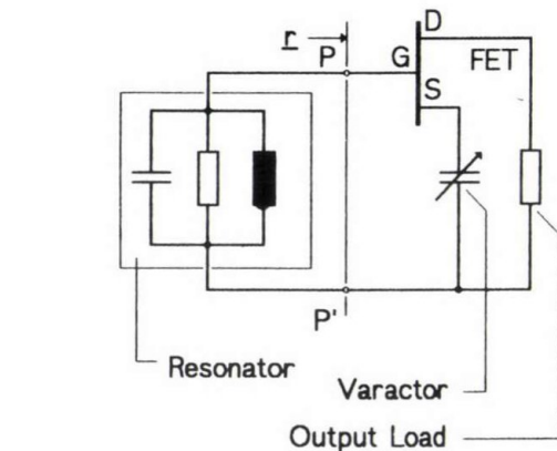
Fig. 6. Equivalent circuit of the oscillator shown in Fig. 5.
