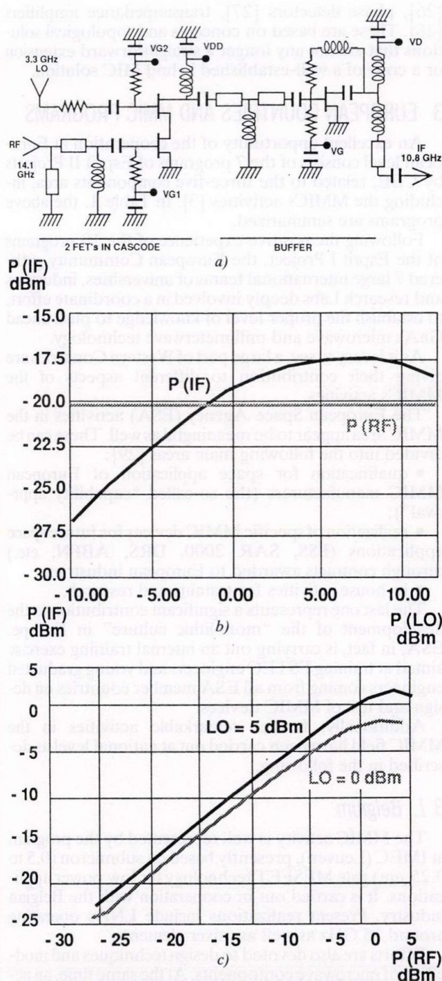
Fig. 1. ALCATEL-ESPACE 14/12 GHz active mixer: a) schematic; b), c) conversion performance
