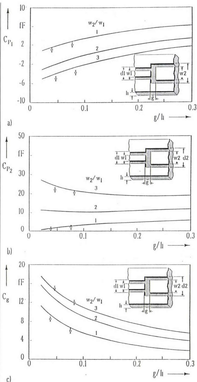
Fig. 9. Equivalent circuit capacitances of a symmetric gap between two 50\Omega coplanar waveguides of different dimensions ( \epsilon_r = 9.8 , h = 635 \mu\text{m} , w_1/h = 0.2 , w_1/d_1 = d_2 = 0.56 , t = 0 ) together with measured values
