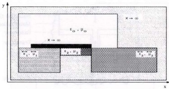
Fig. 8. A transverse structure with isotropic and anisotropic subsections
