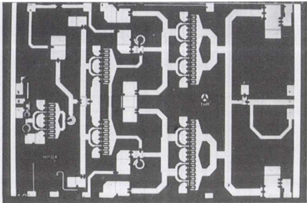
Fig. 22. THOMSON X-band power amplifier
