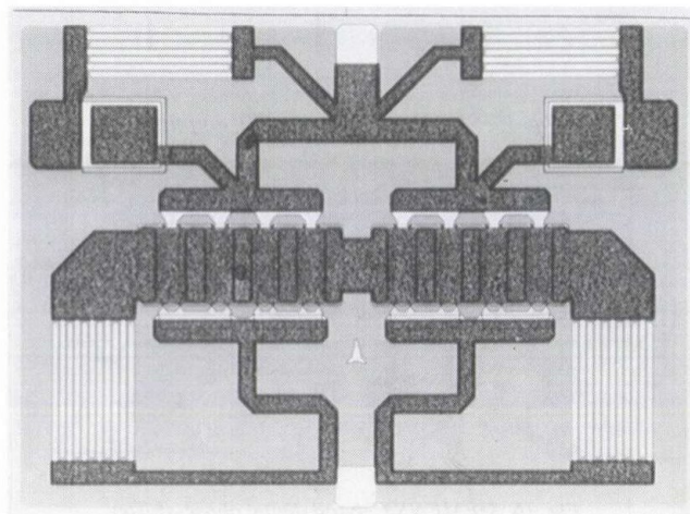
Fig. 14. SELENIA X-band power amplifier
