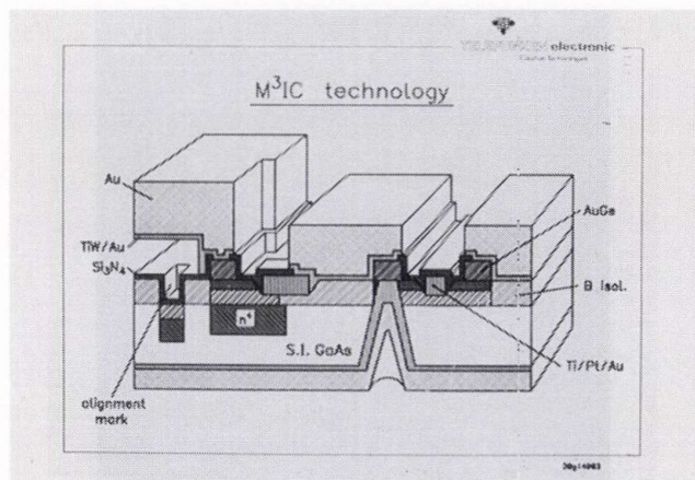
Fig. 18. TELEFUNKEN technology for diode and MESFET single process sequence
