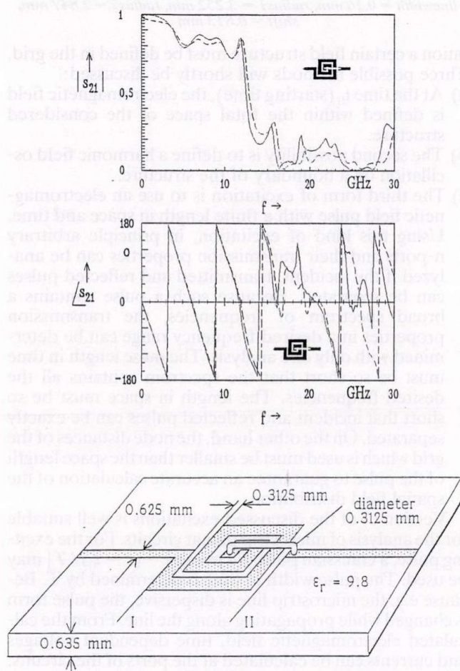
Fig. 18. The spiral inductor and the calculated (—) and measured (---) transmission coefficient of the spiral inductor. The dimensions of the inductor have been chosen to be very large so that resonance effects could be measured in the frequency range up to 30 GHz
