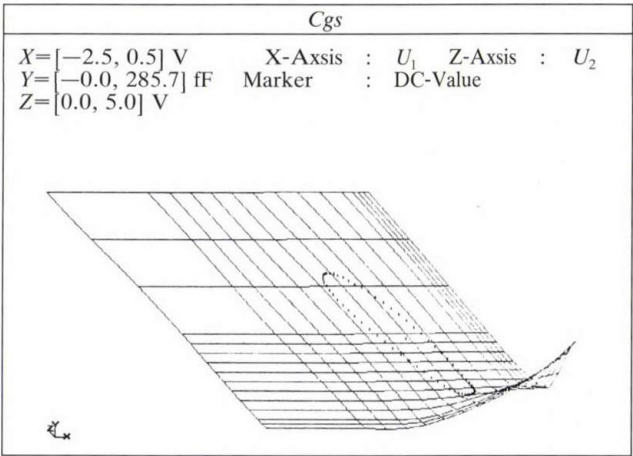
Fig. 22. Nonlinear behaviour of C_{ds}
