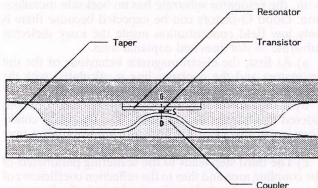
Fig. 18. Layout of an oscillator in slot line technique
