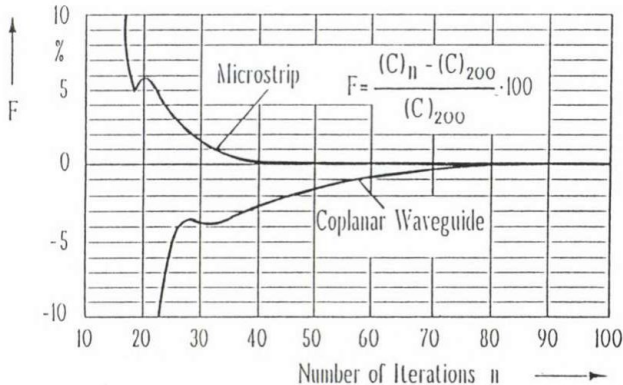
Fig. 2. Relative error of equivalent open-end capacitance as a function, of iteration number
