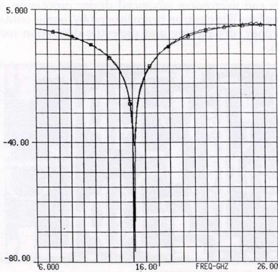
a) Fig. 25. Simulated and measured magnitude S_{21} for 10 Mil alumina. a) LS=80 mils; b) LS=60 mils
