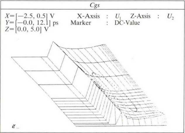
Fig. 23. Nonlinear behaviour of time constant \tau
