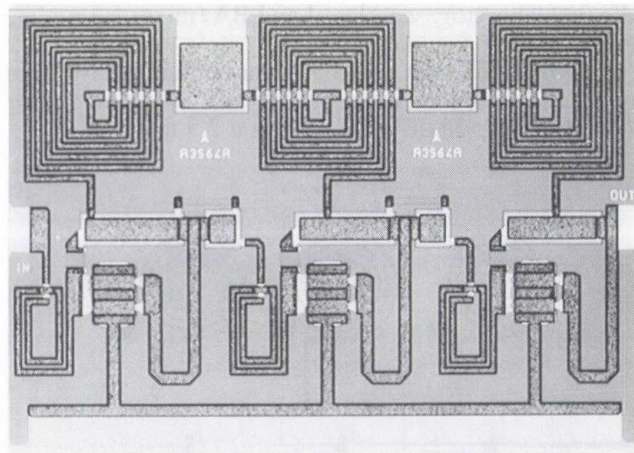
Fig. 13. SELENIA 2 to 6 GHz feedback amplifier
