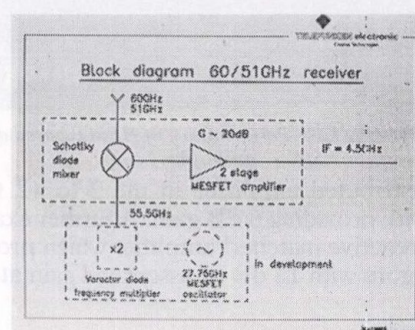
Fig. 19. TELEFUNKEN 60 GHz receiver
