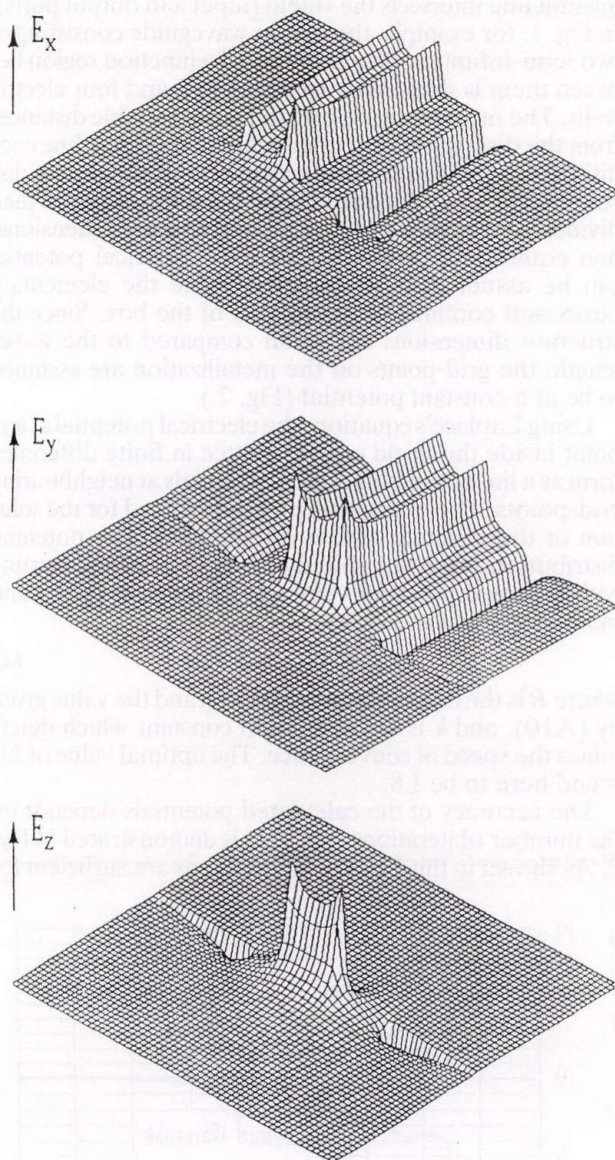
Fig. 6. Electric field components in the conductor plane of an open-ended coplanar waveguide supporting a TEM-wave
