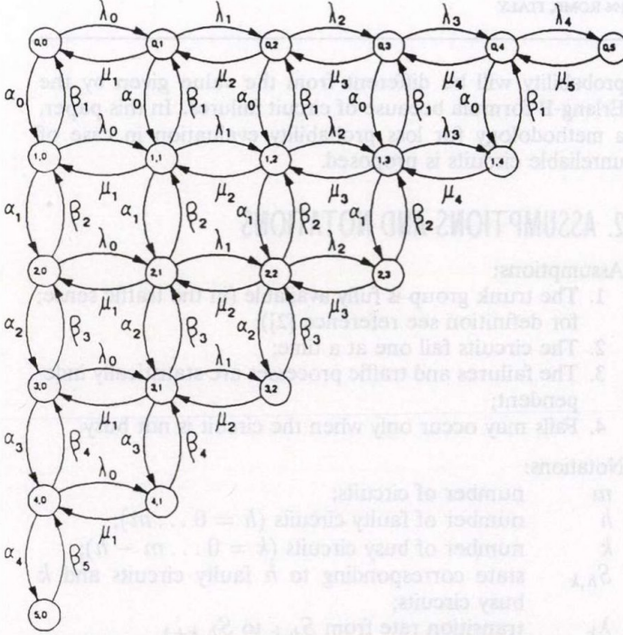
Fig. 2. Two-dimensional state transition-rate diagram, m = 5
