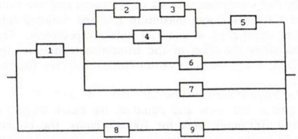
Fig. 3. The reliability block diagram of the example
