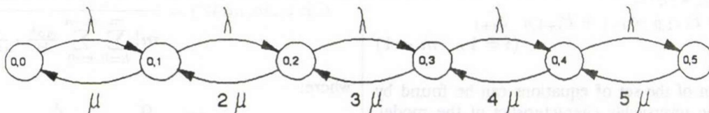
Fig. 1. One-dimensional Markovian model for an M/M/5/0/\infty process
