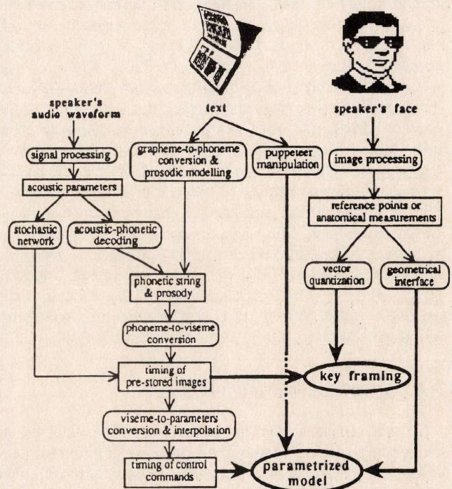
Fig 2. General scheme of Facial Animation showing the possible techniques.
