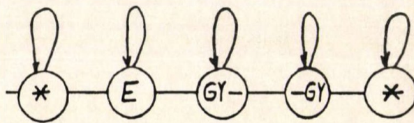
Fig. 9. The Markov model of the Hungarian word "EGY"
