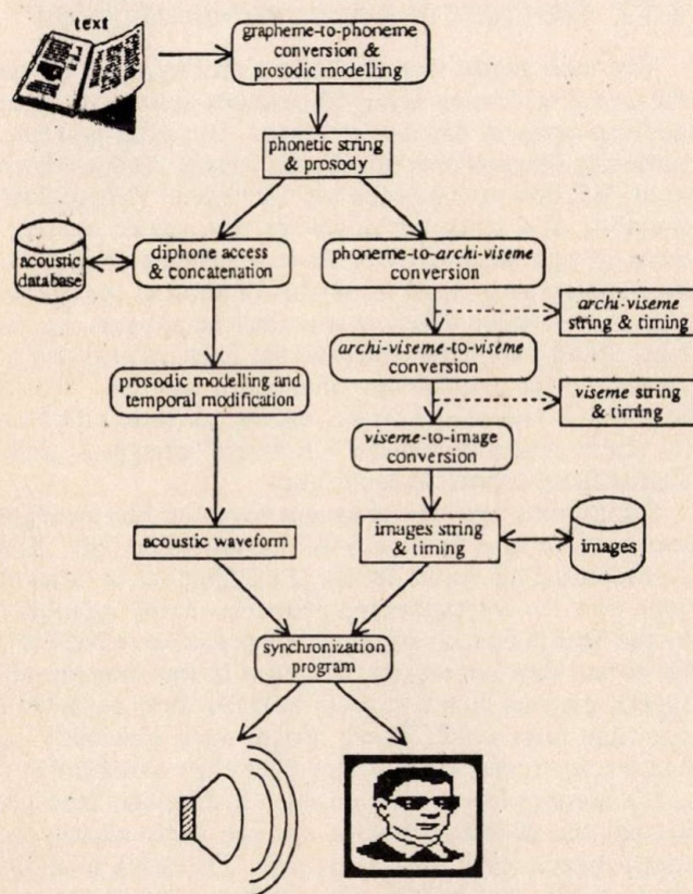
Fig. 3. Simplified principle of the ICP Text-to-Audio-Visual-Speech synthesizer
