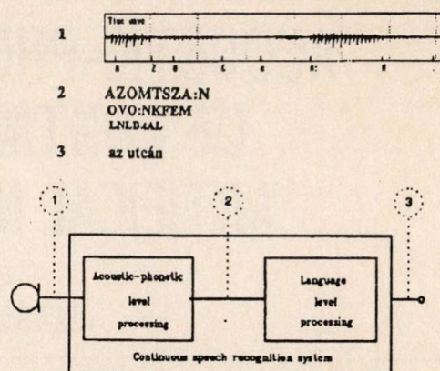
Fig. 1. The basic structure of the recognition system and the different representations used. The input is the speech waveform (representation 1). The output of the acoustic—phonetic unit is a string of phoneme candidates (representation 2). For each segment, the probability of the phoneme candidates is indicated by the character size, large for the first candidates and smaller for the second and third candidates. This level does not indicate any word boundaries. The output of the language unit is ordinary written text. The language processing unit is not included in this study.
