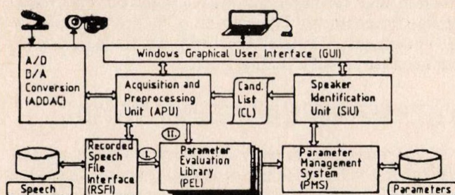
Fig. 1. Architecture of the speaker identification system
