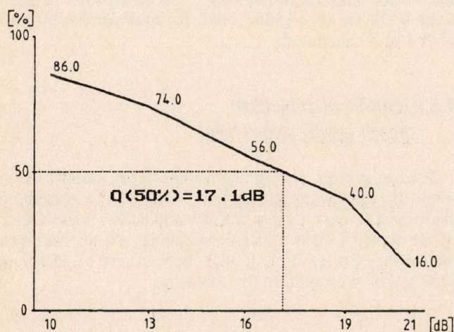
Fig. 3. The result for preference test for a 4800 bit/s CELP coder
