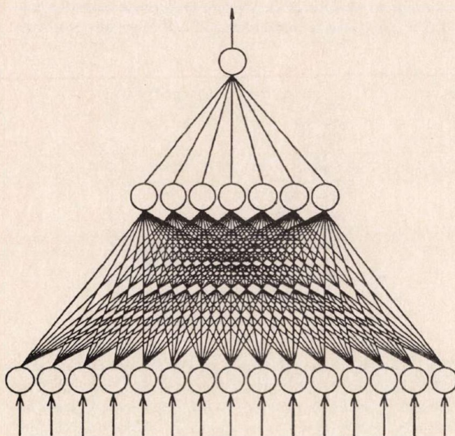
Fig. 10. The structure of the segmentation network with 15 input nodes, 7 hidden nodes and 1 output node.
