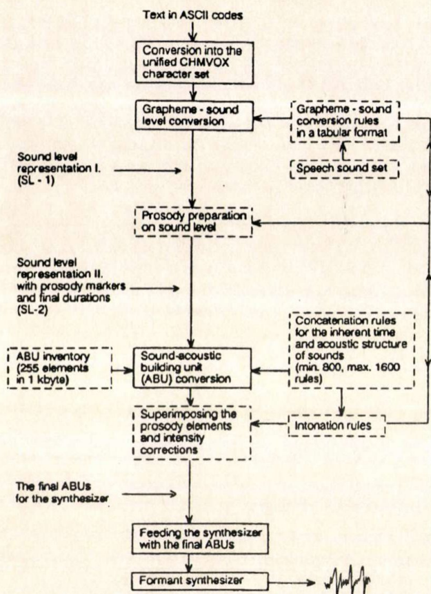
Fig. 1. The main building blocks of the MULTIVOX system
