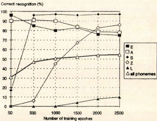
Fig. 12. The evolution of the phoneme recognition performance as a function of the training time for the Hungarian material. Each epoch means one presentation of all the training material.
