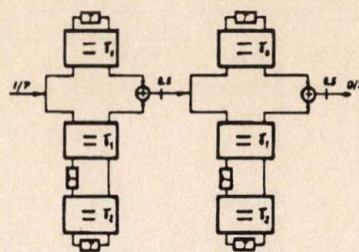
Fig. 10. WD realization of two lattices filter construction
