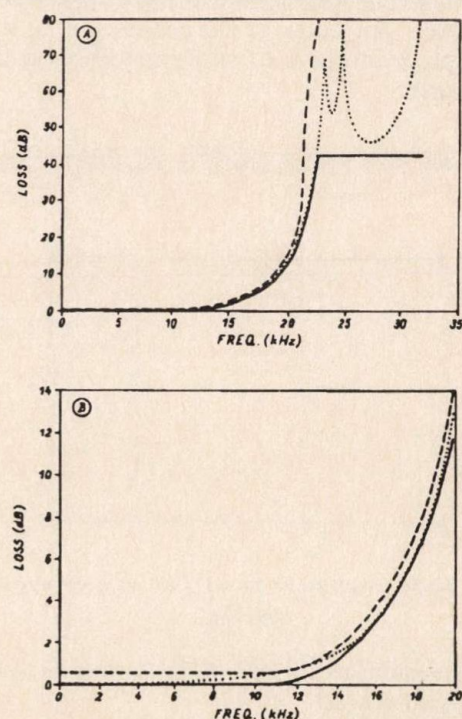
Fig. 5. Loss response of lattice + lattice filter construction (with the specification)
