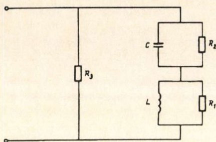
Figure 2. Reference circuit of the second order amplitude equalizer
