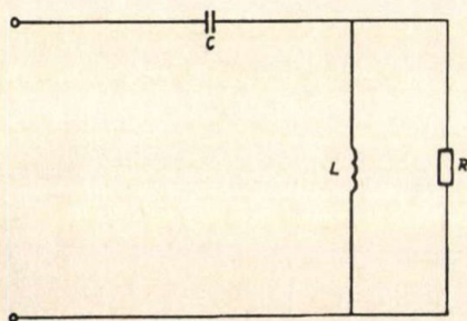
Fig. 3. Simplified reference circuit of second order amplitude equalizer
