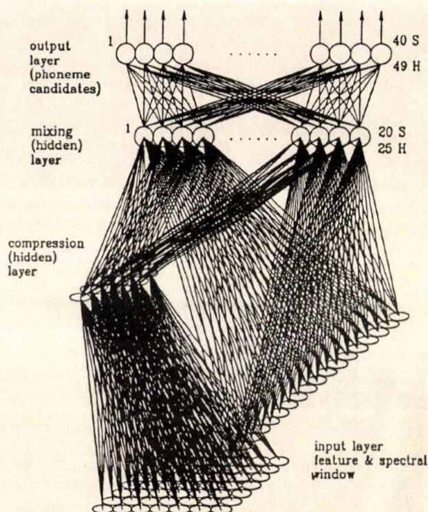
Fig. 7. The structure of the phone classification network. The Swedish network has 20 nodes in the mixing layer and 40 output nodes. The Hungarian network has 25 and 49 nodes, respectively.
