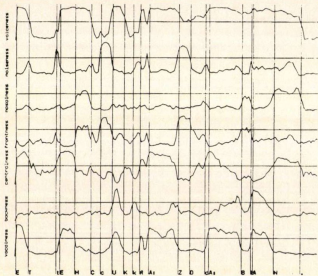
Fig. 11. Output activations of the coarse feature network as a function of time. Manually labelled segments. Horizontal lines indicate a 0.5 activation level for each feature.
