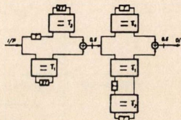
Fig. 11. WD realization of bireciprocal + lattice filter construction
