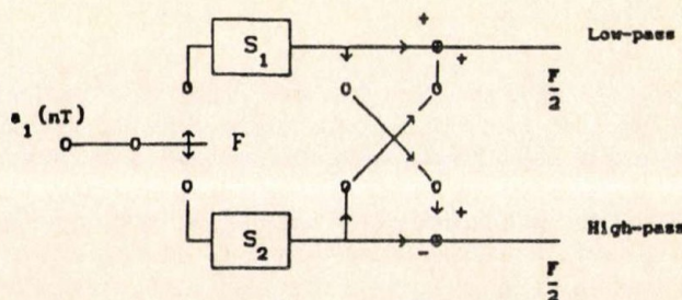
Fig. 2. A bireciprocal structure
