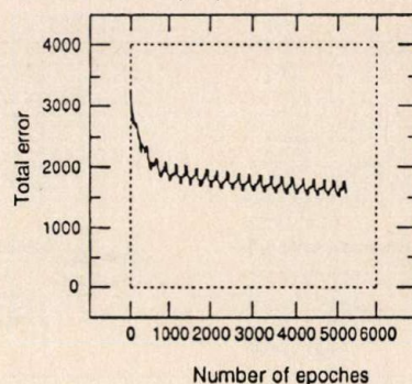
Fig. 6. The total error as a function of the number of epoches during the training of the coarse feature network. The fluctuations are caused by periodically changing the training material between five different training partitions. One epoch in this figure means one presentation of all the patterns in one partition only, and the error is also related to one partition at a time.
