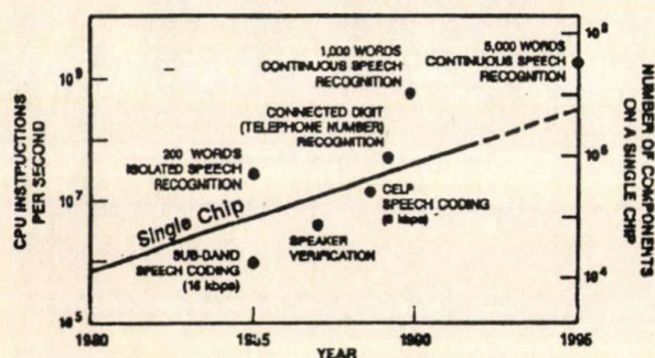
Fig. 1. Computational requirements for selected speech processing algorithms (Points). Processing capability and component density for single-chip digital signal processors as a function of time (Line). J.L. Flanagan, 1991.
