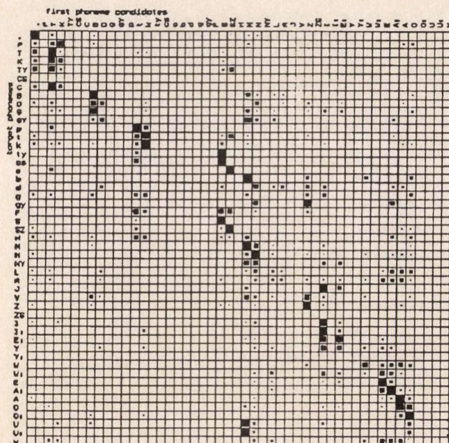
Fig. 13. Phoneme substitutions on the frame level based on the Hungarian MAMO-material. The values are normalized for each row. The area of the black squares is proportional to the number of occurrences in each position.
