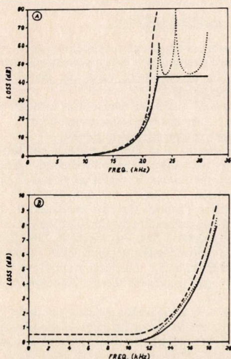
Fig. 4. Loss response of bireciprocal filter construction (with the specification)
