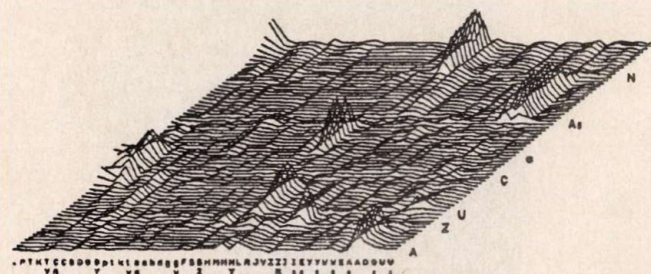
Fig. 9. The output activations of the phone network represented as a surface in a three-dimensional space: time, phoneme, set, and output activations. The manually decided phoneme labels are displayed along the time axis. Each ridge refers to one phoneme.
