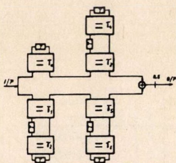
Fig. 6. WD realization of lattice filter construction
