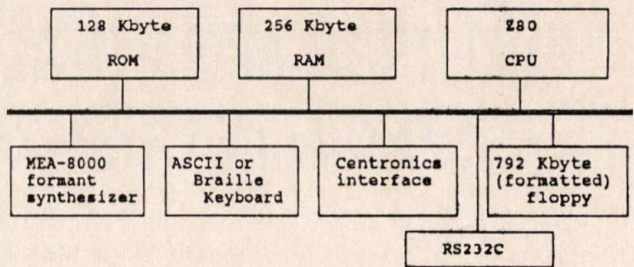
Fig. 6. Configuration of Brailab Plus
