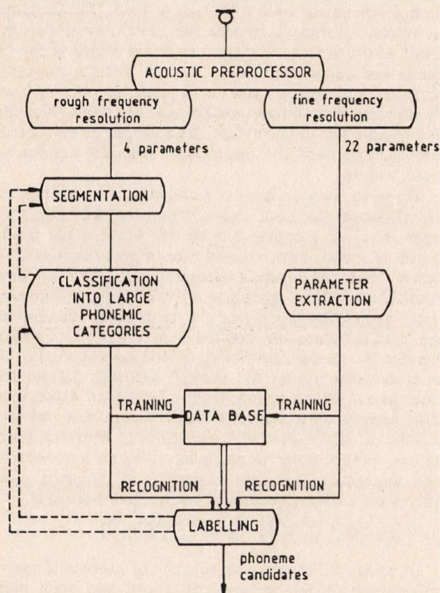
Fig. 2. Continuous speech recognition on acoustic-phonetic level
