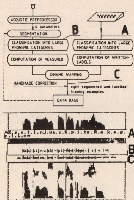
Fig. 8. Automatic training procedure
