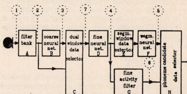
Fig. 2. The elements of the acoustic—phonetic recognition unit. Representations at different points of the system are shown in Fig. 3 and Fig. 4.
