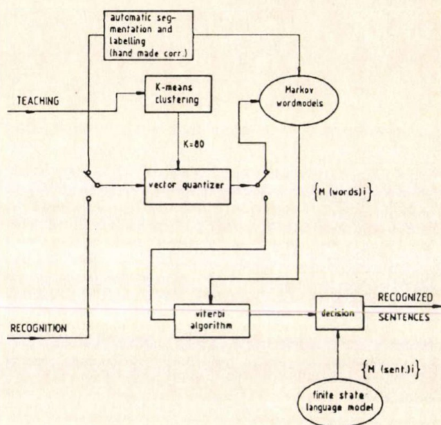
Fig. 10. Connected word recognizer
