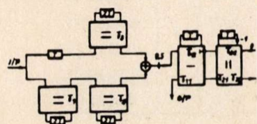
Fig. 9. WD realization of bireciprocal + L,C equalizer filter construction
