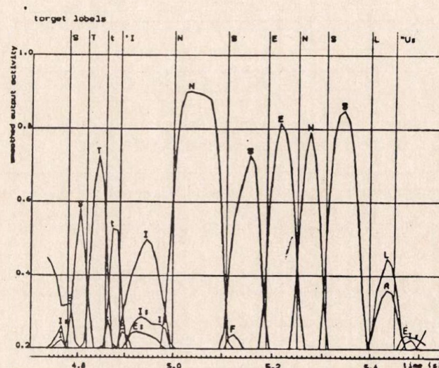
Fig. 14. An example of the smoothed phone net output activations.
