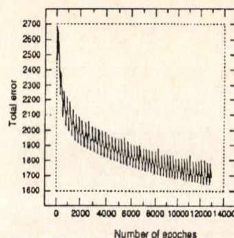
Fig. 8. The total error of the phone net as a function of the number of training epoches for the MAMO material. The fluctuations are caused by periodically changing the training material between five different training partitions. One epoch in this figure means one presentation of all the patterns in one partition only, and the error is also related to one partition at a time.
