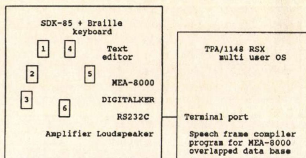
Fig. 1. Development System to Create Data Base for MEA-8000
