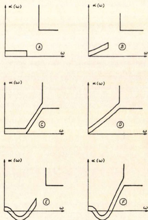
Figure 1. a: Prototype amplitude specification, b-f: arbitrary amplitude specification
