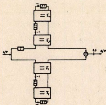
Fig. 7. WD realization of bireciprocal filter construction
