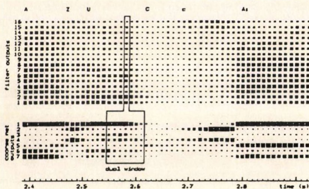
Fig. 4. The dual input window of the phone network. It includes one section of the filter bank output and the coarse phonetic feature parameters in seven frames.
