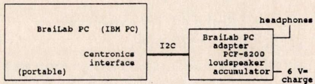
Fig. 7. Configuration of Portable Brailab PC
