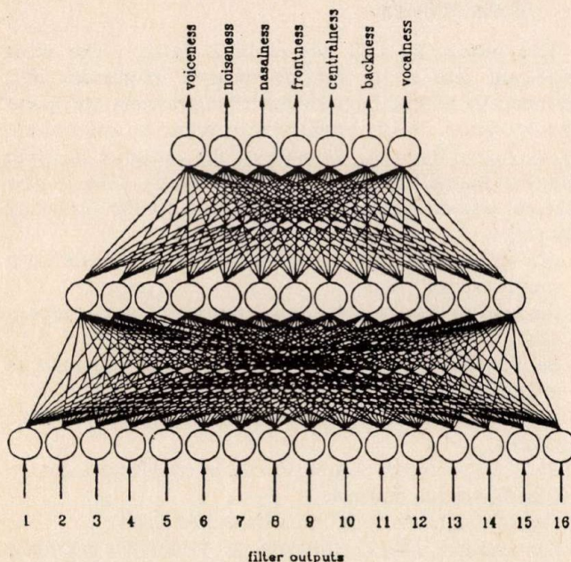
Fig. 5. The structure of the coarse feature network.
