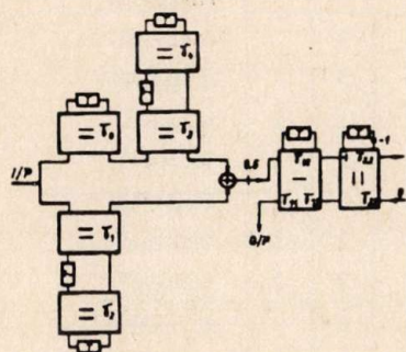
Fig. 8. WD realization of lattice + L,C equalizer filter construction
