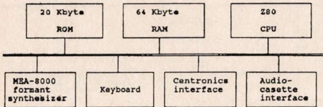
Fig. 5. Configuration of Brailab Basic
