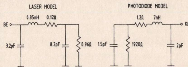
Fig. 9. Electrical models used for laser diode and photodiode
