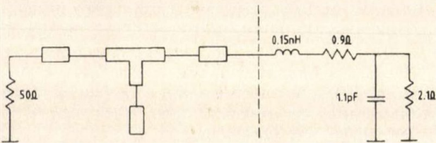
Fig. 3. Single matching stub
