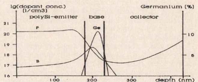
Fig. 4. Impurity profiles obtained by secondary ion mass spectroscopy (SIMS) in polysilicon contacted HBTs.
