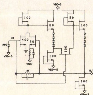
Fig. 4. c) Feed-forward technique proposed in [1] and [17].
