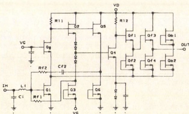
Fig. 4. d) Transimpedance amplifier with three feedback loops in [22].
