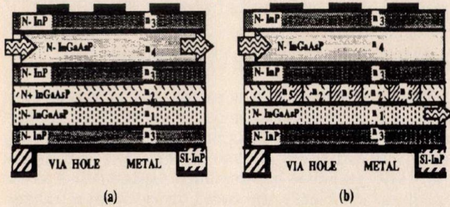
Fig. 3. Optical switch/modulator structure. With no applied electric field, Fig. 3a, light is guided through the upper waveguide. The electric field depletes carriers under the Schottky contacts forming a grating through this grating both waveguides are coupled and light is switched from the upper to the lower waveguide.
