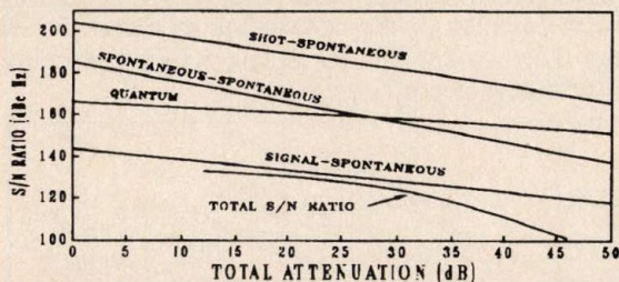
Fig. 4. Modelled S/N ratio of the link using one semiconductor laser amplifier. The various noise contributions due to the laser amplifier can be seen.
