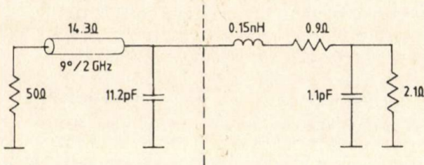
Fig. 2. One section matching impedance
