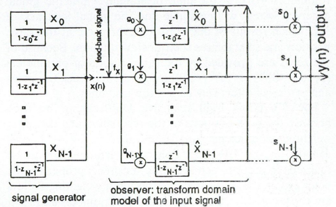
Fig. 6. Concept and structure of resonator based digital filter
