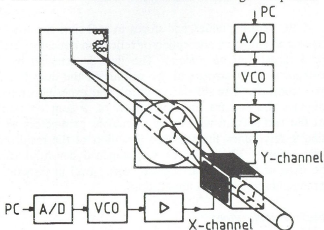
Fig. 2. XY-deflector system
