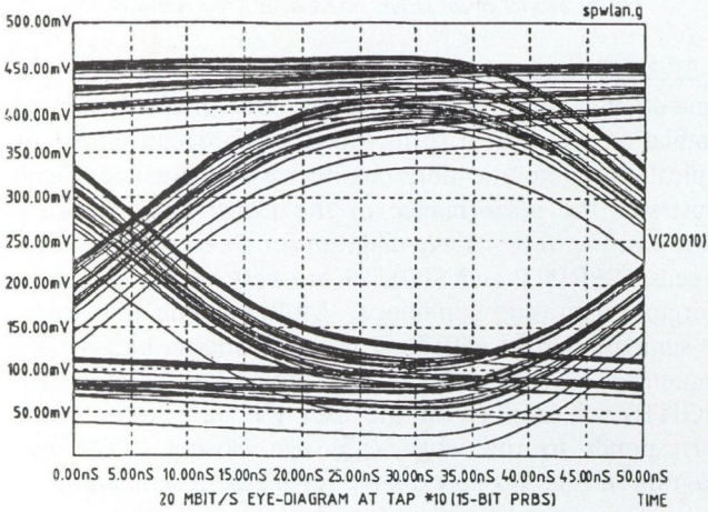
Fig. 9. Performance of the LAN for PRBS input, in the form of eye diagram.
