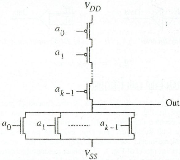
Fig. 4. Static row decoder circuit
