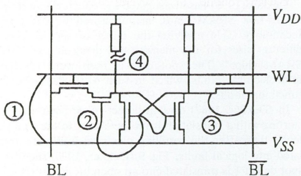
Fig. 10. Examples of defects in the electrical circuit
