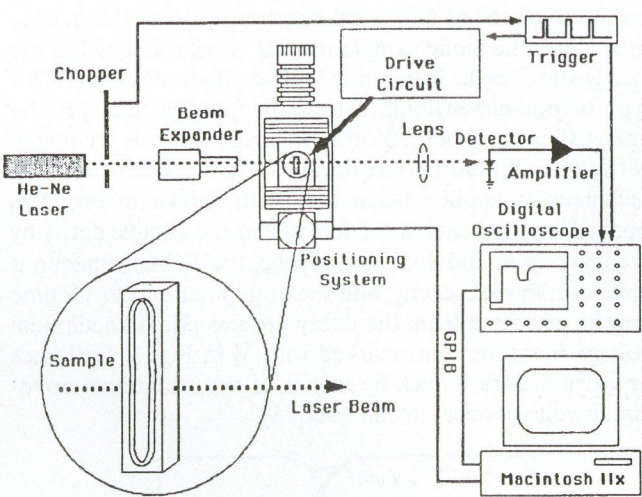
Fig. 2. Schematic view of the FCA measurement system
