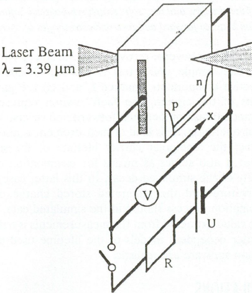
Fig. 3. Schematic view of the circuit used for FCA measurements of P-I-N diodes
