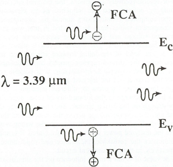
Fig. 1. Illustration of the physical principle of free-carrier absorption (FCA) measurements
