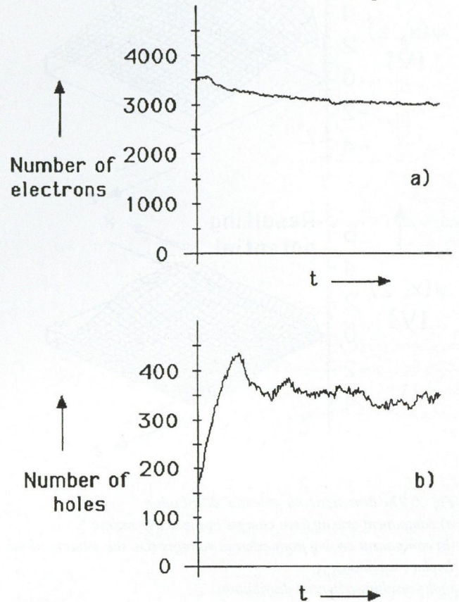
Fig. 11. The number of carriers vs. time a) electrons; b) holes.
