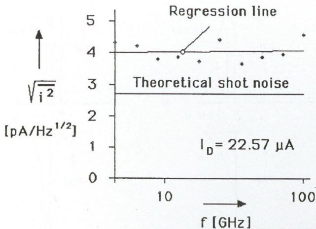
Fig. 14. Shot noise of the drain current
