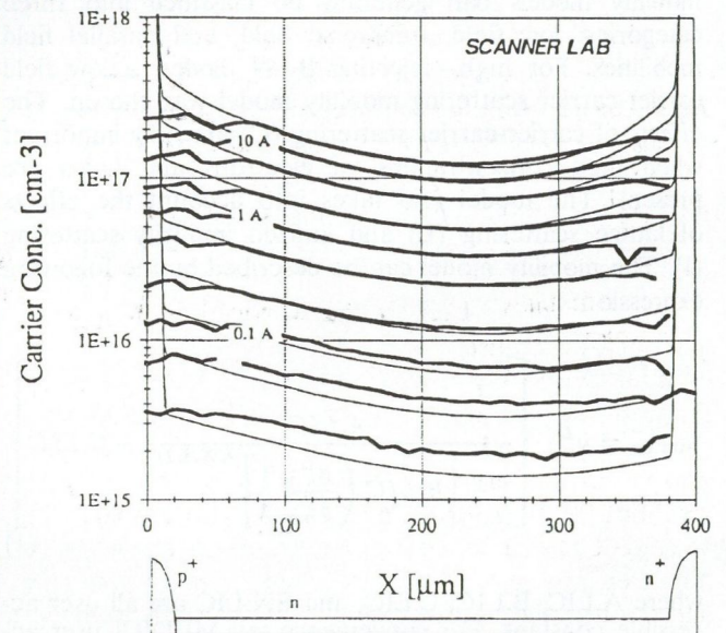
Fig. 8. Comparison between measured (thick lines) and simulated (thin lines) one-dimensional excess carrier distributions in the n -base of a P-I-N diode for different injection levels. The diode forward current ranges from 20 A (topmost two curves) to 20 mA (lowest two curves).
