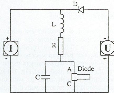
Fig. 5. The outer circuit used in simulation. Only one half of the sample structure is simulated, due to symmetry.
