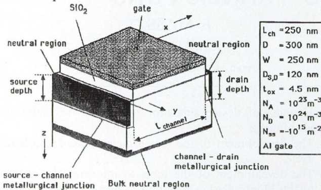
Fig. 1. The simulated structure. The active region is simulated by molecular dynamics Monte Carlo method. The active region is the channel region, and limited volumes of the source, drain and bulk neutral regions. Outside the active region classical approximations are used.
