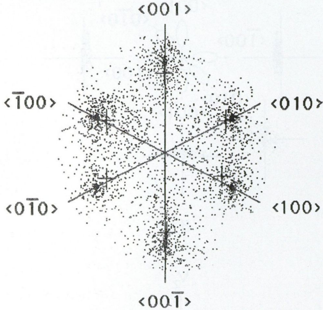
Fig. 9. Axonometric view of the k -vector distribution of electrons corresponding to various ellipsoids in the k -space
