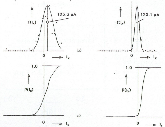
Fig. 13. The conduction current along the x -axis
