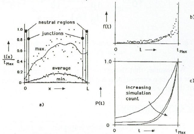
Fig. 12. The time spent in the structure at various stages of the simulation (electrons)
