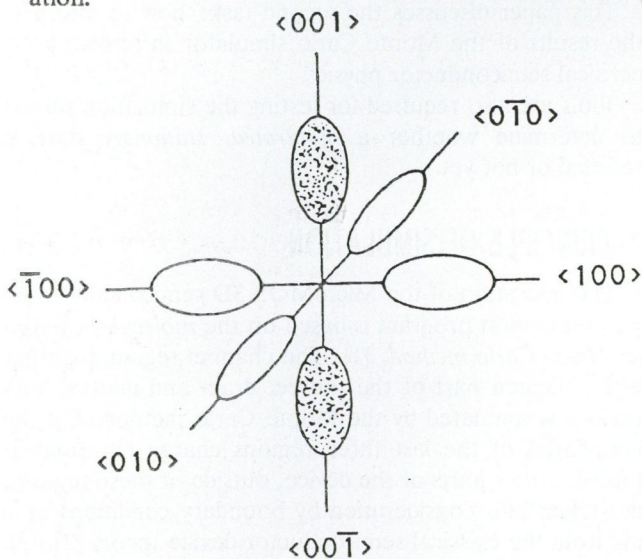
Fig. 2. Constant energy surfaces of electrons in the k -space
