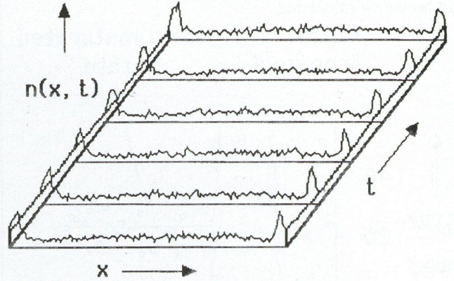
Fig. 4. The instantaneous concentration along the x -axis vs. time
