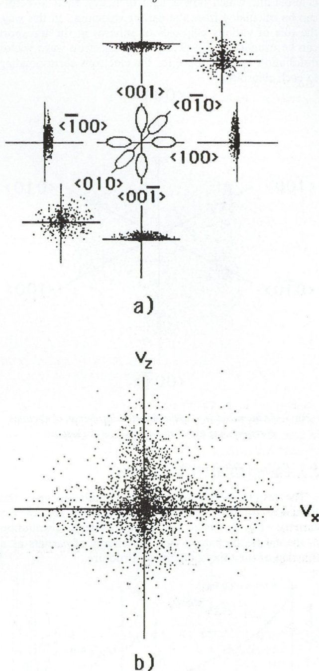
Fig. 8. The velocity distribution of electrons in the velocity space (as seen from the direction of the y -axis) a) the components corresponding to various ellipsoids; b) the resulting velocity distribution.
