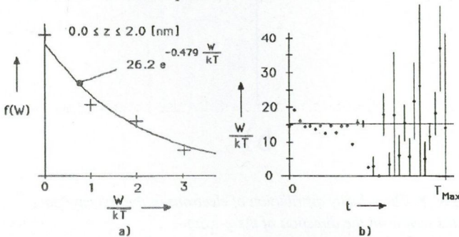
Fig. 10. The energy distribution of electrons a) the distribution function near the Si-SiO 2 interface; b) the energy distribution vs. the time spent in the structure. The vertical bars show the influence of \pm 1 electron.
