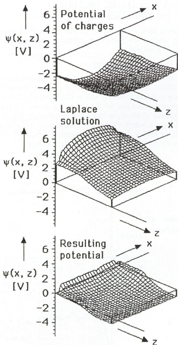
Fig. 7. The instantaneous potential distribution a) component arising from charges in the active region; b) component arising from external voltages (i.e. the solution of the Laplace equation); c) the resulting potential distribution.
