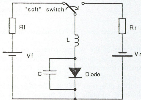
Fig. 4. The circuitry used for reverse-recovery measurements of P-I-N diodes. The reactive components (L and C) represent parasitic effects of the circuitry, and the "soft" switch symbolizes a soft/ramped transition between forward and reverse biased modes of operation.
