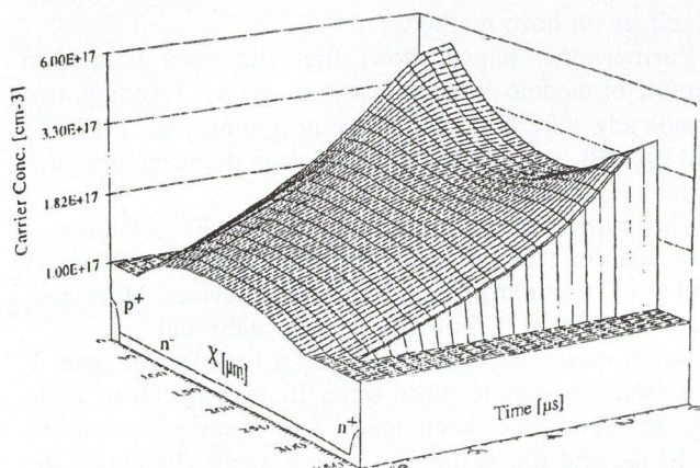
Fig. 9. Example of measured one-dimensional carrier distribution in the n -base of a P-I-N diode. The anode-to cathode carrier distribution is decaying from steady-state (at t = 0 ) to the open-circuit distribution after 8.8 \mu\text{s} . The forward current level is 20 \text{ A} in this case.
