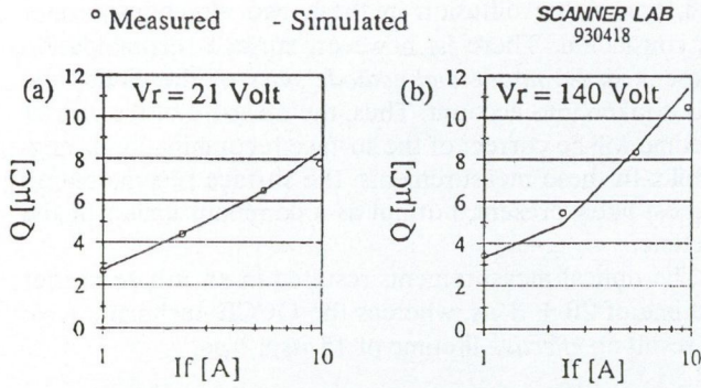
Fig. 11. Comparison between measured and simulated reverse-recovered charge for a P-I-N diode at four different forward current levels and at two different reverse voltages. The current slopes after turn-off are about 16 \text{ A}/\mu\text{s} in (a) and approximately 100 \text{ A}/\mu\text{s} in (b). In this simulation the n -base (bulk) lifetime used was 17 \mu\text{s} .
