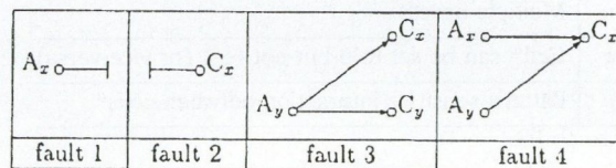
Fig. 8. Address decoder faults
