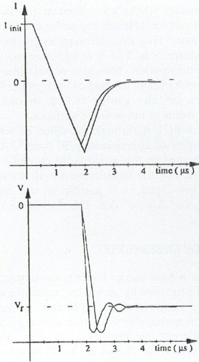
Fig. 6. a) Illustration of how the peak of the i(t) curve moves down if C decreases. b) Illustration of how the peak of the v(t) curve moves sideways if C decreases.
