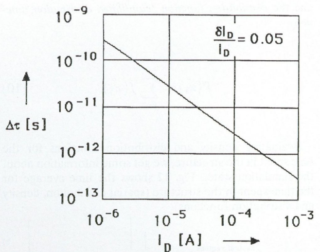
Fig. 15. The time averaging interval vs. drain current (for 5% drain current fluctuation)
