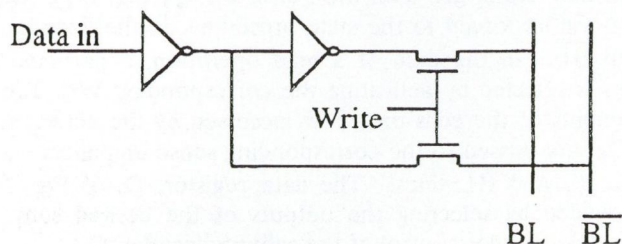
Fig. 5. RAM write circuit
