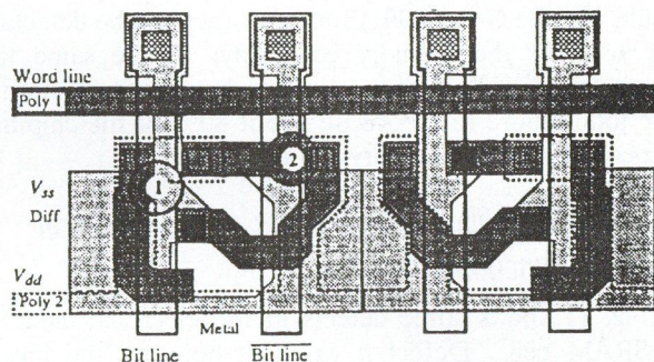
Fig. 9. Relationship spot defects — electrical faults
