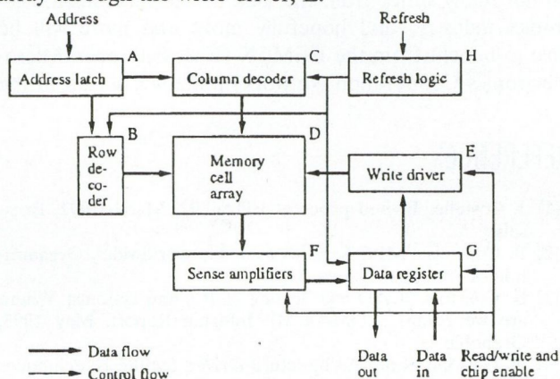
Fig. 1. Functional model (data path and control) of a DRAM chip
