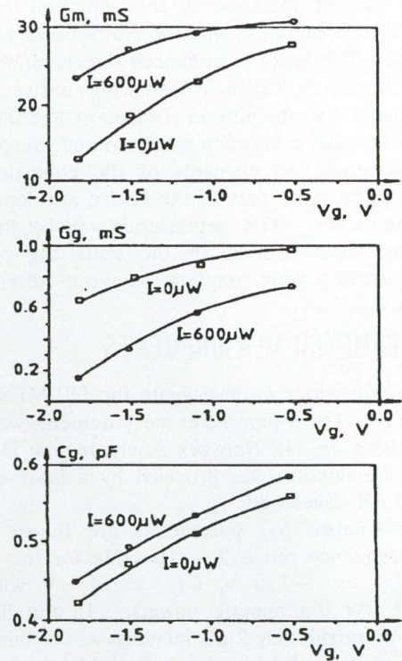
Fig. 6. Admittances vs. gate voltage
