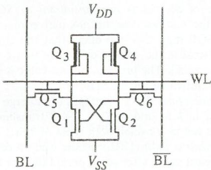
Fig. 3. Six-device SRAM cell structure
