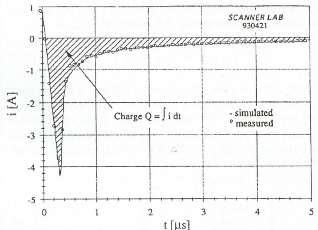
Fig. 10. Comparison between measured and simulated current of a ramped reverse-recovery process. The recovered charge Q is shown as the shaded area. In this particular case, the forward current is 1.0 \text{ A} , the reverse voltage is 21 \text{ V} , and the current slope is 16 \text{ A}/\mu\text{s} .
