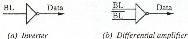
Fig. 6. Simple read circuits
