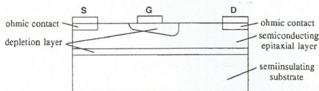
Fig. 1. The structure of the MESFET device
