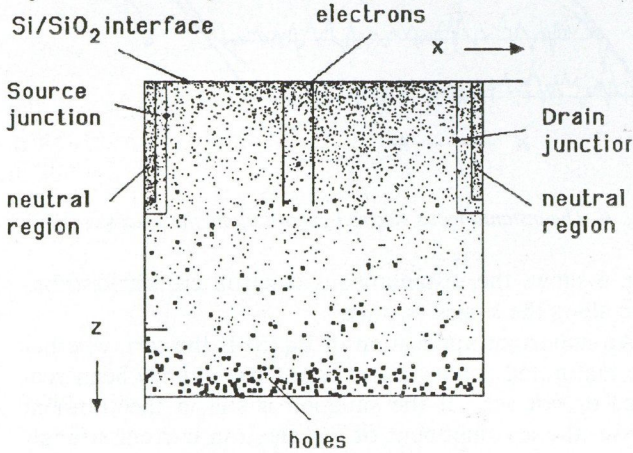
Fig. 3. Electron and hole distribution in the simulated structure
