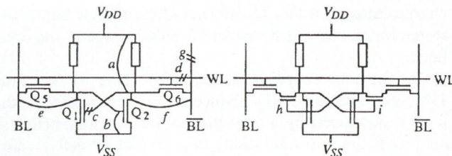
Fig. 11. Defects in a SRAM cell
