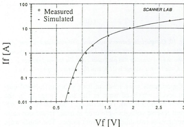
Fig. 12. I-V characteristics of a P-I-N diode. The simulated data (line) are compared with measured data (points).
