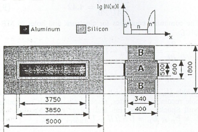
Fig. 7. Cross-sections of the sample diode. All dimensions are in \mu\text{m} .
