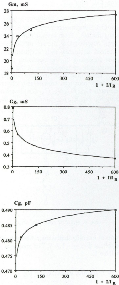
Fig. 5. Admittances vs. optical power
