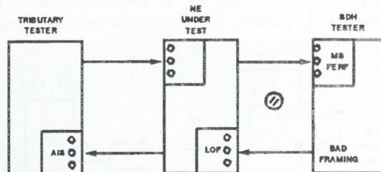
Fig. 15. Alarm testing
