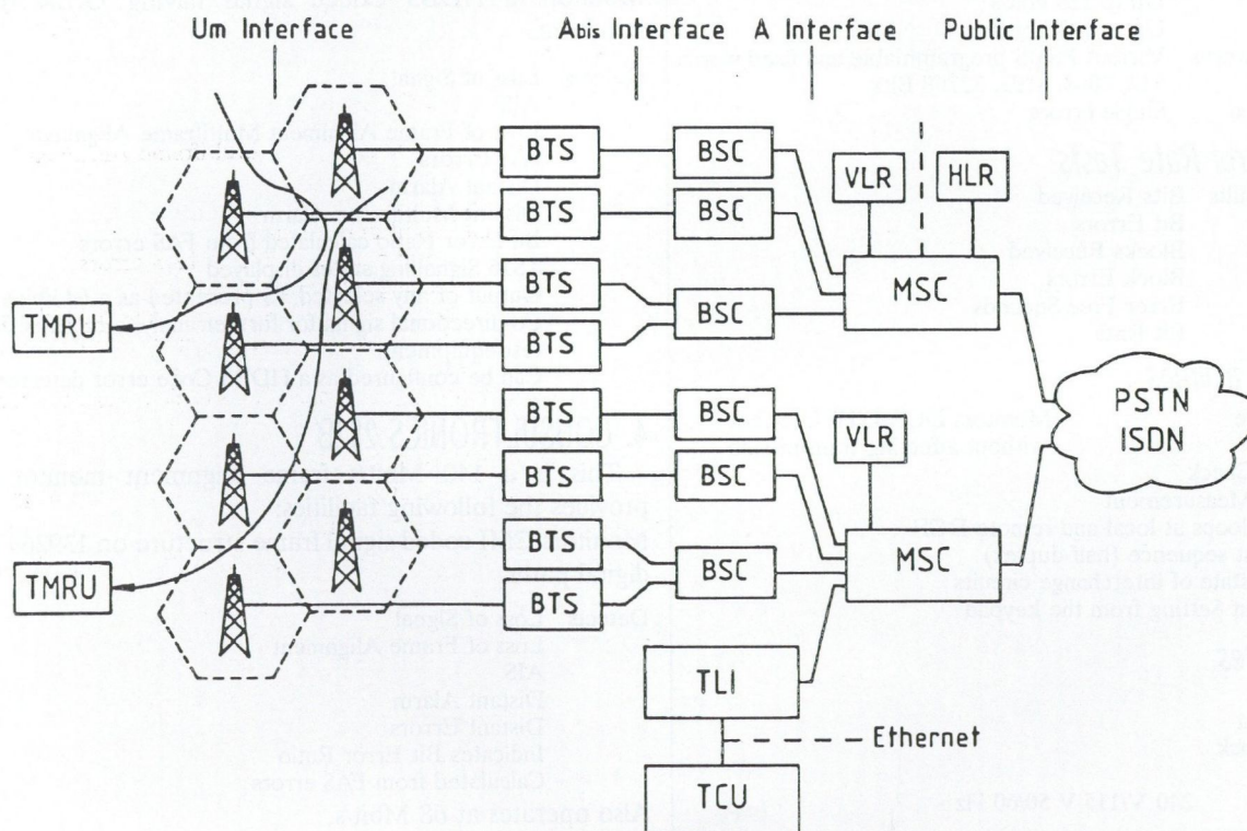
Fig. 1. GSM network elements
