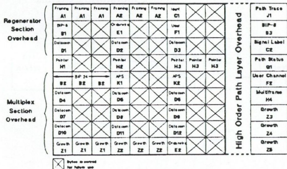
Fig. 6. STM-1 overhead bytes
