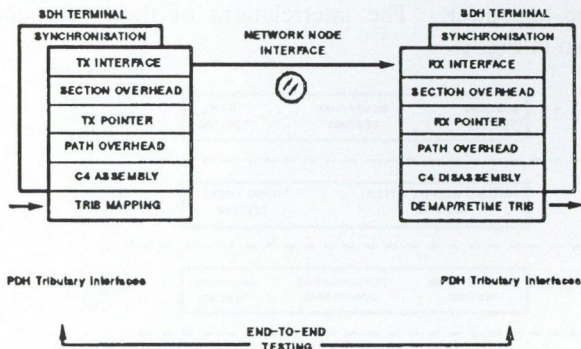
Fig. 3. SDH test environment
