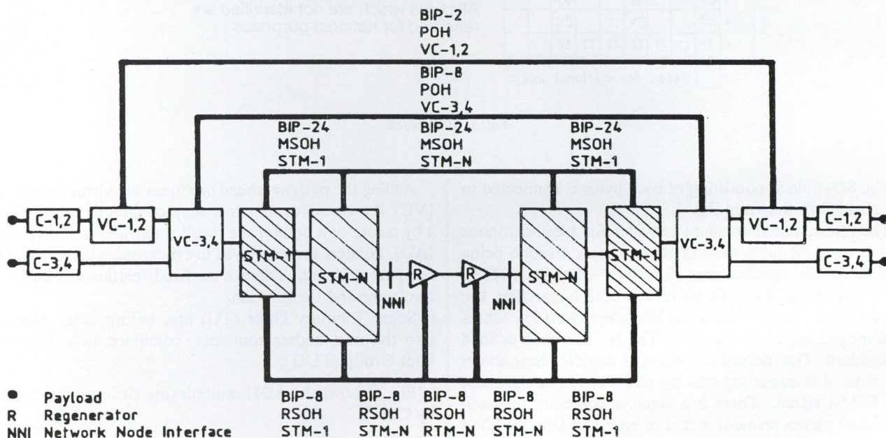
Fig. 7. Supervising sections in SDH systems
