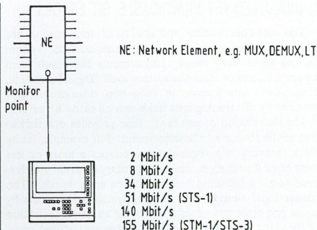
Fig. 2. In-service-monitoring of framed signals
