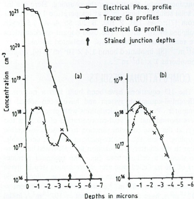
Fig. 1. Experimental profiles from [5]. (a): 15 min/1100°C Ga diffusion followed by 3.5 min/1050°C P diffusion; (b): the Ga diffusion only
