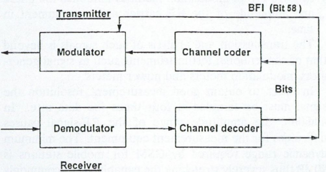
Fig. 6. Indication of faulty frames in GSM Mobile Station
