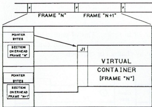
Fig. 5. Link between section overhead and VC
