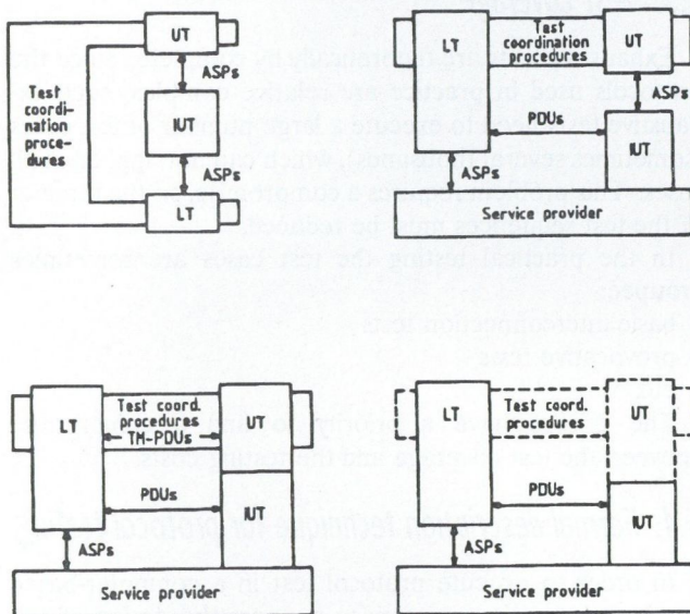
Fig. 3. Abstract test methods
