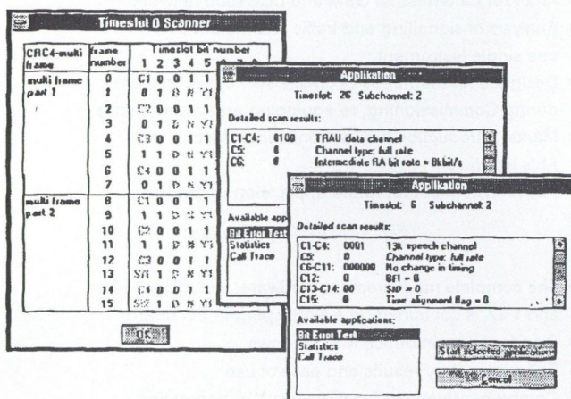
Fig. 3. SCANNER application a) determining the content of a 2 Mbit/s frame b) detailed analysis of traffic channels
