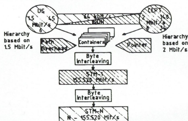
Fig. 2. Multiplex transmission principle
