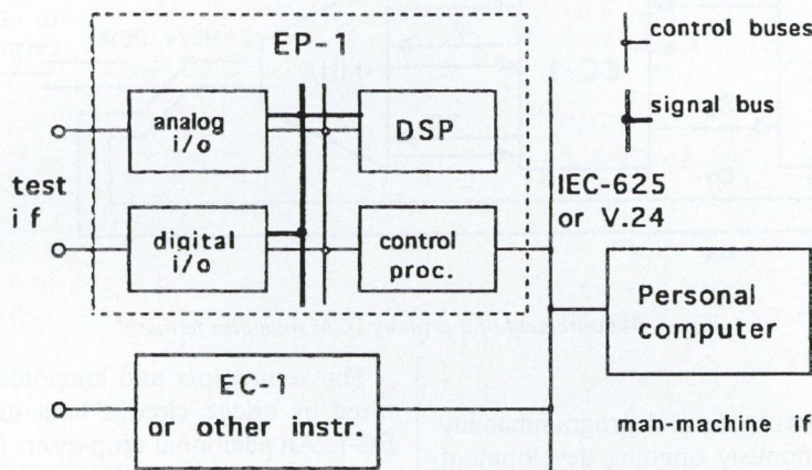
Fig. 1. The three processor architecture of EP-1
