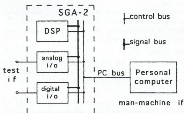
Fig. 2. The two processor architecture of SGA-2
