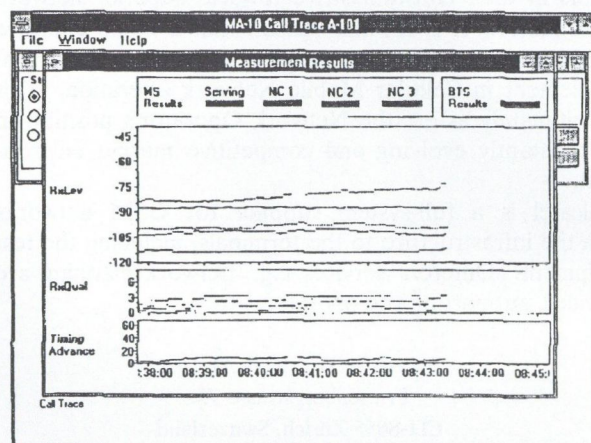
Fig. 4. CALL TRACE application a) listing connections from set-up to clear-down b) graphic representation of measurement results
