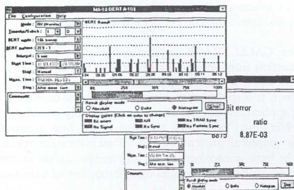
Fig. 5. BERT application, numerical or graphic representations
