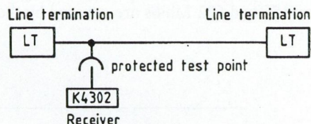
Fig. 9. In service monitoring
