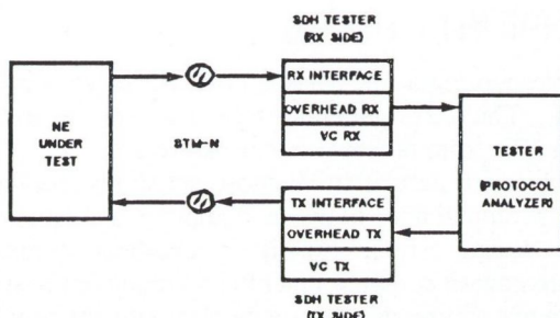
Fig. 21. Embedded communications channel testing
