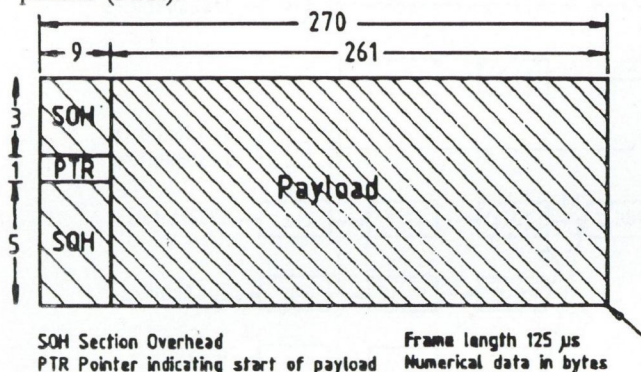
Fig. 4. STM-1 frame
