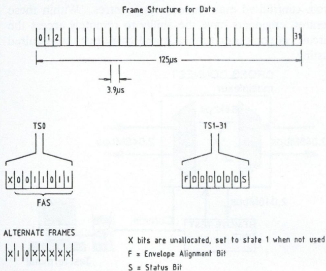
Fig. 1. Frame structure for 2.048 Mbit/s data signal
