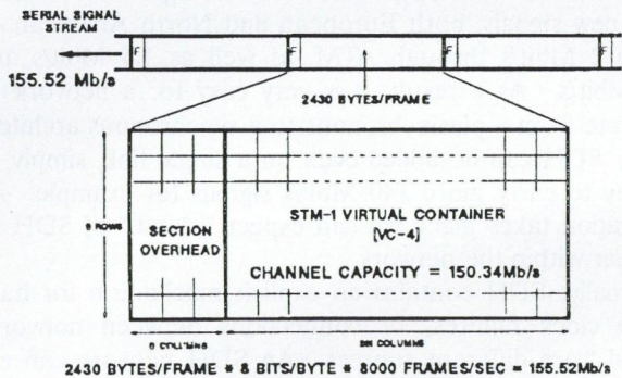
Fig. 4. STM-1 frame structure
