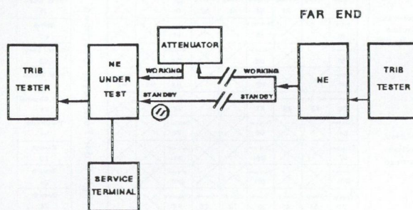
Fig. 10. Protection testing
