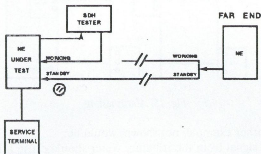
Fig. 11. Protection testing with an SDH tester
