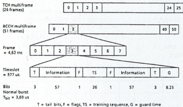
Fig. 3. Structure of time-slots and frames in GSM
