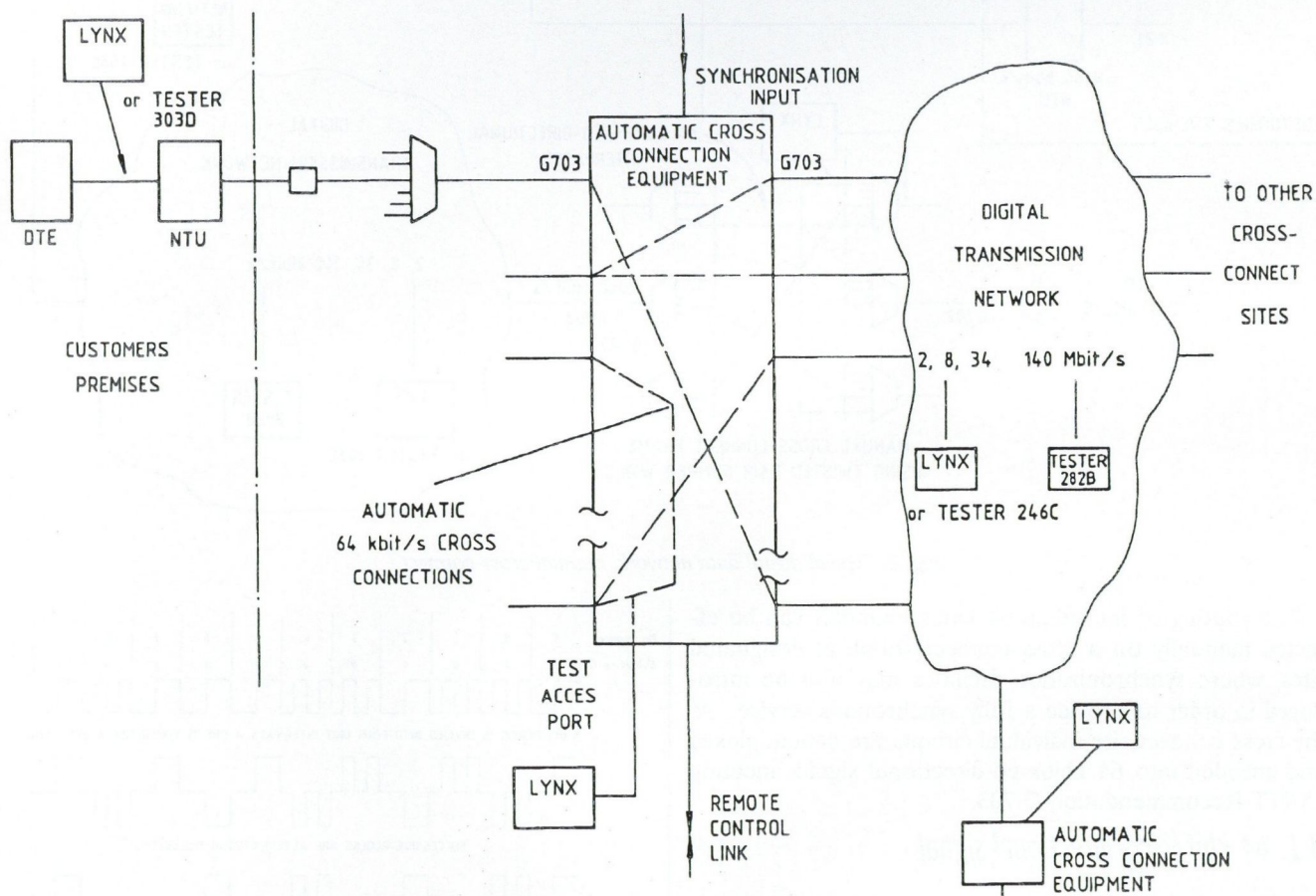
Fig. 4. Typical digital data network, automatic cross-connect
