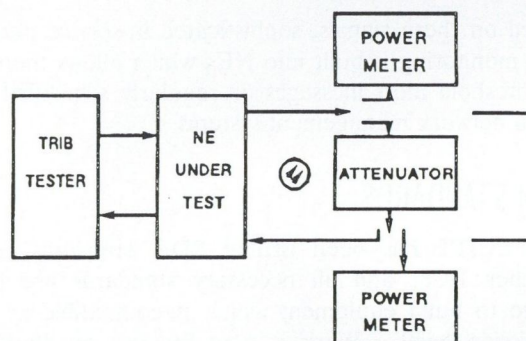
Fig. 8. Optical output and Rx sensitivity testing
