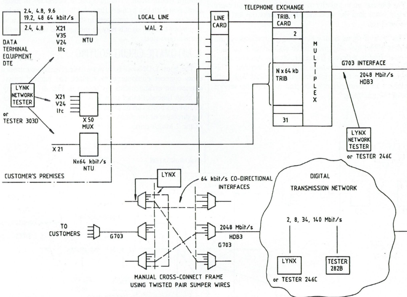
Fig. 2. Typical digital data network, manual cross-connect
