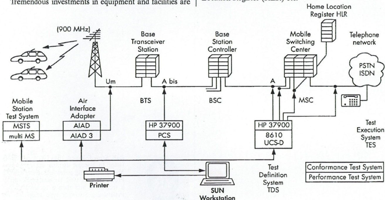
Fig. 1. GSM network elements and test points
