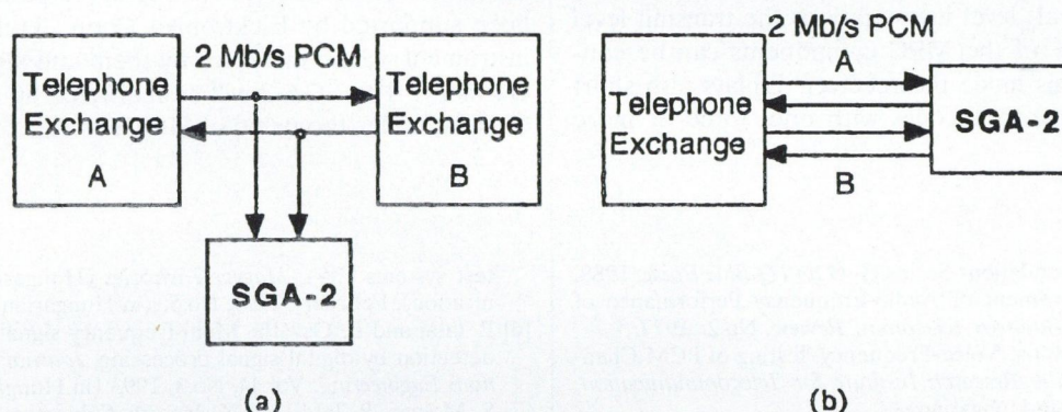
Fig. 4. Testing configurations with SGA-2. Passive monitoring (a) and active emulation (b)
