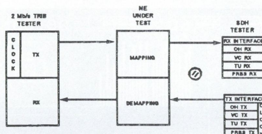
Fig. 16. Tributary continuity stress testing
