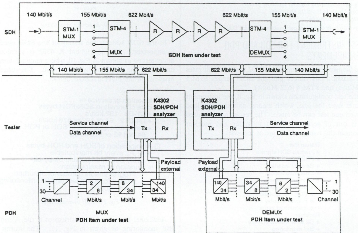
Fig. 13. Typical applications of K 4302 SDH/PDH analyzer: route measurements.
