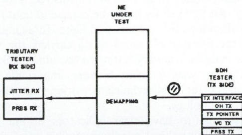
Fig. 17. Tributary output jitter testing
