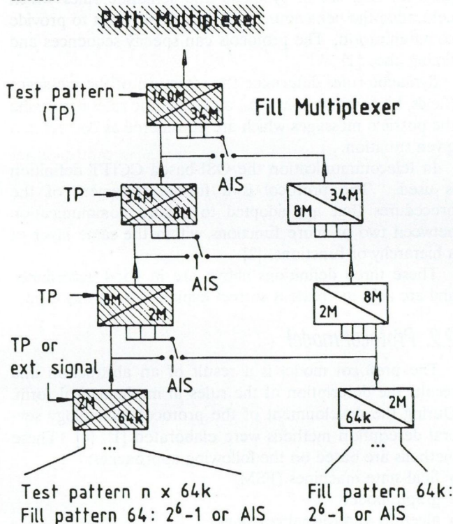
Fig. 6. Option Frame Generator/Analyzer with Multiplex Chain
