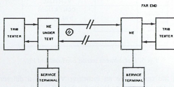
Fig. 9. Low-speed end-to-end error testing
