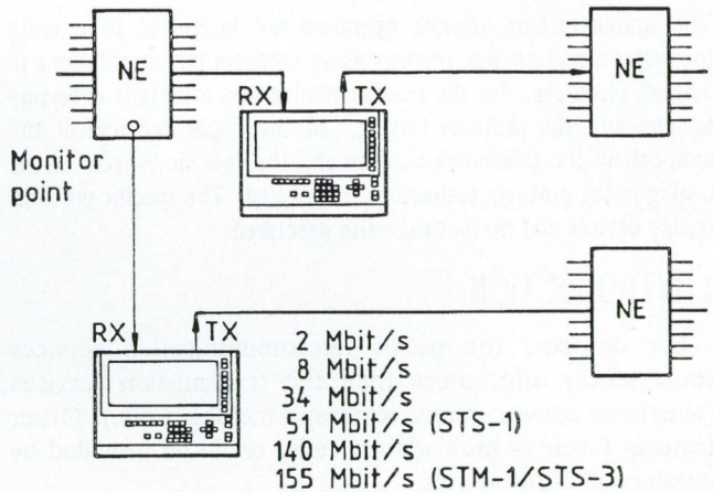
Fig. 7. Operational mode "loop-through"
