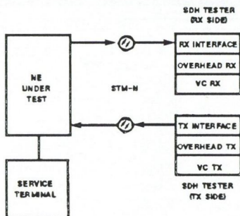
Fig. 22. Performance monitoring testing
