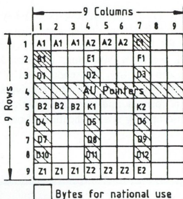
Fig. 4. STM-1 frame
