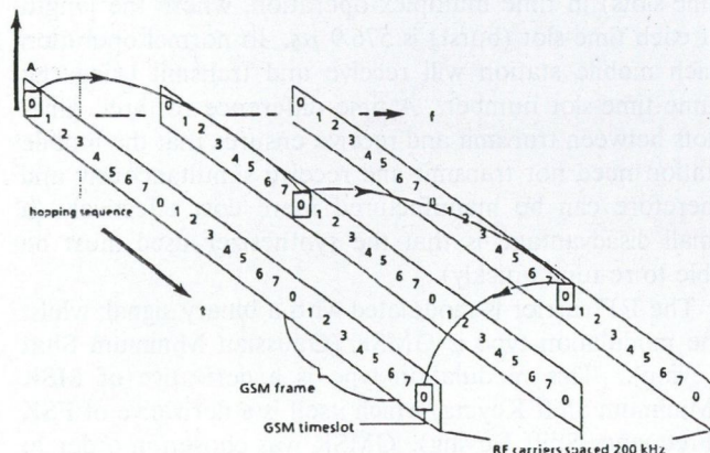
Fig. 4. Time and frequency multiplex on RF-path
