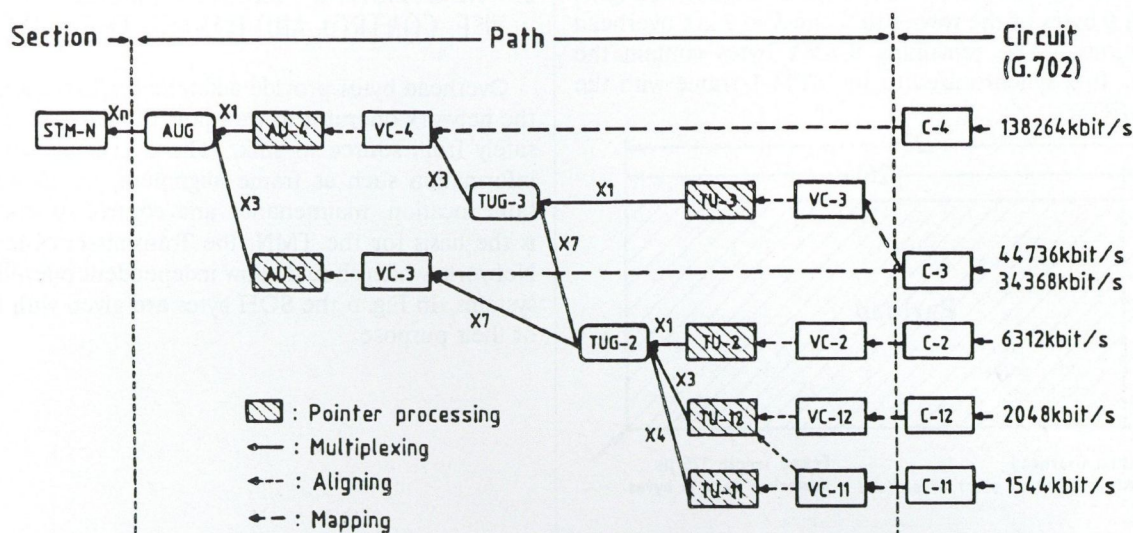
Fig. 6. SDH multiplexing structure
