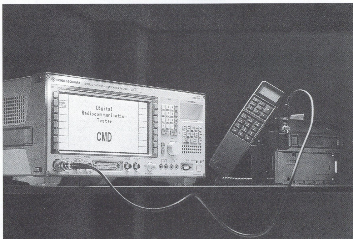
Fig. 1. GSM mobile telephone testing with Digital Radiocommunication Tester CMD
