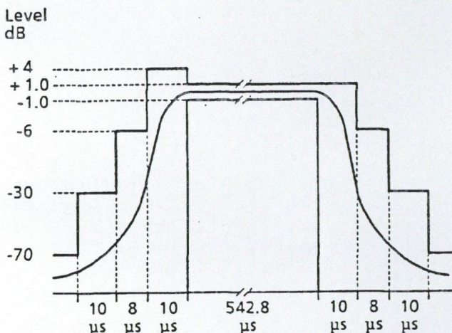
Fig. 5. GSM mobile power ramping (from GSM recommendation 11.10)
