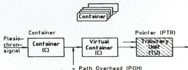
Fig. 3. SDH system blocks. Path overhead (POH)..... Pointer (PTR).....
