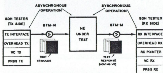
Fig. 18. Timing offset testing
