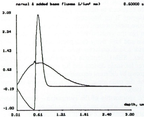
Fig. 2. The ordinary and the additional base fluxes at the start of diffusion. The major peak in the added flux causes the depletion of base impurities, thus the base-dip. See text for more details.
