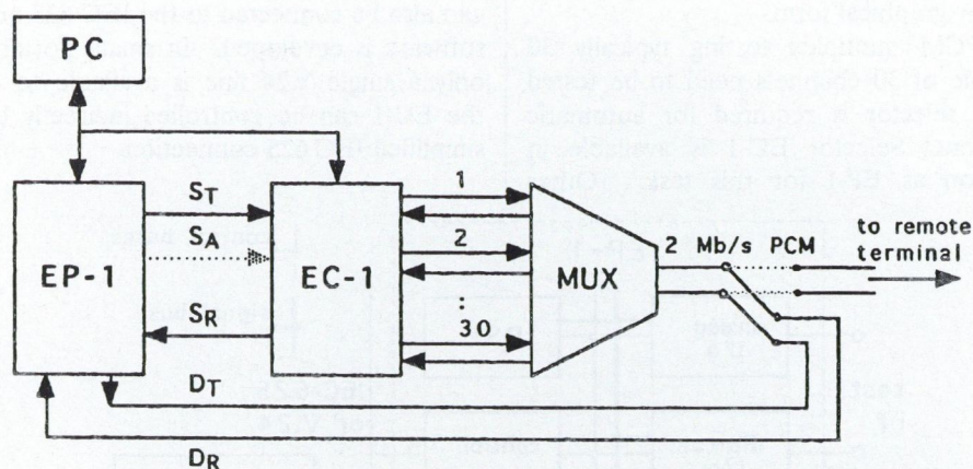
Fig. 3. Measurement of a primary PCM multiplex terminal
