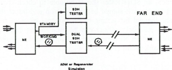
Fig. 23. In-service testing in through mode
