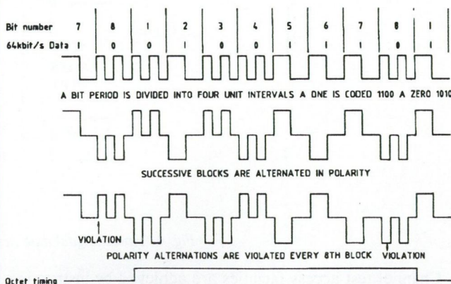
Fig. 3. 64 kbit/s co-directional signal characteristics
