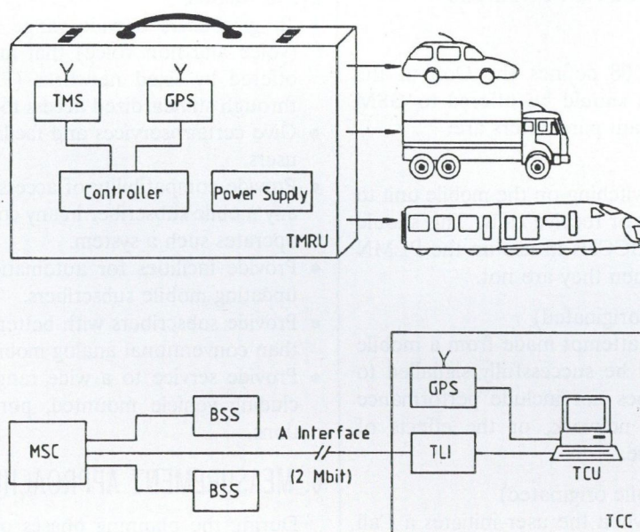
Fig. 2. Network QoS Monitoring
