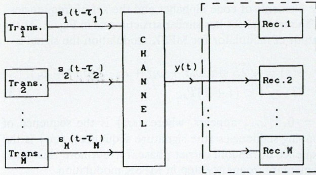
Fig. 2. The multi-access channel
