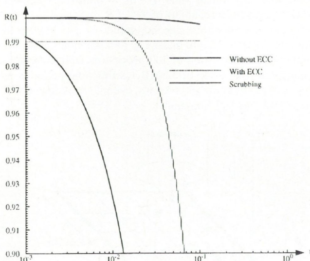
Fig. 2. Reliability of the memory for different protection strategies
