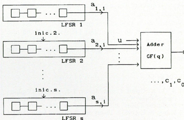
Fig. 5. The structure of the code generator
