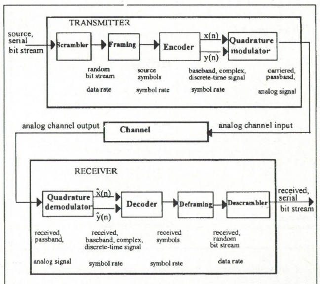
Fig. 1. Data transmission over analog channel
