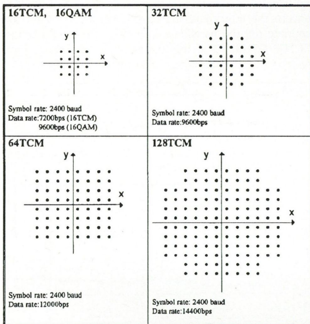
Fig. 2. Baseband discrete-time complex signal constellation diagrams
