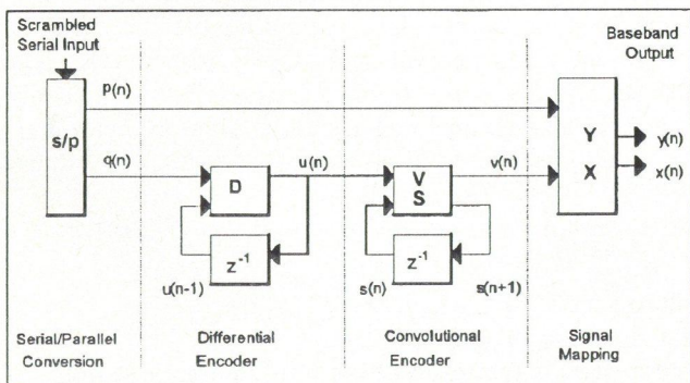
Fig. 5. Block diagram of framing and the trellis encoder
