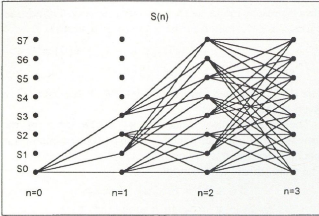
Fig. 6. Trellis diagram of encoder state sequence
