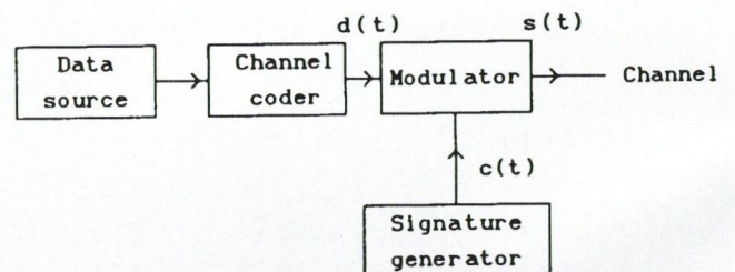
Fig. 1. The transmitter
