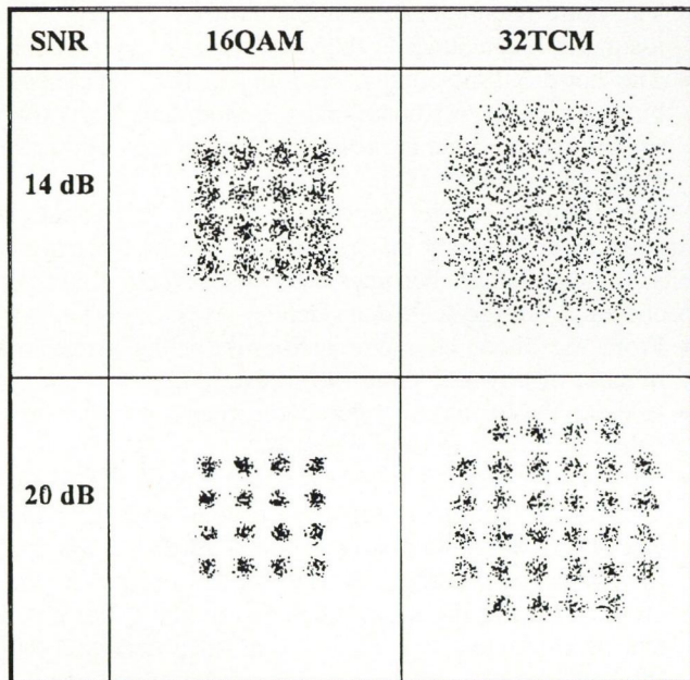
Fig. 11. Noisy signal constellations
