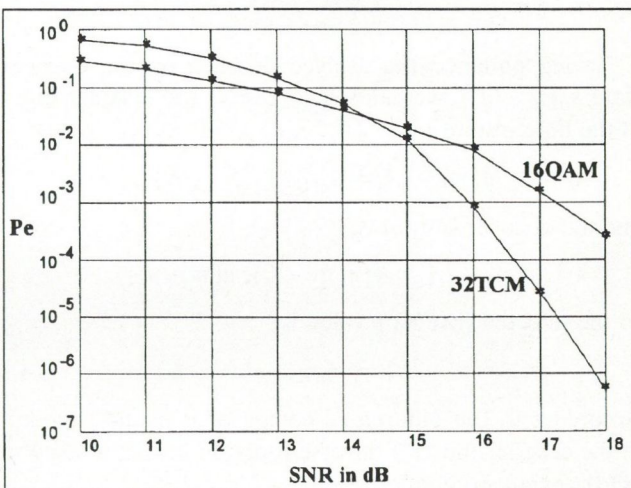
Fig. 10. Probability of error ( P_e ) versus signal to noise ratio (SNR) in case of 16QAM and 32TCM coding techniques
