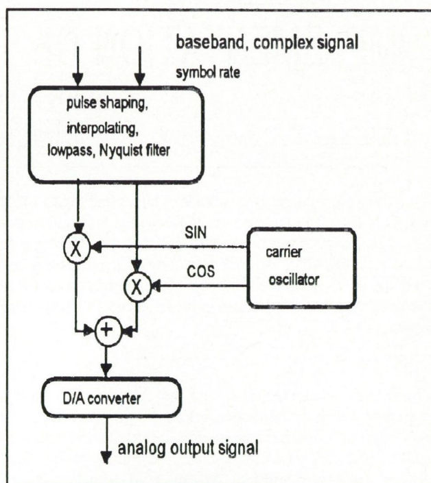
Fig. 3. Quadrature modulator
