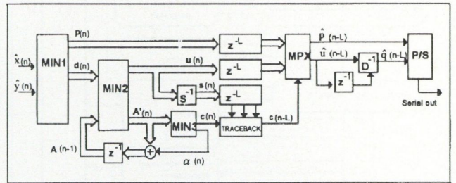
Fig. 7. Block diagram of Viterbi decoder
