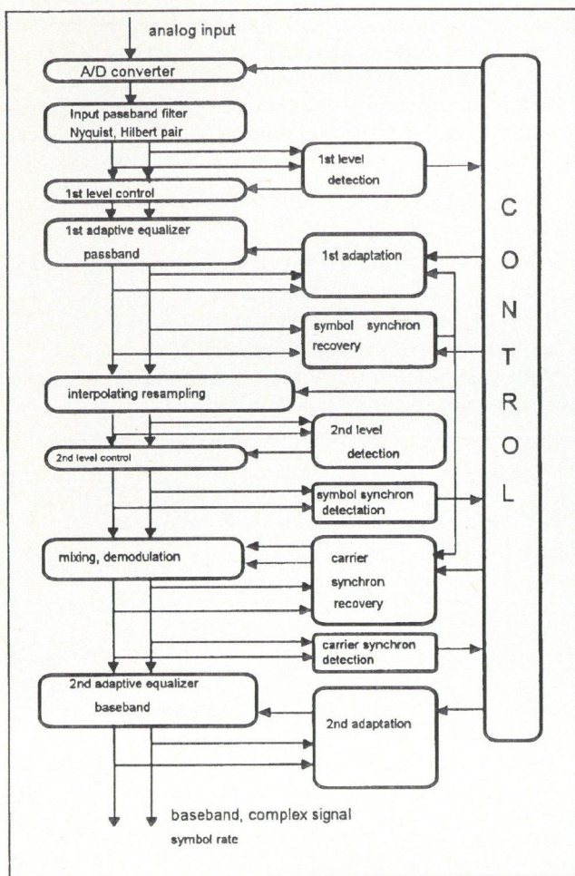
Fig. 4. Quadrature demodulator
