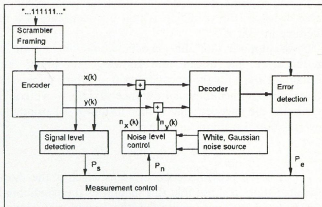
Fig. 9. Block diagram of baseband measurement of the error probability versus SNR
