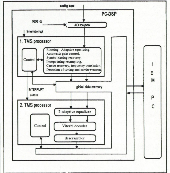
Fig. 8. Implementation of the receiver on PC-DSP board
