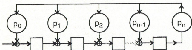
Fig. 3. Polynomial division circuit
