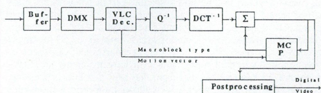
Fig. 4b. Generic block scheme of motion-compensated hybrid decoder
