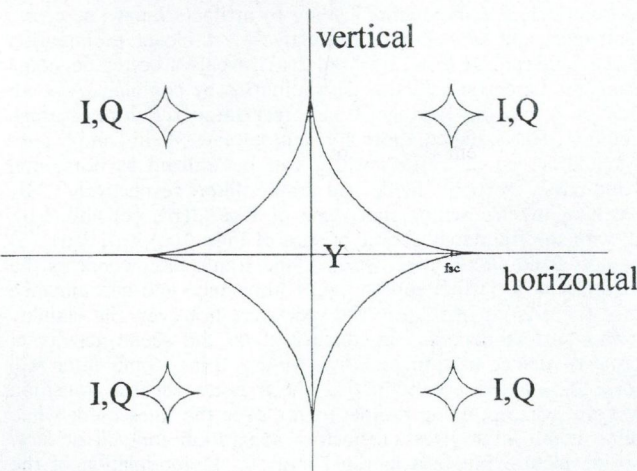
Fig. 1(b). NTSC vertical/horizontal frequency spectrum
