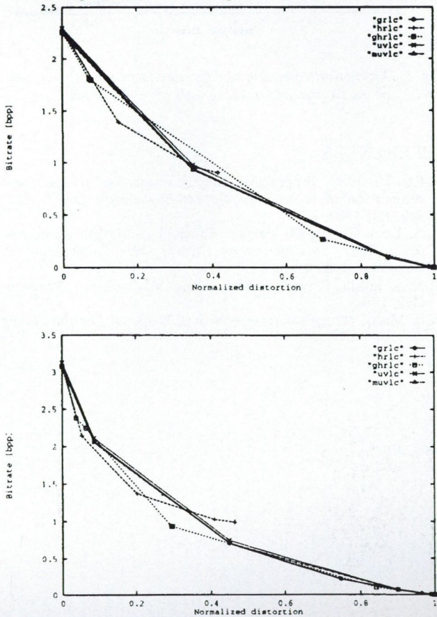
Fig. 2. Distortion-rate function of different coders, for a source with \sigma^2 = 1 (up) and a source with \sigma^2 = 4 (down)
