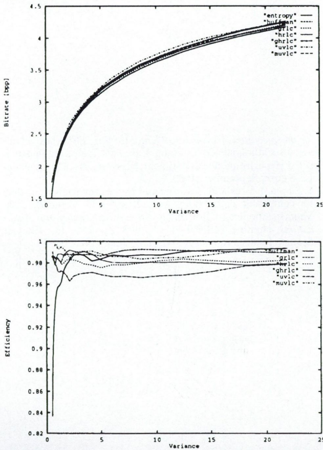
Fig. 1. Bit rate (up) and efficiency (down) for coding Laplacian sources with different variance
