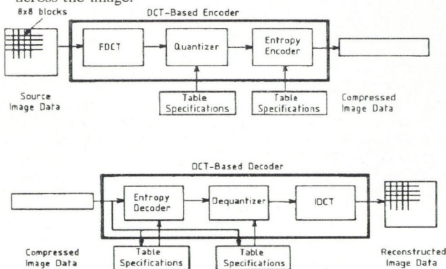
Fig. 7. JPEG compression and decompression
