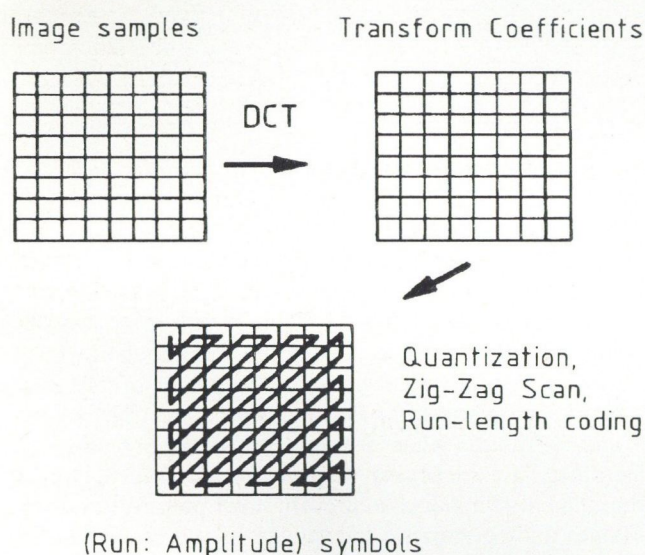
Fig. 1. Transform coding, quantization as well as run-length coding
