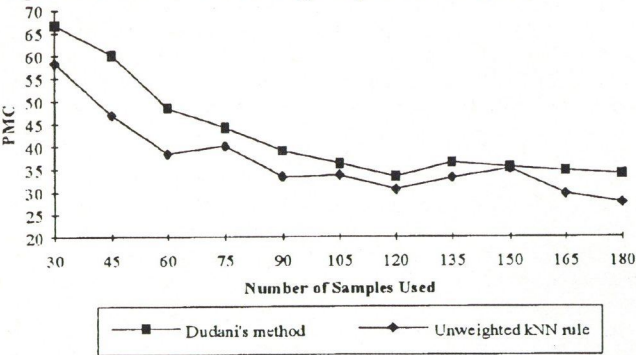
Fig. 5. Comparison of Dudani's method and unweighted kNN rule for 3 neighbours and 5 features
