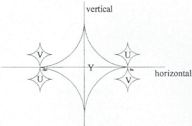
Fig. 2b. PAL vertical/horizontal frequency spectrum
