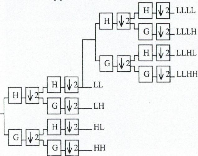
Fig. 1. Example of a filterbank
