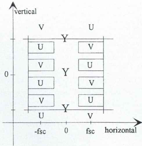
Fig. 2d. PAL vertical/horizontal
