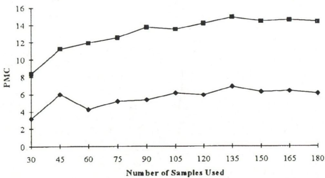
Fig. 1. Upper and lower bounds on the Bayes error for 3 features and \alpha_n = 0.3
