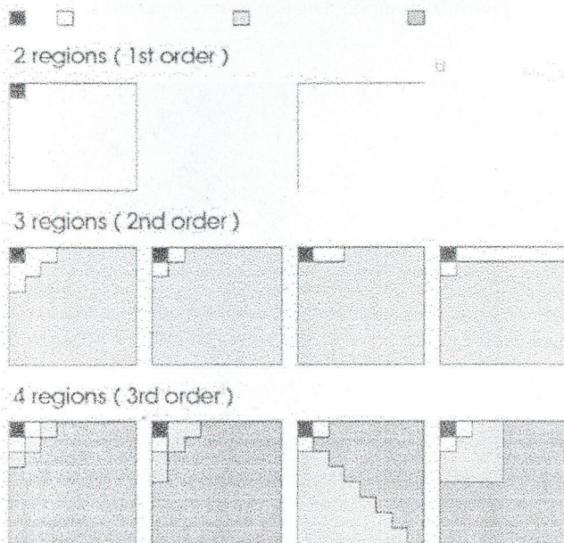
Fig. 8. Examples of different frequency domain partitions for luminance transformations of 1 st , 2 nd , and 3 rd order (block size 8 \times 8 )
