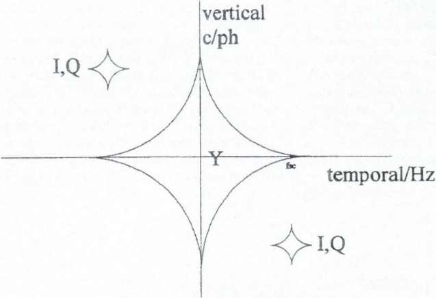
Fig. 1(c). NTSC vertical/temporal frequency spectrum
