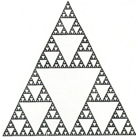
Fig. 1. The Sierpinski gasket that is generated using an IFS consisting of three contractions mappings
