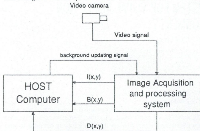
Fig. 2. The image acquisition module
