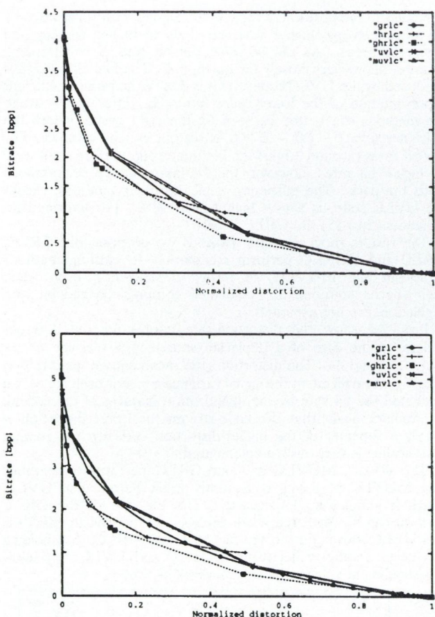
Fig. 3. Distortion-rate function of different coders, for a source with \sigma^2 = 16 (up) and a source with \sigma^2 = 64 (down)
