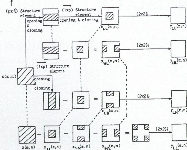
Fig. 2. Block diagram of analysis filter bank for four-subband splitting
