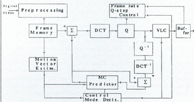
Fig. 4a. Generic block scheme of motion-compensated hybrid encoder
