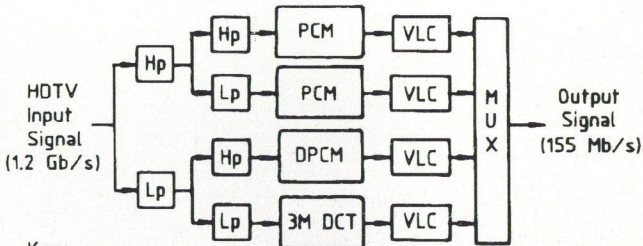
Fig. 3. Subband DPCM for HDTV coding
