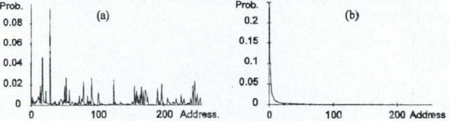
Fig. 2. (a) An example of the addresses' histogram for a memoryless vector quantizer; (b) the same example but for a dynamic-codebook-reordering vector quantizer
