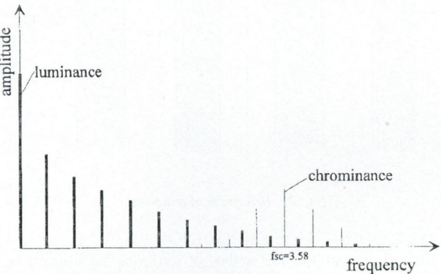
Fig. 1(a). NTSC horizontal frequency spectrum
