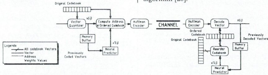
Fig. 3. The global architecture of a dynamic-codebook-reordering vector quantizer
