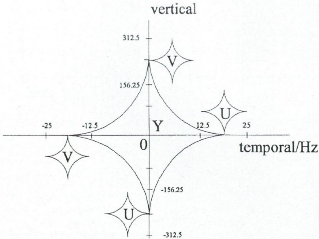
Fig. 2c. PAL vertical/temporal frequency spectrum
