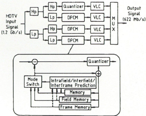
Fig. 3. Subband DPCM for HDTV coding
