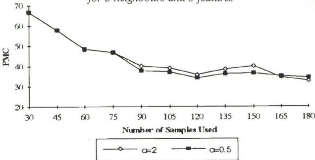
Fig. 6. Change of performance of the \alpha -weighted kNN rule for different values of \alpha
