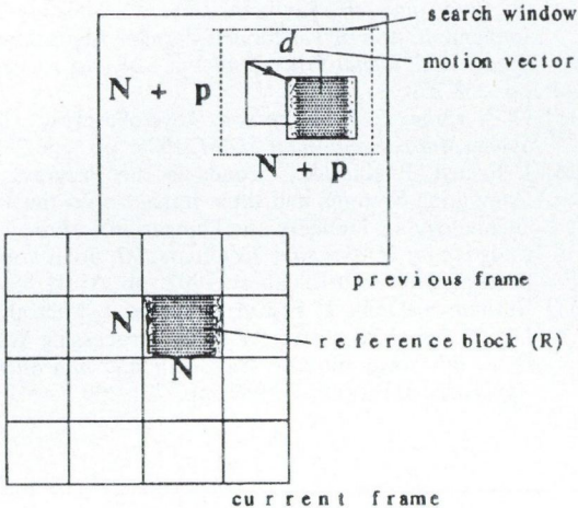
Fig. 5. Motion vector estimation with BMA
