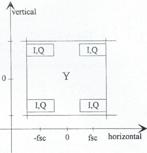
Fig. 1(d). NTSC vertical/horizontal frequency spectrum
