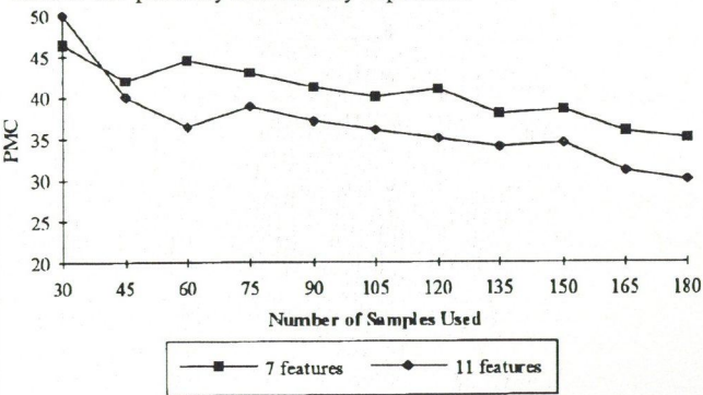
Fig. 7. The performance of the LDF classifier for different number of features
