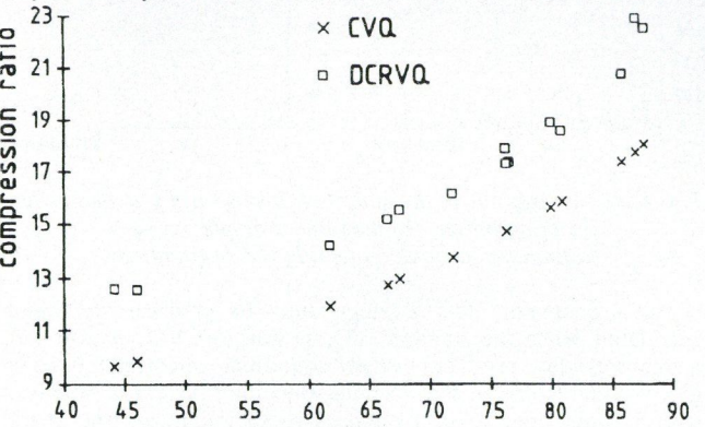
Fig. 4. Performance comparison for neural-predicted CVQ and DCRVQ
