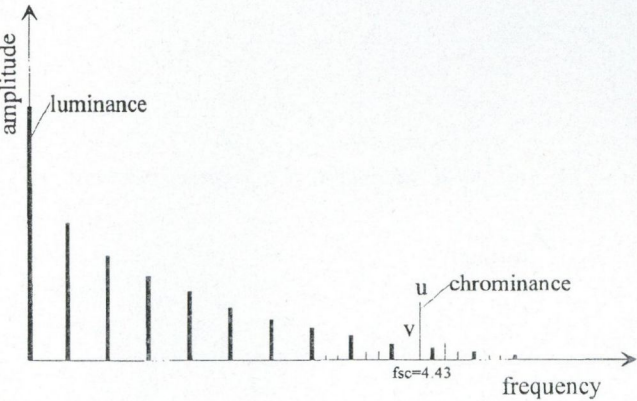
Fig. 2(a). PAL horizontal frequency spectrum
