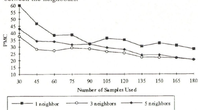
Fig. 8. The performance of the unweighted kNN rule against 5 % impulsive noise for different number of neighbours
