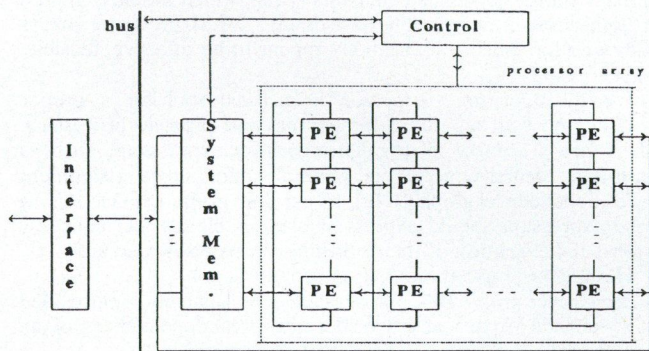
Fig. 3. The overall system of a mesh-connected systolic array
