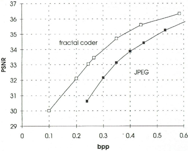
Fig. 10. Coding results of the new fractal coding scheme compared to JPEG. (Image: LENA 512 \times 512 pixels)
