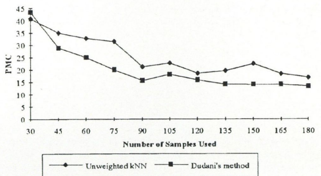
Fig. 4. Comparison of Dudani's method and unweighted kNN rule for 3 neighbours and 11 features
