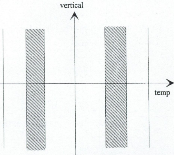
Fig. 1(e). NTSC vertical/temporal frequency spectrum
