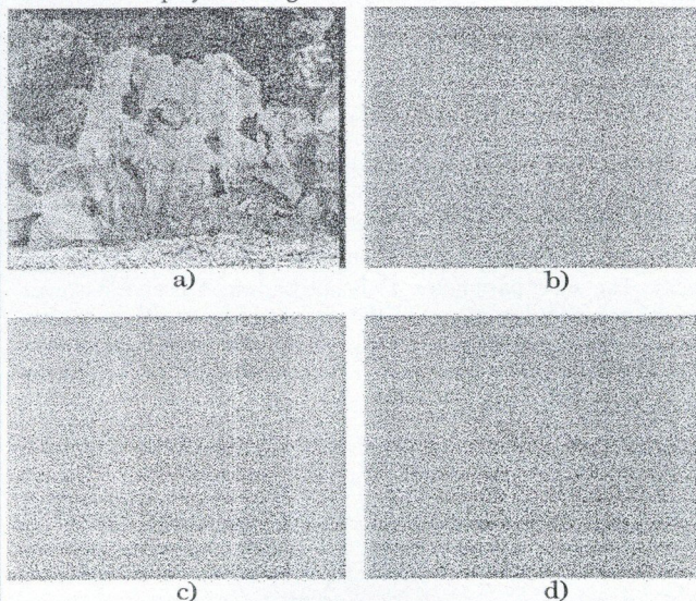
Fig. 4. Images from the "aqua" experiment: (a) Original image (right channel); (b) Error image for DCT coding; (c) Error image for KLT-based coding with no segmentation; (d) Error image for KLT-based coding using variance-based segmentation with 2 segments. Error images are enhanced to show differences.
