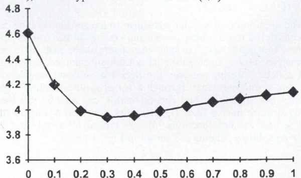
Fig. 4. Mean-square-error of the algorithm as a function of P for frames 31-32 of image sequence "Trevor White"
