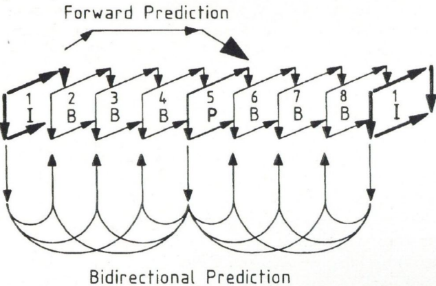
Fig. 2. Relationship between intra, predicted and interpolated pictures
