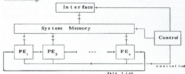
Fig. 2. The ring systolic system architecture
