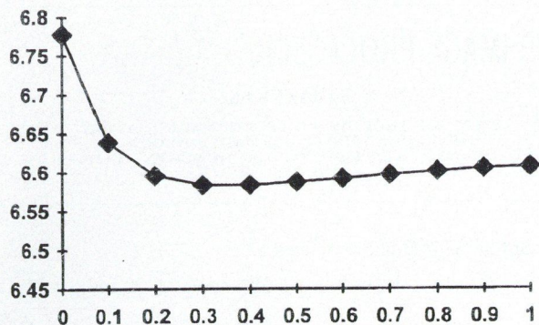
Fig. 5. Mean-square-error of the algorithm as a function of Q for frames 33–35 of image sequence "Trevor White"
