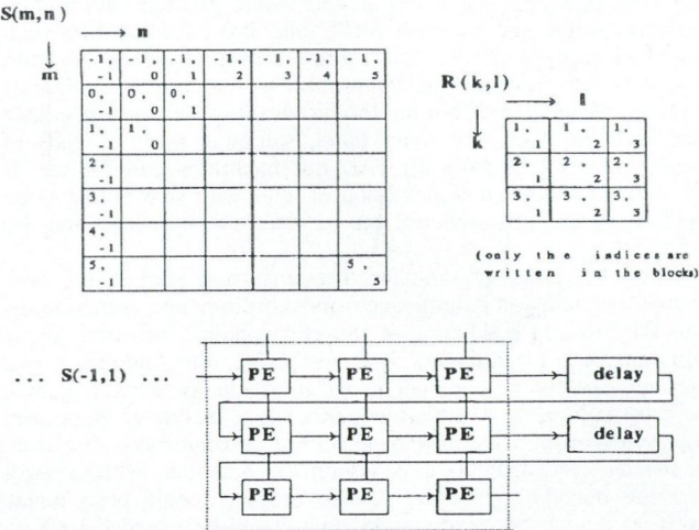
Fig. 6. The operation of a simplified BMA
