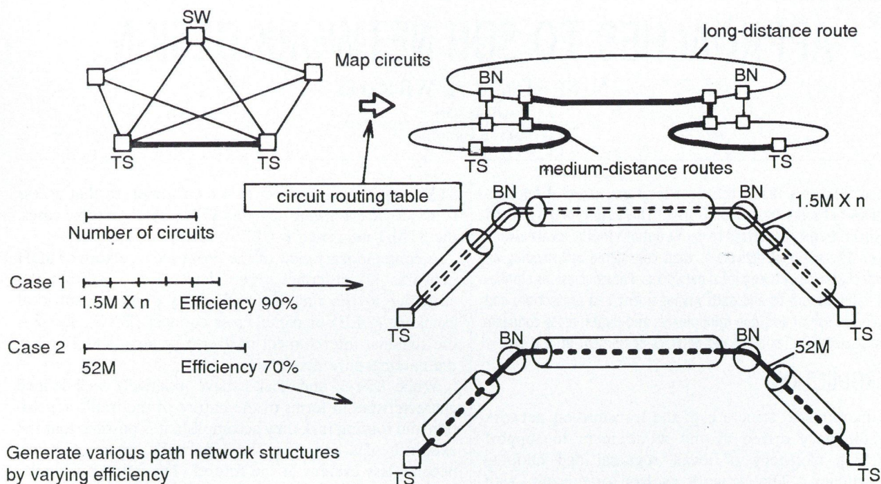
Fig. 9. Path network generation
