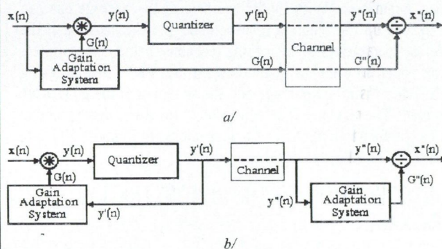
Fig. 2. The feedback (a) and the feed-forward (b) structures for gain adaptation of quantizers
