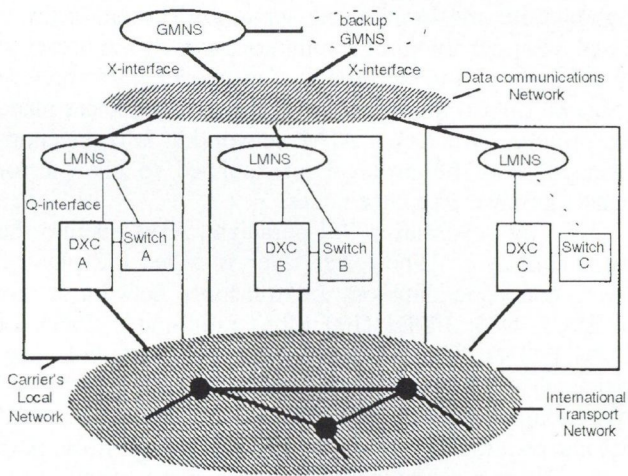
Fig. 4. GNP Network Management Architecture
