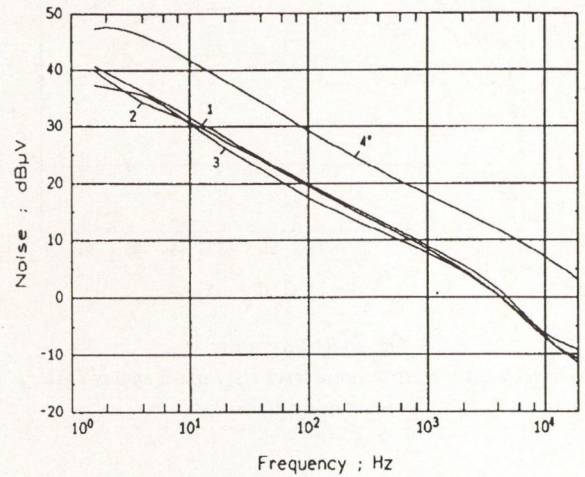
Fig. 7. The noise spectra of the TLM pattern
