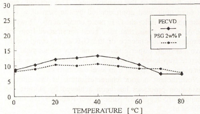
Fig. 7. Typical plots of the NPR vs. temperature for PECVD passivation. Conventional PECVD and modified PECVD in phosphorous ambient (PSG) are compared for GaAs.
