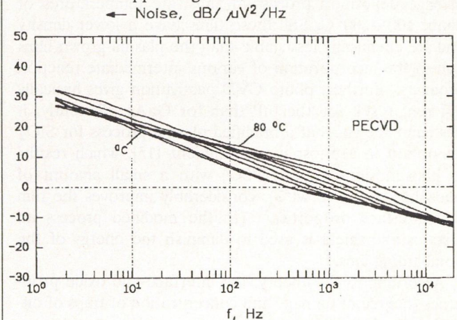
Fig. 8. Typical temperature-dependence of the low-frequency noise spectrum for InP in the temperature range of 0—80°C. The sample was passivated by conventional PECVD technology.
