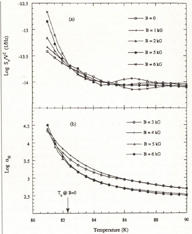
Fig. 2. \text{YBa}_2\text{Cu}_3\text{O}_{7-\delta} thin film on \text{LaAl}_2\text{O}_3 : Normalized voltage noise power spectral density at 5 Hz vs. temperature for different values of applied magnetic field, B . In (a) the normalization was done with respect to only applied voltage. In (b) the normalization was done with respect to voltage and Hall-carrier density.
