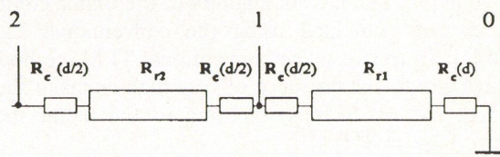
Fig. 5. The equivalent circuit of the TLM pattern
