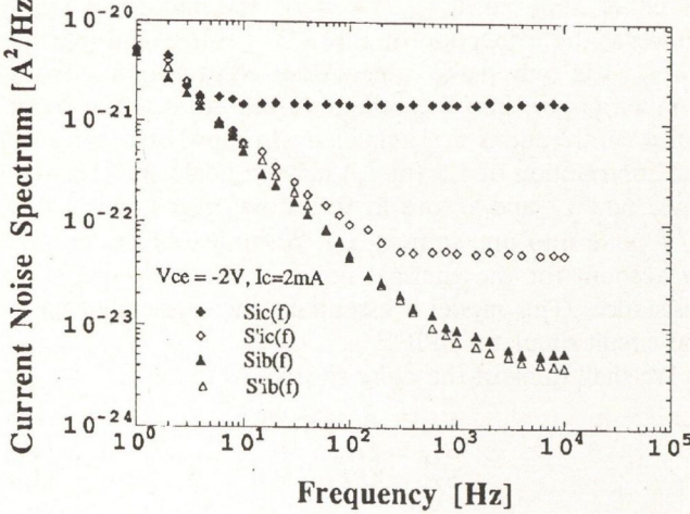
Fig. 3. Current noise spectra (base and collector, with and without feedback) taken from GE-82 pnp bipolar transistor biased at I_C = 2 mA and V_{CE} = -2 V. See [4] Fig. 4, device 1.
