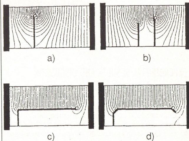
Fig. 1. Trimming cuts
