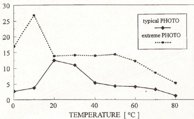
Fig. 6. Plots of the noise factor NPR vs. temperature for photo-CVD passivated GaAs resistor chips. Typical values have been obtained from most of the analyzed chips. Extreme values are not unique, they did occur on the same wafer.
