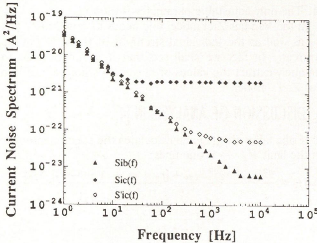
Fig. 4. Current noise spectra (base and collector, with and without feedback) taken from GE-82 pnp bipolar transistor biased at I_C = 2 mA and V_{CE} = -2 V. See [4] Fig. 6, device 2.
