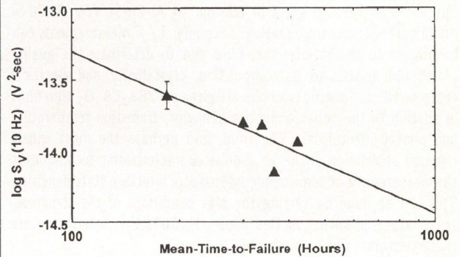
Fig. 1. TiW/W/2% Cu-Al thin films: Voltage noise power spectral density at 10 Hz vs. Mean-Time-to-Failure for five wafers. Noise measurements were performed at T = 150^\circ\text{C} with the samples biased with J = 4 \times 10^6 \text{ A/cm}^2 . Life-time tests were done at T = 200^\circ\text{C} ( T_{\text{stripe}} = 216^\circ\text{C} ) and J = 2 \times 10^6 \text{ A/cm}^2 . The least-squares fitted line shows an inverse relationship between these parameters.
