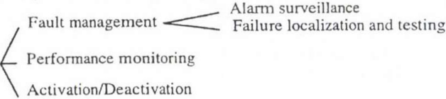
Fig. 3. OAM function for the F4 flow
