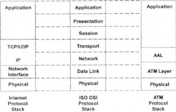
Fig. 5. Comparison of Internet, ISO OSI and ATM protocol stacks
