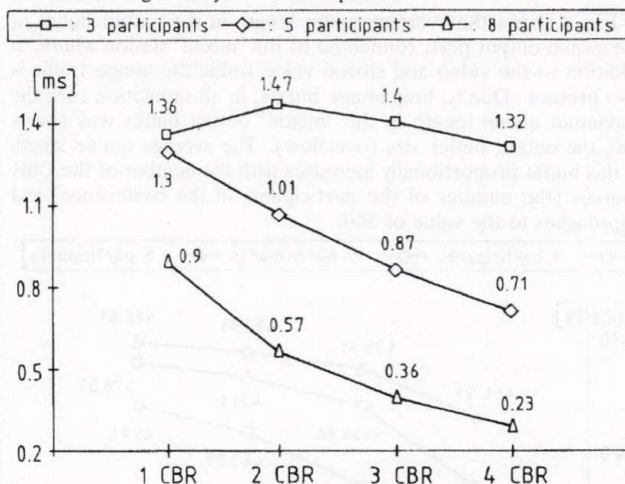
Fig. 8. Average delays at the switch
