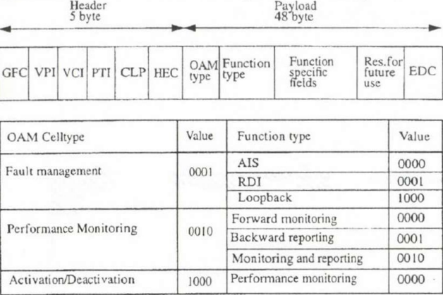
Fig. 4. The format of the OAM cell
