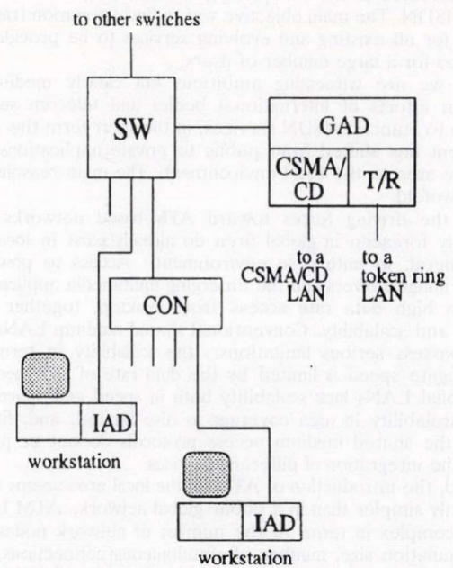
Fig. 1. An ATM LAN configuration example containing all four building blocks, where SW: ATM switch, CON: concentrator, GAD: group access device, IAD: individual access device.
