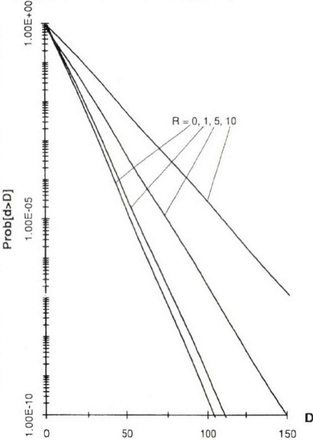
Fig. 6. \text{Prob}[d > D] versus D , \sigma = 0.9 , R = 0, 1, 5, 10
