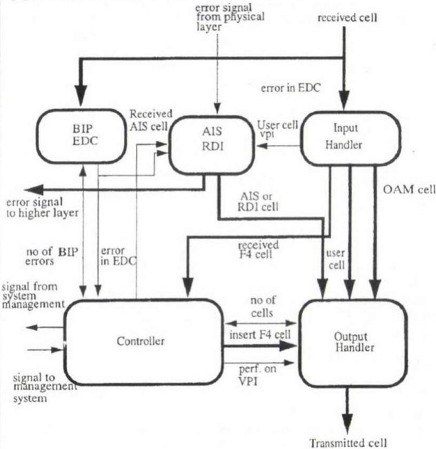
Fig. 9. Architecture of the F4 block
