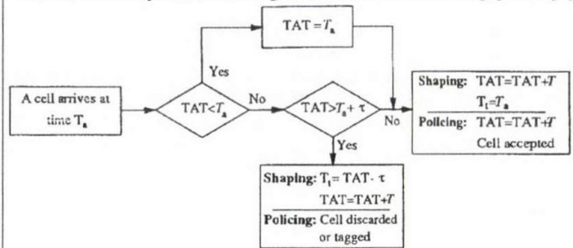
Fig. 2. Flow diagram of the Generic Cell Rate Algorithm used for shaping and policing: T_a = arrival time of a cell; T = nominal cell interarrival time; \tau = cell delay variation tolerance; T_i = transmission time of a cell; TAT = theoretical arrival time of a cell
