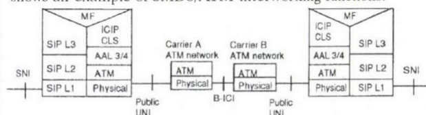
Fig. 10. SMDS/ATM interworking; where MF: mapping function
