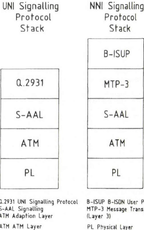
Fig. 6. ATM UNI and NNI Signalling Protocol Stacks
