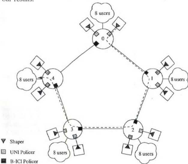
Fig. 1. Model of the interconnected ATM network system
