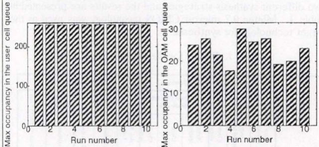
Fig. 11. Simulation results
