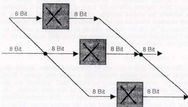
Fig. 5. Performance expansion
