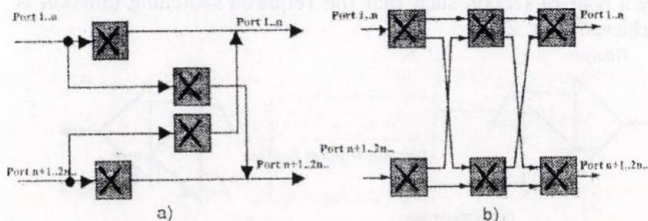
Fig. 3. Switch-on-a-chip port expansion a) single-stage port expansion; b) multi-stage port expansion
