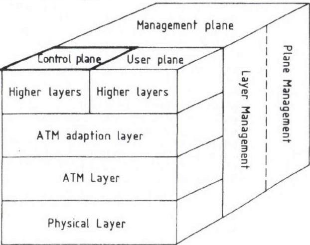
Fig. 1. ATM Protocol Reference Model
