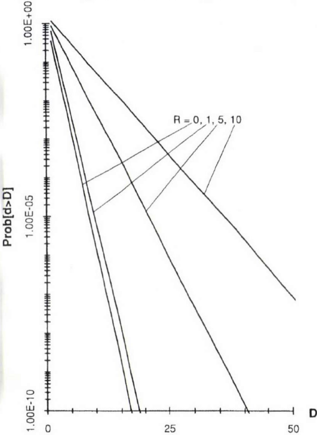
Fig. 5. \text{Prob}[d > D] versus D , \sigma = 0.5 , R = 0, 1, 5, 10
