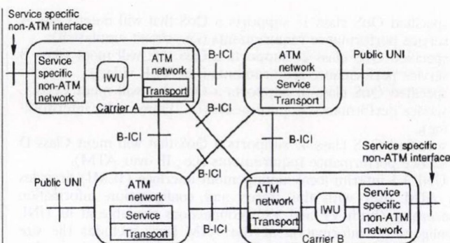
Fig. 6. A generic view of service specific networks inter-connected via ATM networks
