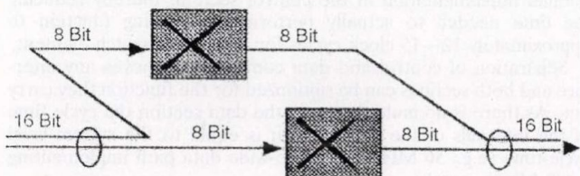
Fig. 4. Speed expansion
