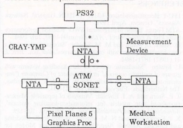
Fig. 1. Traffic Data Collection Sites
