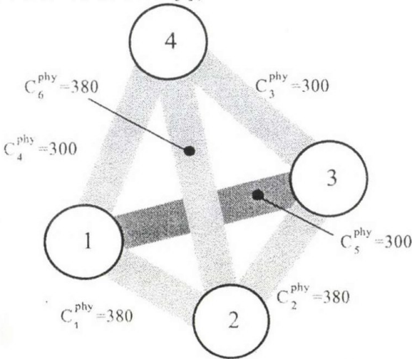
Fig. 1. The four node fully connected network
