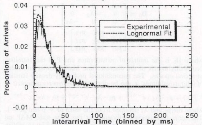
Fig. 7. Adapted ATM Burst Interarrival Density Function
