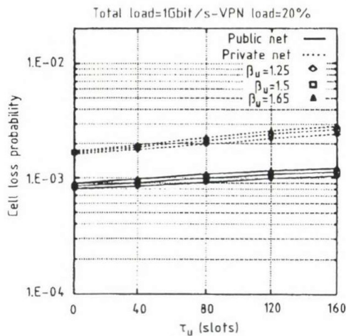
Fig. 4. Diagrams of cell loss probability and End-to-End delay versus \beta_u and \tau_u . The figure is referred to the case where a shaping function is implemented at each private user's premise.
