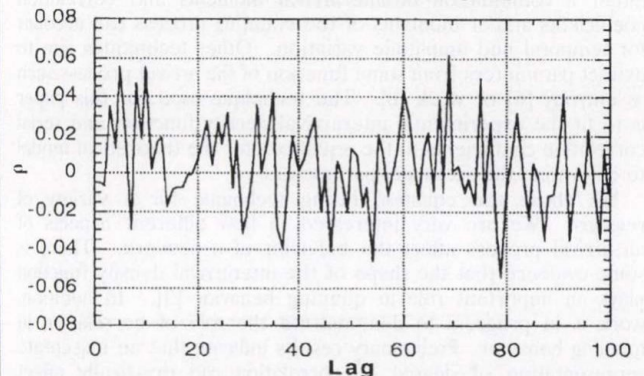
Fig. 8. Burst Interarrival Time Serial Correlation Coefficients
