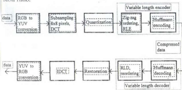
Fig. 1. The JPEG standard algorithm's baseline structure
