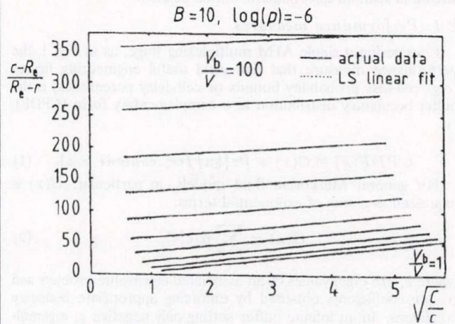
Fig. 2. Effective rate versus output capacity
