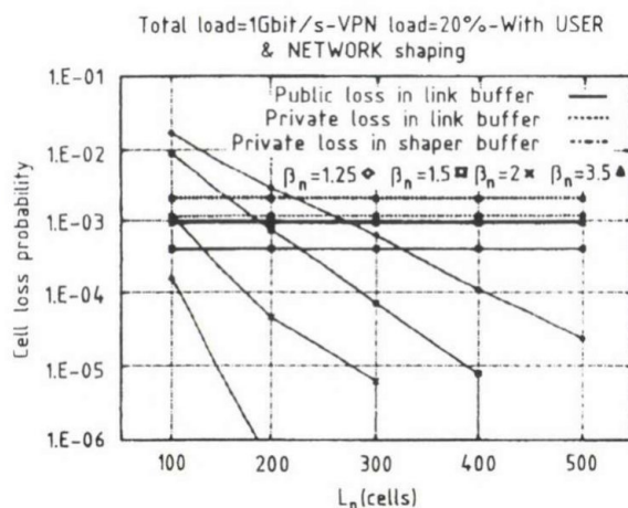
Fig. 8. Diagram of cell loss probability versus L_n and \beta_n . The figure shows separately the losses at the link-buffers and that at the shaper-buffers, and is referred to the case where a two-level (users and network) shaping function is operated on the private traffic.
