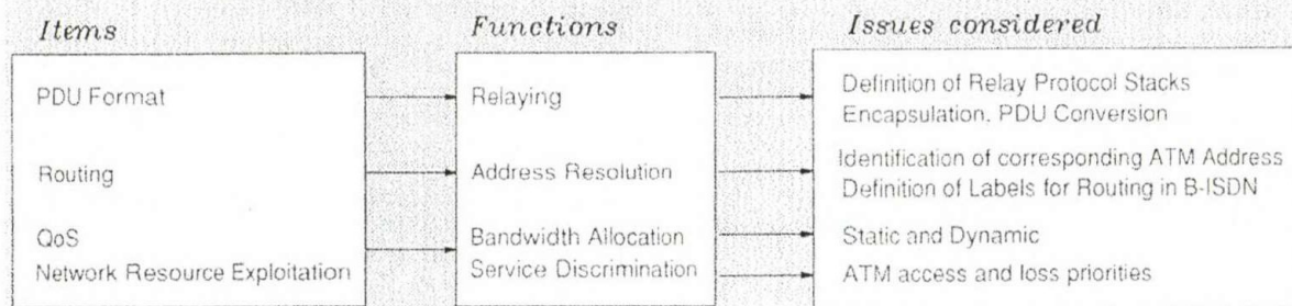
Fig. 1. AIU's scope and functions
