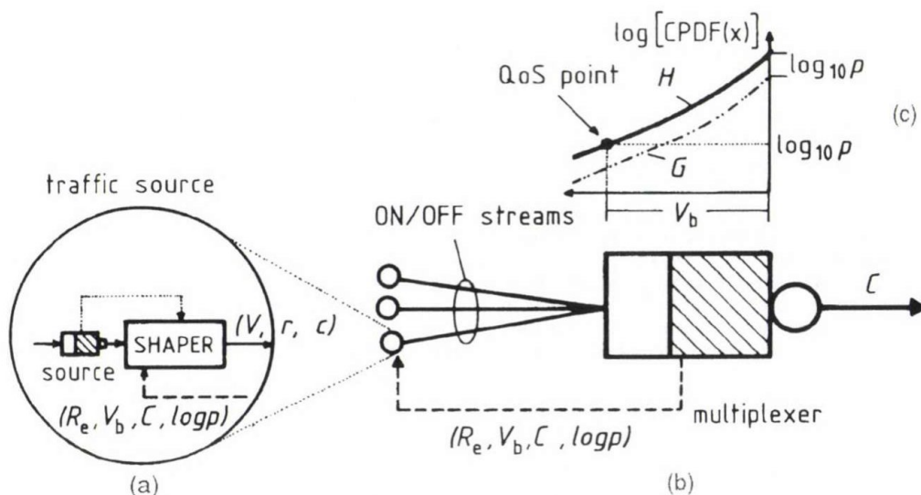
Fig. 1. An ATM statistical multiplexing environment. (a) traffic sources with adaptive shaping capabilities; (b) multiplexer; (c) complementary distribution of buffer occupancy
