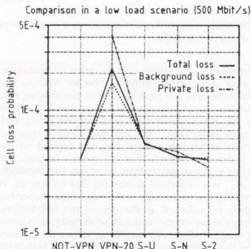
Fig. 10. Diagram of the improvement obtained in a low load scenario with the different traffic shaping strategies.
