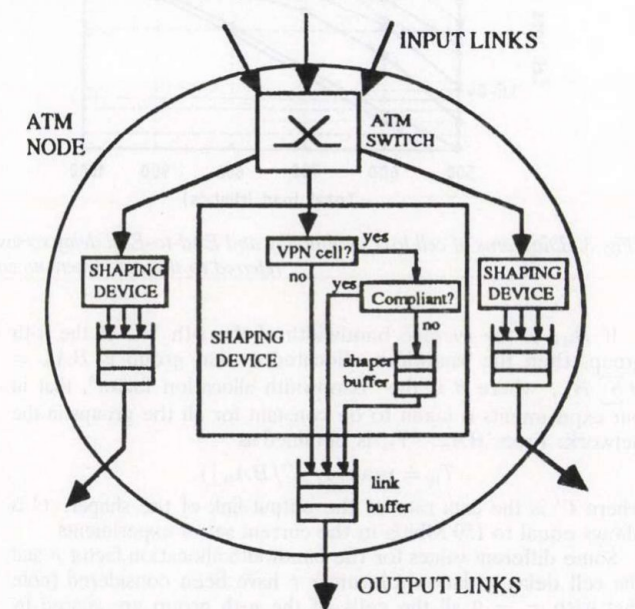
Fig. 5. Architecture of the traffic shaping mechanism implemented inside the ATM network.
