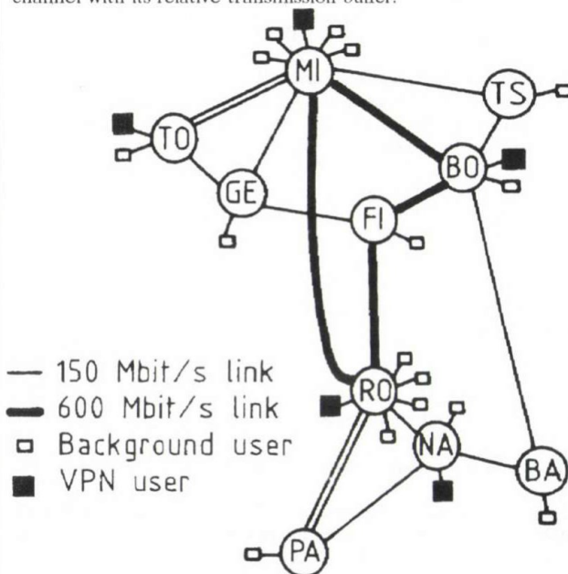
Fig. 2. Topology of the simulated network. The B-VPN users are marked.
