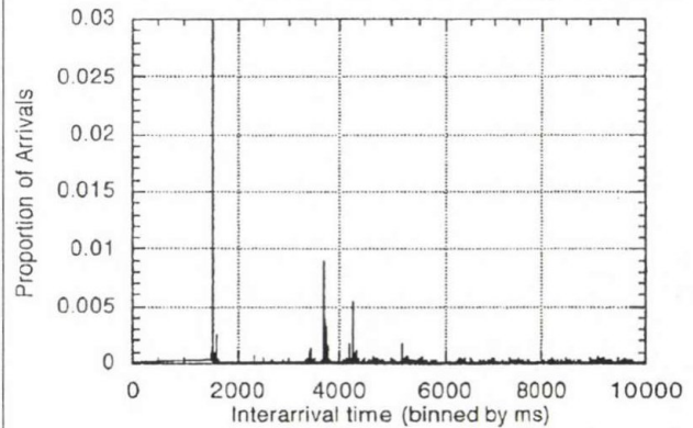
Fig. 2. Packet Interarrival Time Density Function
