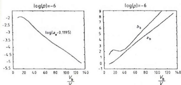
Fig. 4. Parameters a_a , a_b , b_b versus mean volume of bursts
