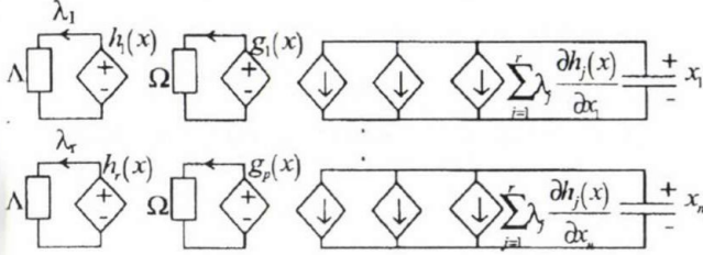
Fig. 2. The modified nonlinear programming circuit
