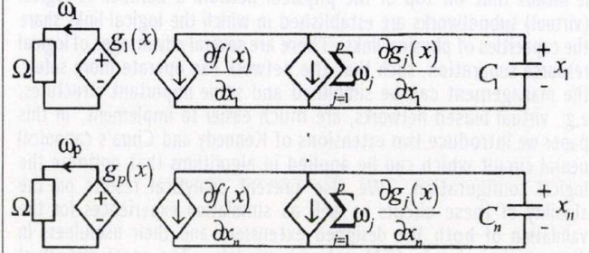
Fig. 1. The canonical nonlinear programming neural circuit of Kennedy and Chua
