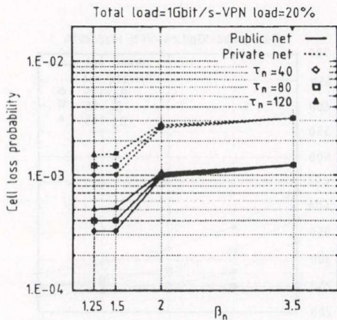
Fig. 6. Diagrams of cell loss probability and End-to-End delay versus \beta_n and \tau_n . The figure is referred to the case where a shaping function is implemented inside the ATM network on the whole traffic of each VP used by the Private Network.
