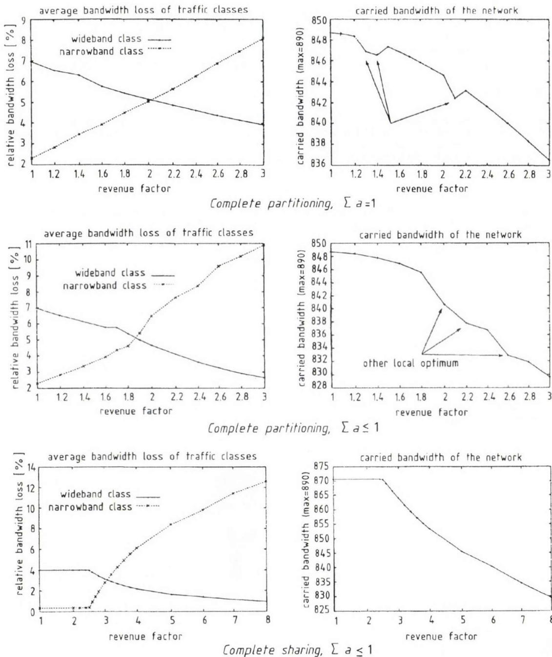
Fig. 4. Tuning w_r of a traffic class in the 5 node network
