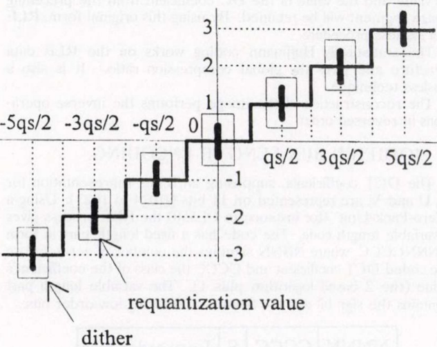
Fig. 3. Requantization with dither
