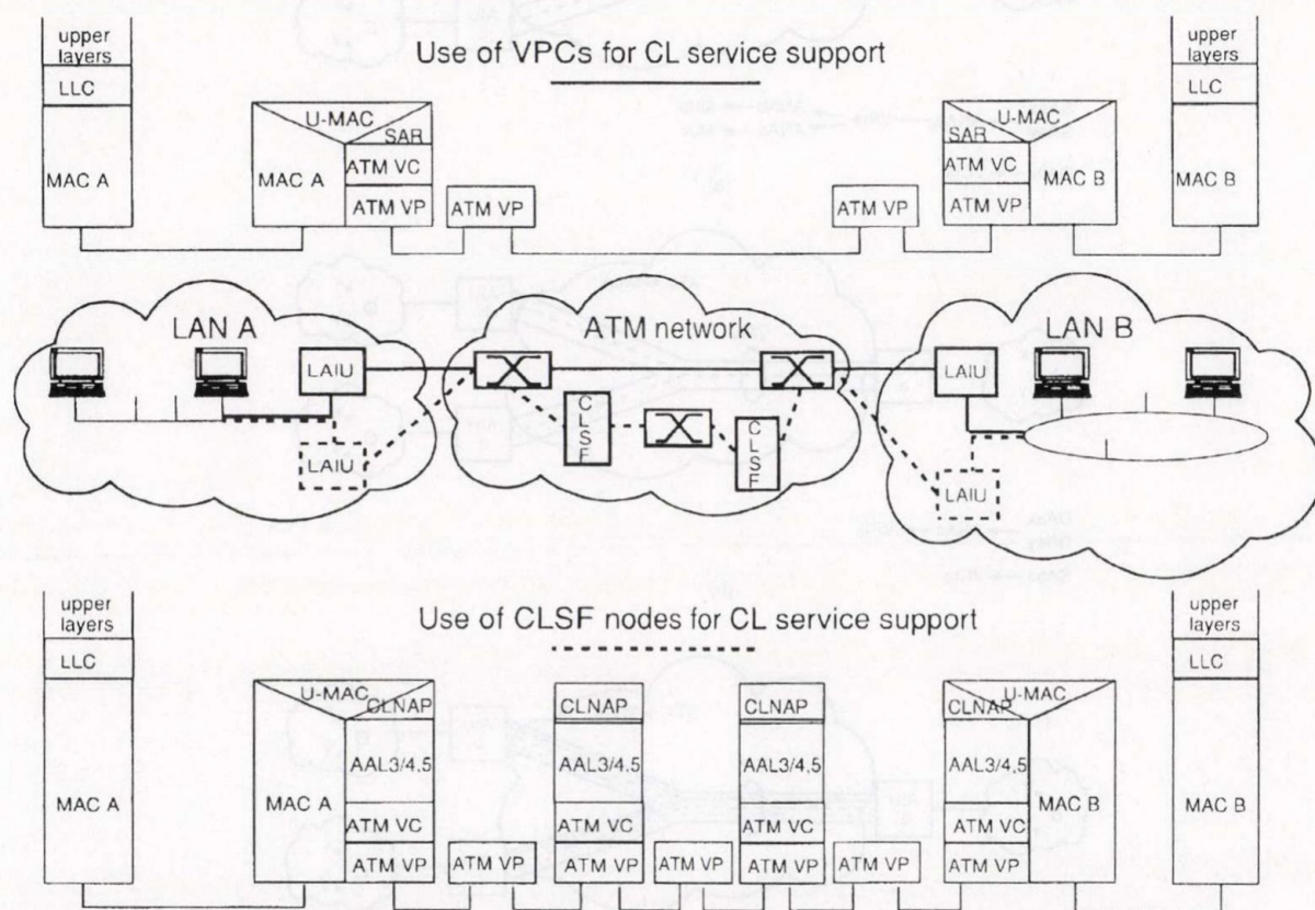
Fig. 5. AIU protocol stacks for IEEE 802.3-5 LAN interconnection
