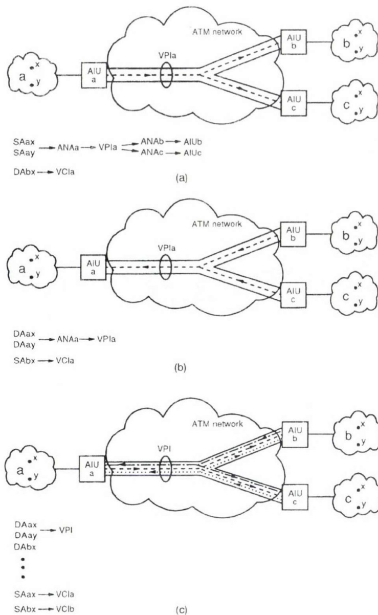
Fig. 4. Configurations and usage of VCI with the ITU-T mechanism for CL service support
