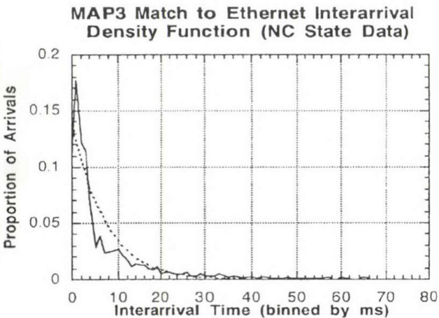
Fig. 9. MAP3 Match to Ethernet Interarrival Density Function (NC State Data)
