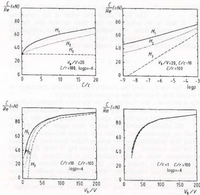
Fig. 7. Maximum number of admissible connections with the three control laws. (a) versus peak rate; (b) versus overflow probability; (c), (d) versus buffer size
