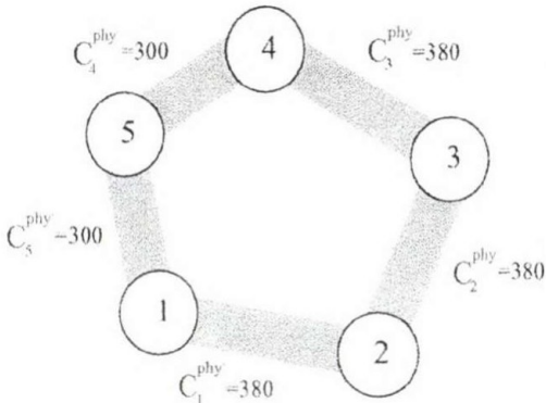
Fig. 2. The five node ring
