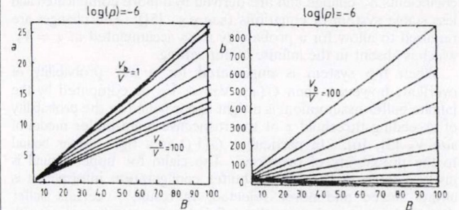
Fig. 3. Parameters a and b versus burstiness
