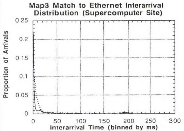
Fig. 10. MAP3 Match to Ethernet Interarrival Distribution (Supercomputer Site)
