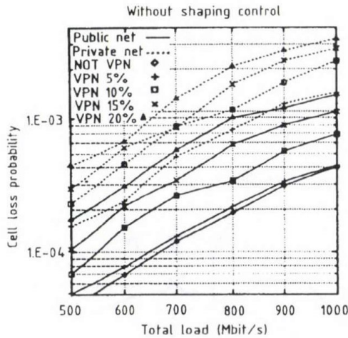
Fig. 3. Diagrams of cell loss probability and End-to-End delay versus total network load and private network load percentage. The figure is referred to the case where no control exists on the private traffic.
