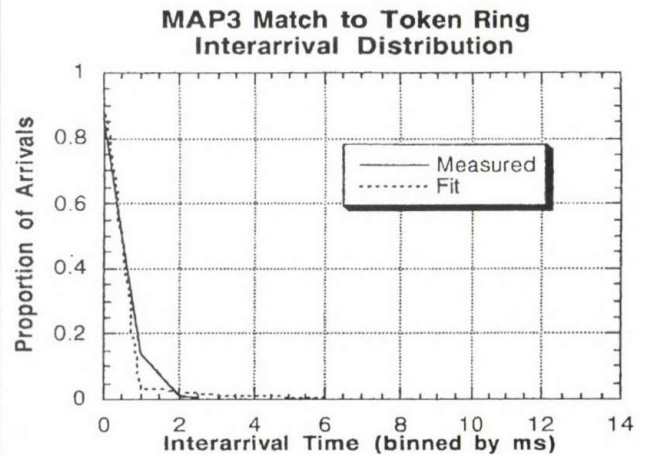
Fig. 11. MAP3 Match to Token Ring Interarrival Distribution
