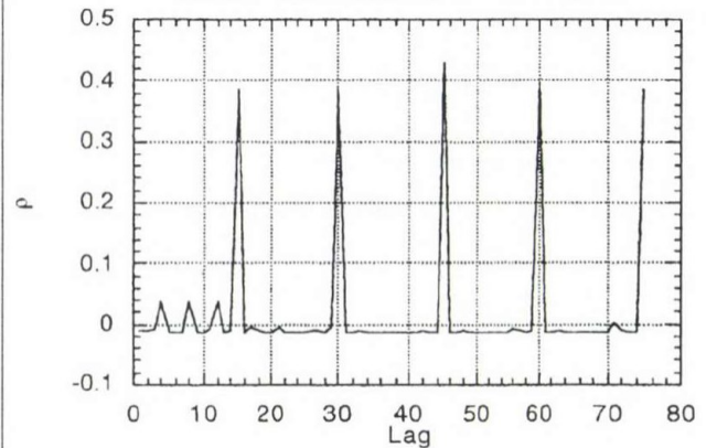
Fig. 3. Serial Correlation Coefficients
