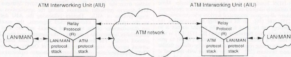
Fig. 2. ATM interworking unit protocol stack overview
