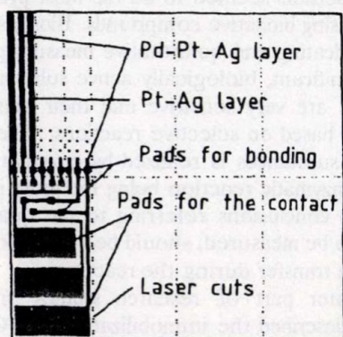
Fig. 7. The electrode structure of the biosensor
