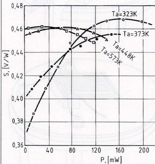
Fig. 6. Power sensitivity as a function of power dissipated in the heater. (Circular construction — Fig. 1a — working as r.m.s. sensor.) The end of the measurement range due to overloading can be seen for ambient temperatures of 448 K and 573 K.
