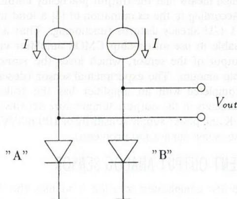
Fig. 1. Principle of a bipolar PTAT sensor
