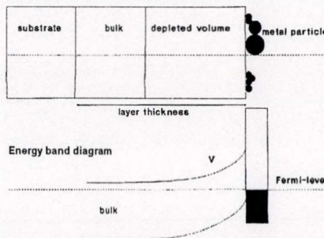
Fig. 1b. Schematic cross-section of a semiconductor thin film surface with metal particles
