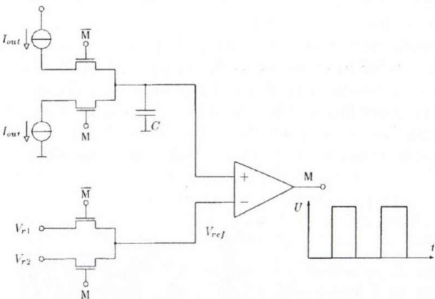
Fig. 6. Frequency-output temperature sensor based on the current-output cell of Fig. 3
