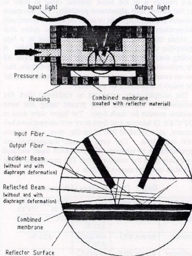
Fig. 3. The cross-section of the flexible membrane fibre-optic intensity pressure sensor
