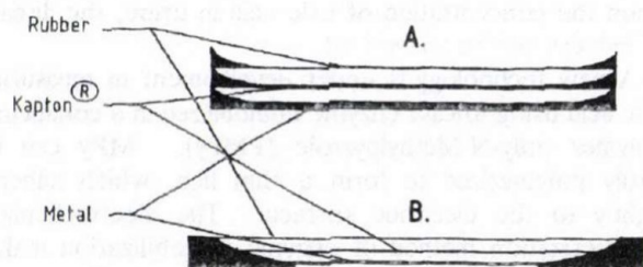
Fig. 4. Multilayer pressure sensitive flexible membranes using different frames
