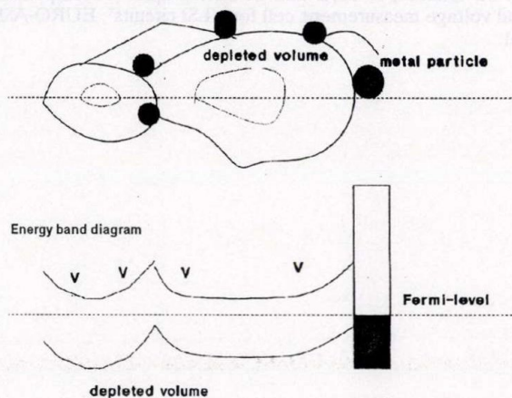
Fig. 1a. Schematic cross-section of a grainy semiconductor material with metal particles (model of sintered thick sensor layer)
