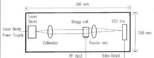
Fig. 4. The optical system of the MW RTSA
