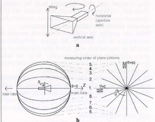
Fig. 1. a) Moving modes necessary for directing an antenna to any direction. b) The method of measuring a three-dimensional antenna pattern.
