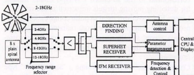
Fig. 2. ESM receiver configuration with DF capabilities
