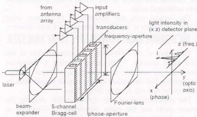
Fig. 5. Direction finding system based on a 5-channel DOAP
