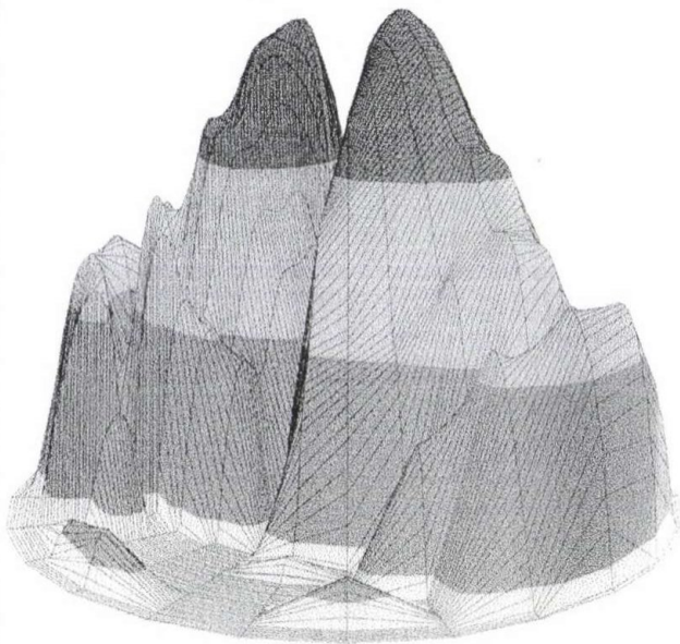
Fig. 7. Three-dimensional pattern of a microstrip antenna represented in cylindrical co-ordinate system
