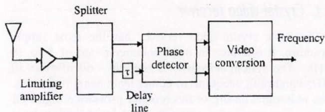
Fig. 1. Instantaneous Frequency Measurement
