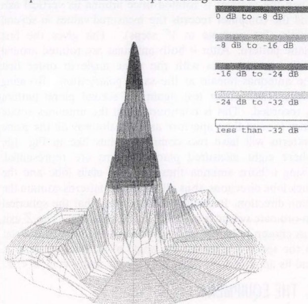
Fig. 4. Three-dimensional pattern of a horn antenna represented in cylindrical co-ordinate system
