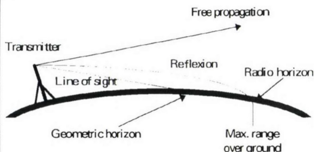
Fig. 6. VHF-UHF Wave Propagation
