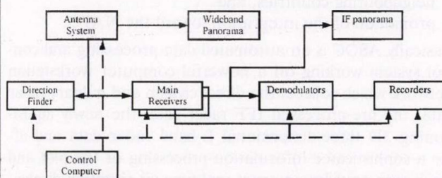
Fig. 2. General structure of radio reconnaissance station
