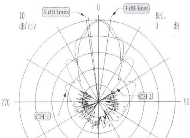
Fig. 2. E (CH2, \varphi = 90^\circ ) and H (CH1, \varphi = 0^\circ ) plane pattern of a horn antenna in polar co-ordinate system
