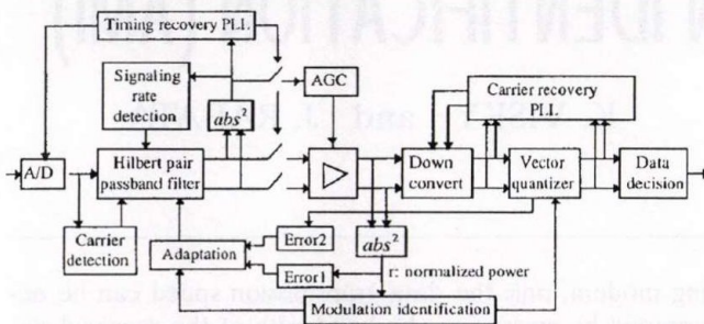
Fig. 2. Block diagram of the universal demodulator
