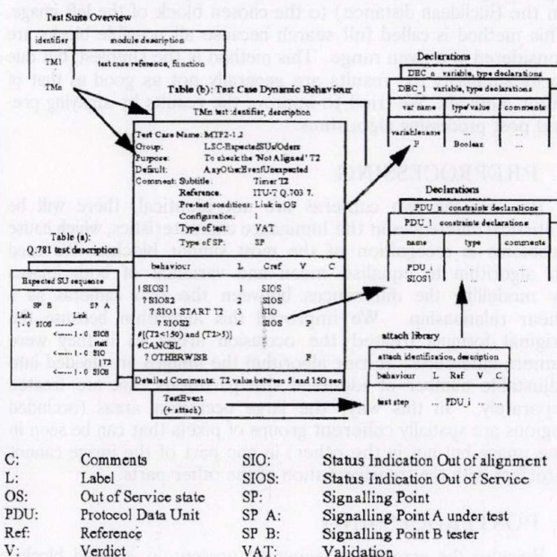
Fig. 1. Illustration of abstract test suite in TTCN
