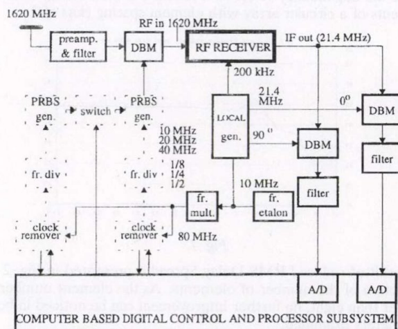
Fig. 1. The receiver of the sounder. The functions implemented by XILINX module are shown with dotted border.
