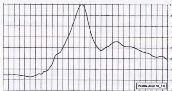
Fig. 2. Delay profile. Elevation angle 60°, full circle. Average delay spread = 57.83 ns.
