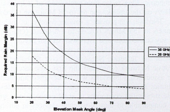
Fig. 2. Required Rain Margin (Region D2, 99.9 % Availability)
