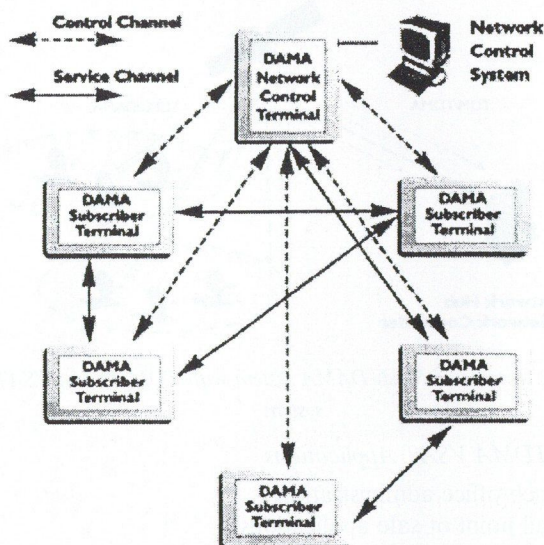
Fig. 5. Mesh-DAMA connections
