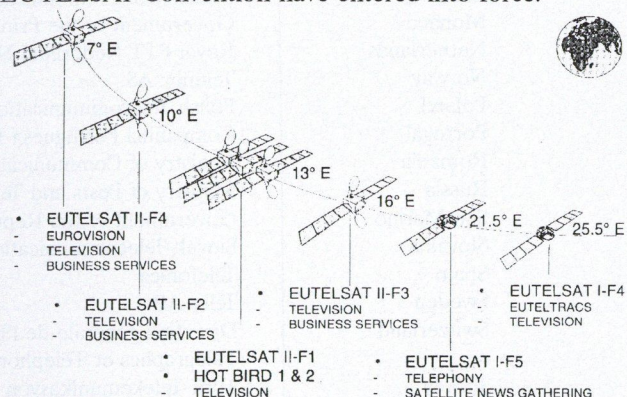
Fig. 1. The EUTELSAT System in January 1997
