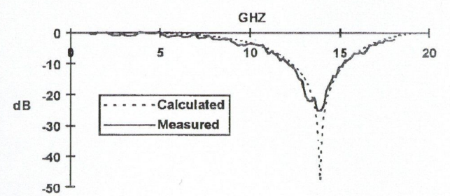
Fig. 3. Measured and calculated fiber transmission, L = 18 km, D = 9 \frac{ps}{km \cdot nm}
