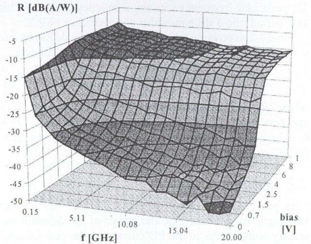
Fig. 5. Responsivity of 12 \times 12 \mu\text{m}^2 photodiode P_{opt} = 323 \mu\text{W} , f = 0.45 \text{ GHz} \dots 20 \text{ GHz}
