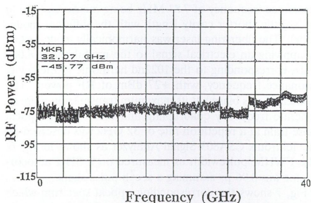
Fig. 8. Measured RF spectrum of 32 GHz optical pulse train (RBW = 300 kHz, VBW = 10 kHz)
