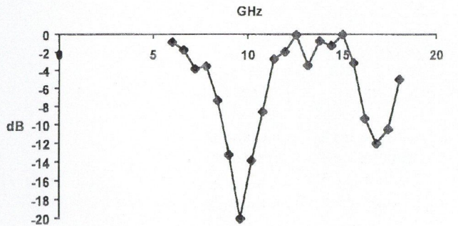
Fig. 4. Measured transmission, L = 38.6 km
