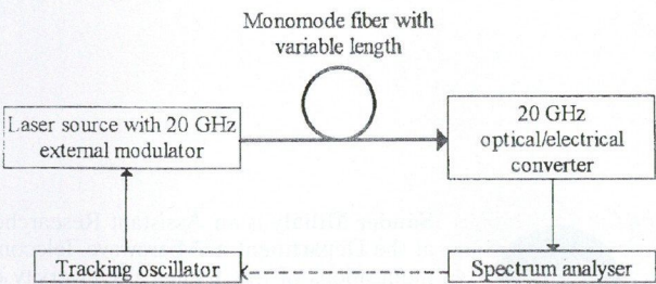
Fig. 2. Measurement setup
