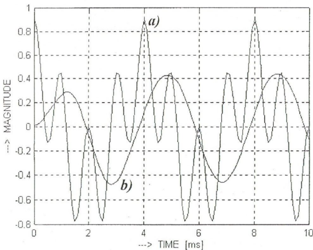
Fig. 8. Testing signals for the lattice lowpass filter: a) input signal x(n) , b) out signal y(n)
