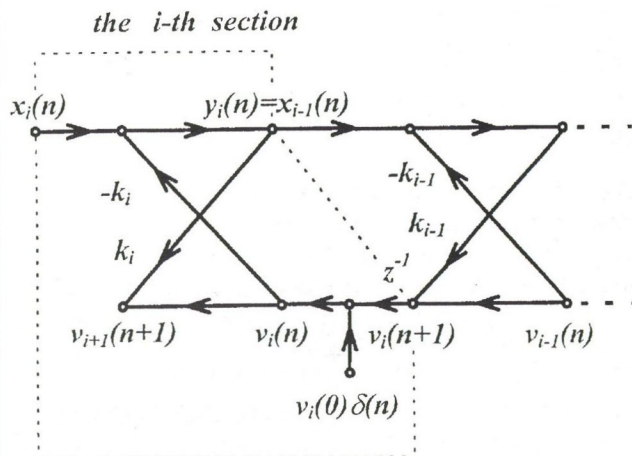
Fig. 2. The i -th lattice section with two multipliers
