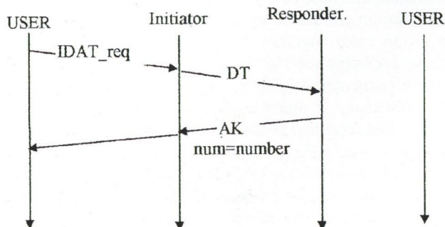
Fig. 8. Time-Sequence diagram
