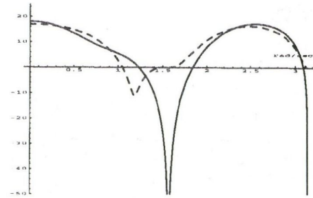
Fig. 5. STF and NTF transfer characteristics
