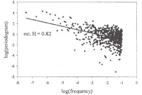
Fig. 8. Periodogram plot of IP data set
