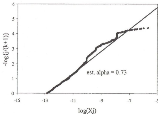
Fig. 4. The modified QQ-plot estimation of WFS data set
