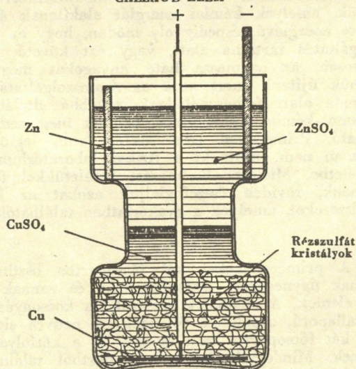
CALLAUD ELEM
