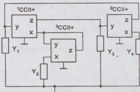
Fig. 7. Autonomous circuit with characteristic equation (CE) Y_1 Y_3 + Y_2 Y_4 = 0
