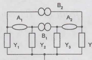
Fig. 1. Two nullors on a ring circuit
