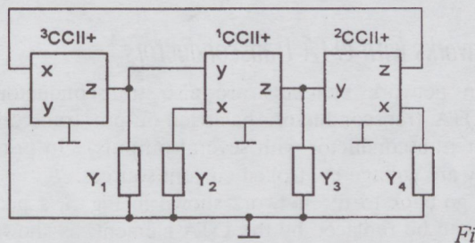
Fig. 8. Autonomous circuit with the same CE as that in Fig. 7
