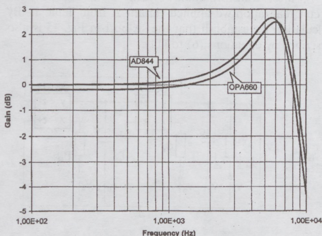
Fig. 19. Detailed comparison of voltage mode frequency gain response of LPF using AD844 or OPA660
