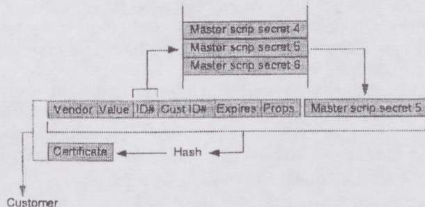
Fig. 3. The certificate of a piece of scrip is generated by hashing the body of the scrip with a secret. The secret is selected using a portion of the scrip's ID#.
