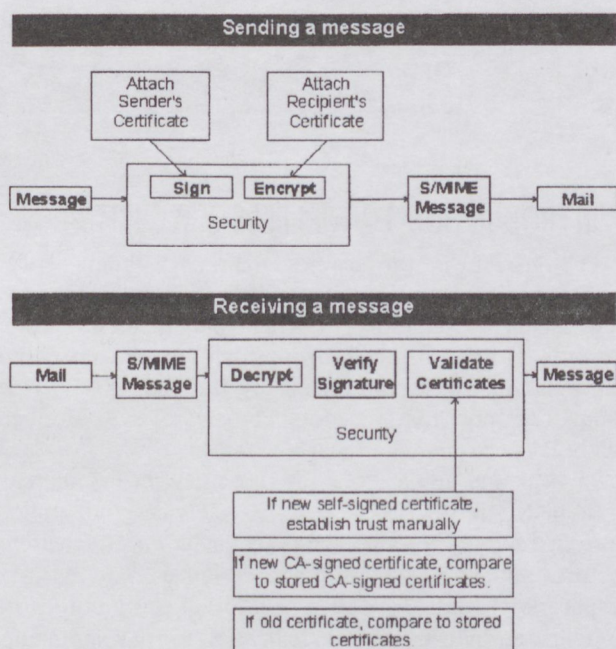
Fig. 8. Sending and receiving messages using SMT
