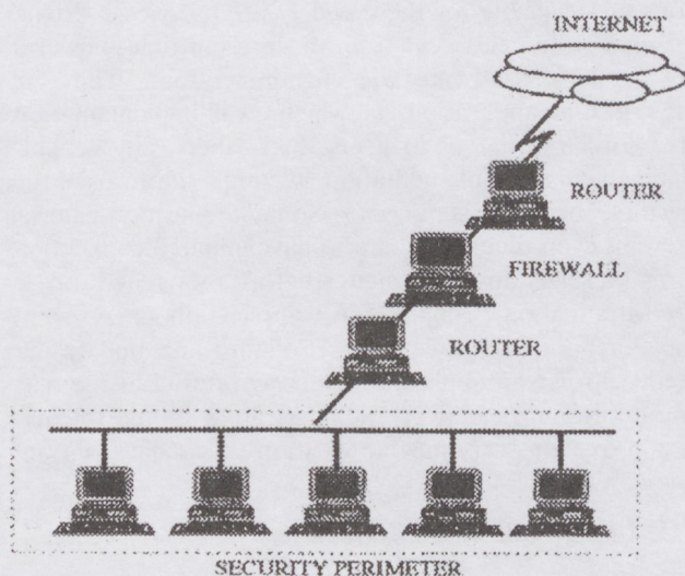
Fig. 8. A Typical Gate-Based Firewall Architecture
