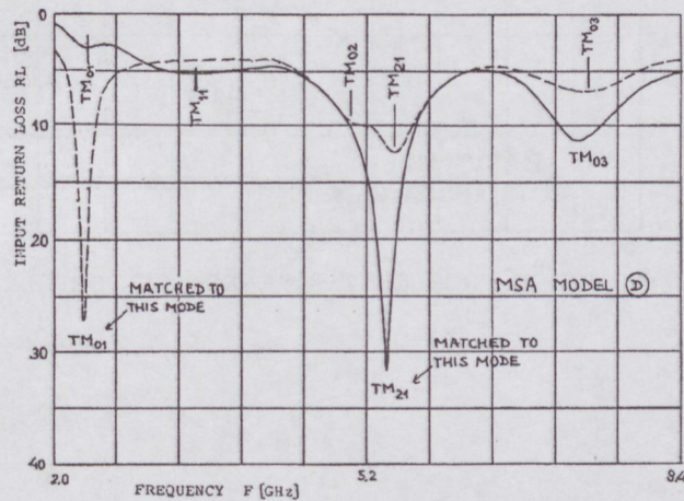
Fig. 5. Input return loss versus frequency for Model-D
