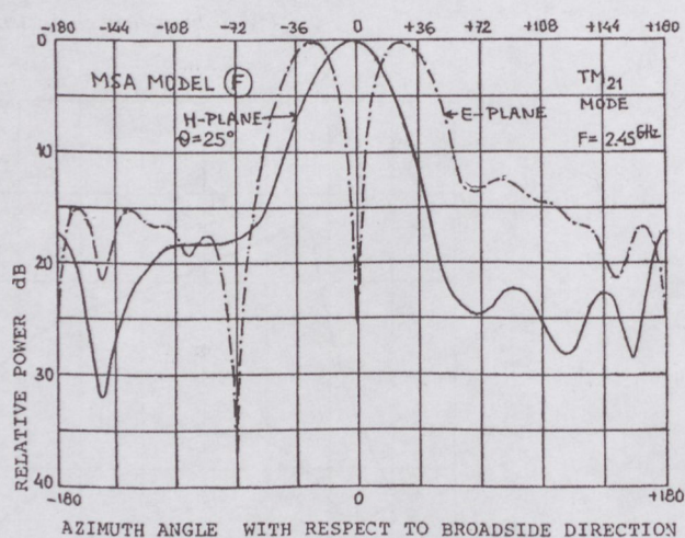
Fig. 12. Far-field characteristics for Model-F in TM 21 mode
