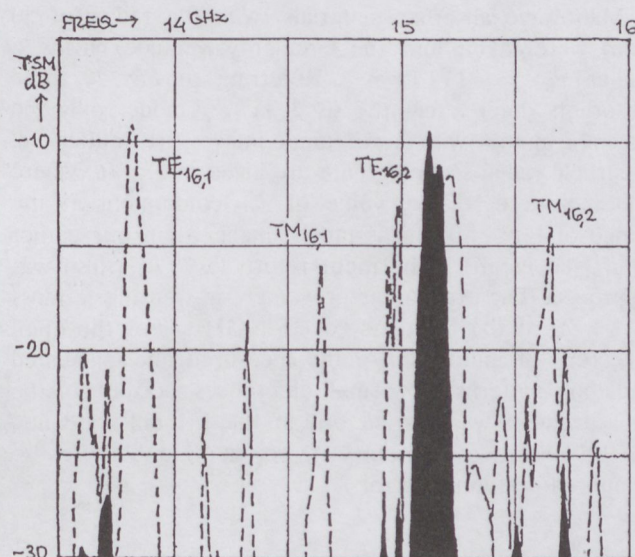
Fig. 8. Measured transmission characteristic of closed structure (black shadowing: using irises).
