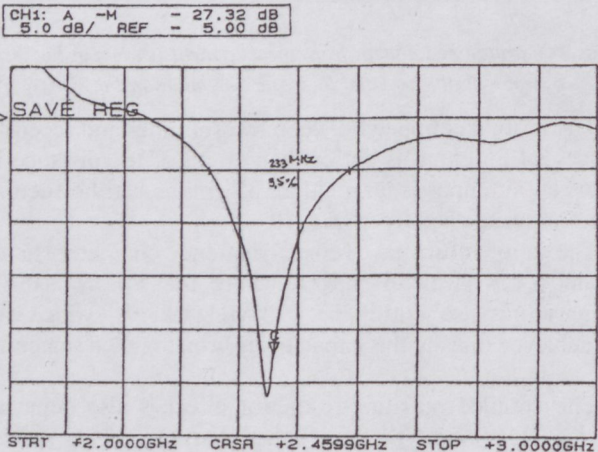
Fig. 11. Measured input return loss versus frequency for FXS antenna Model S.1
