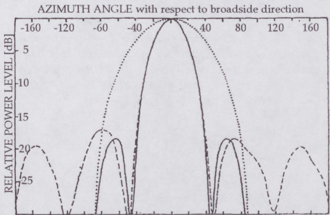
Fig. 3. Calculated H-plane radiation characteristics for single element (... line) and four element passive array at the frequency of f_{\text{max}} . Measured values, for varactor tuned MSA are also shown (dotted line).
