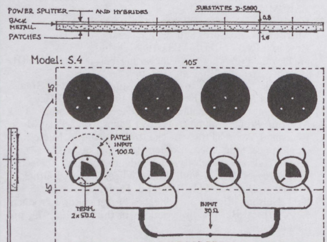
Fig. 1. RHCP-array for FXS at 5.8 GHz
