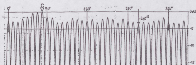
Fig. 7. Azimuthal scanning of the E_r -component.
