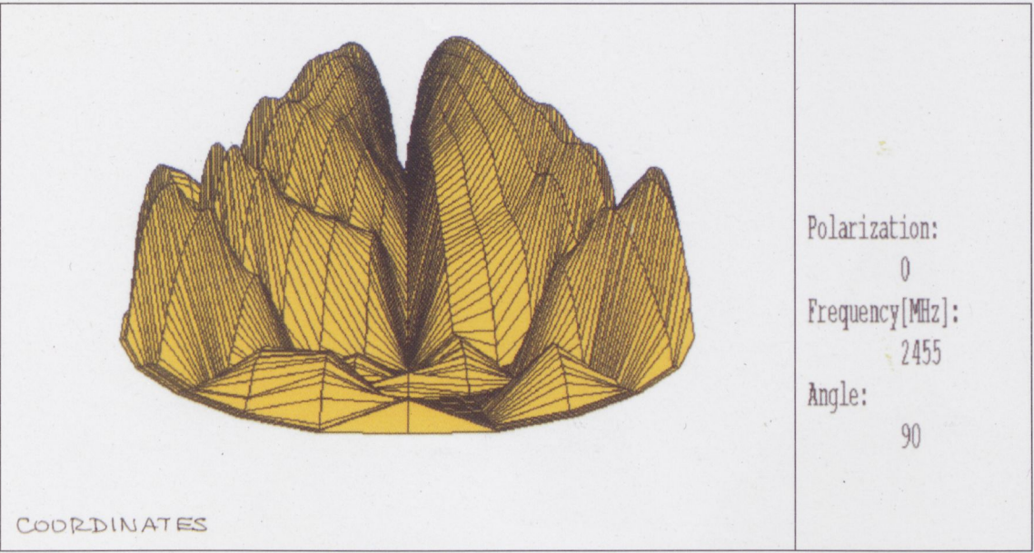
Fig. 13. Stereoscopic radiation of Model S.3, depicted in cylindrcal coordinates.
