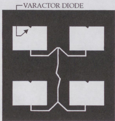
Fig. 4. Frequency Agile Microstrip Antenna (FAMSA). Outer dimensions of the 4-element module: 10 \times 10 \times 0.08 \text{ cm}^3 , substrate material: 3M-Cuclad-217. Tuneability: 10 %, gain at f_{\text{max}} is 12.7 dB, half power beamwidth nearly 36^\circ and 46^\circ are, respectively. Instantaneous bandwidth is 1.5 %.
