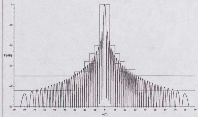
Fig. 10. Calculated E-plane radiation pattern of the 64 \times 64 element MSA-array with uniform amplitude distribution. The lower tolerance-lines show the IEEE-recommendation for side-lobe reduction.
