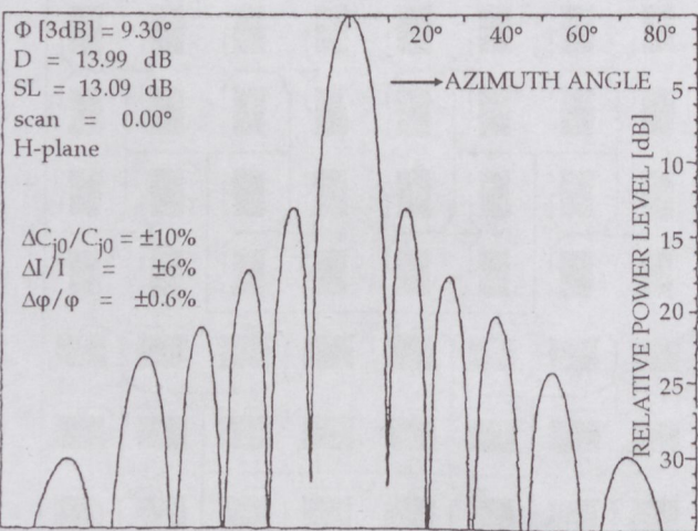
Fig. 7. Calculated H-plane pattern for the given capacitance matching
