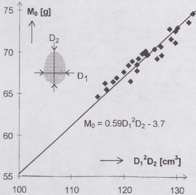
Fig. 4. Measured "fresh-mass" versus dimensions of eggs
