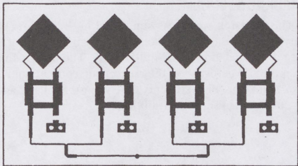
Fig. 20. Circularly polarized TX (and RX) antenna with 90° hybrids and the microstrip power splitter.
