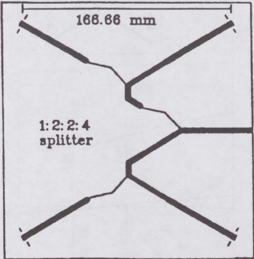
Fig. 5a. The reactive, 1:2:2:4 splitter.
