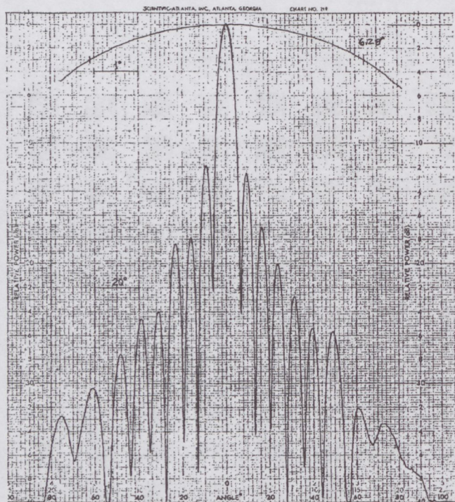
Fig. 8. Measured H-plane radiation pattern of the 8 × 16 element MSA-array.
