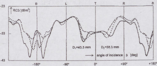
Fig. 10. Measured RCS of an egg versus angle of incidence. Various kinds of curves are shown depending on the geometrical positioning. The bistatic angle and frequency are 30° and 14.2 GHz, respectively.
