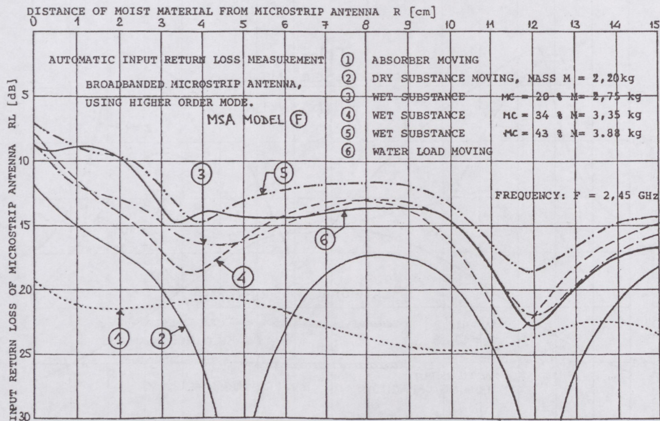
Fig. 10. Near-field reflections from wet substances
