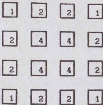
Fig. 3. Relative amplitudes of the -27\text{ dB} sidelobe level MSA-array.
