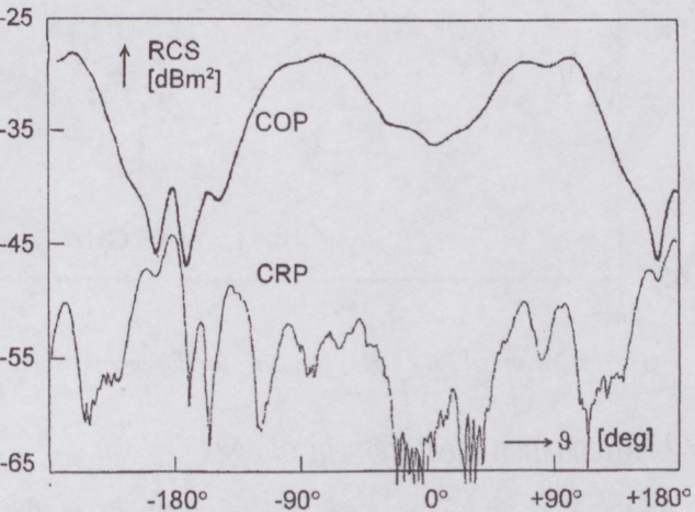
Fig. 12. Measured copolarized (COP) and crosspolarized (CRP) radar cross sections for egg
