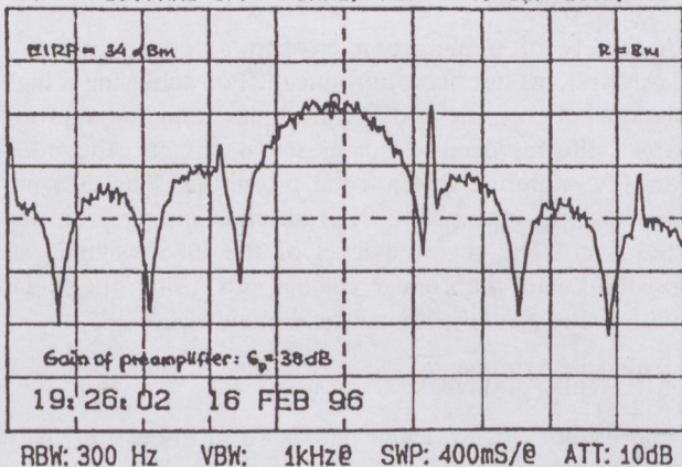
Fig. 7. Received power level versus frequency
