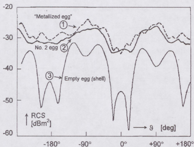
Fig. 13. Measured RCS versus angle of incidence, for different models
