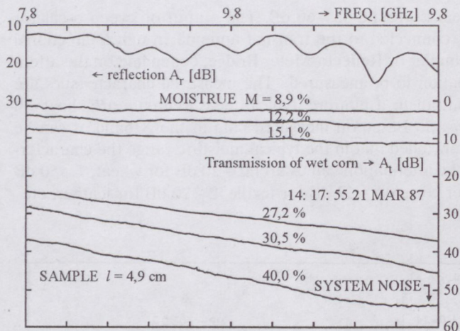
Fig. 3. Measured antenna input reflection and transmission attenuation of wet corn versus frequency
