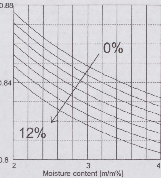
Fig. 11. \sqrt[3]{\varepsilon'} - 1/\sqrt{\varepsilon''} versus MC. Volumetric ratio of air changes 0 % and 12 % in 2 % steps.
