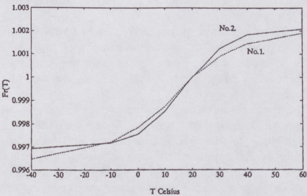
Fig. 4. Measured relative resonance frequency as a function of temperature.
