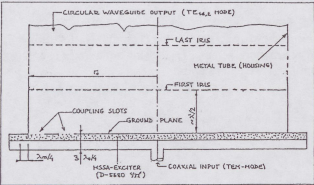
Fig. 3. Schematic of the MSSA-excited mode converter.
