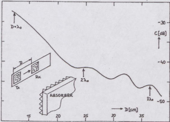
Fig. 10. Measured mutual coupling between S.1 antennas with horizontal polarization
