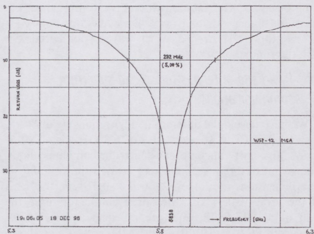
Fig. 7. Measured input return loss versus frequency characteristic of the 8 × 16 element MSA-array.
