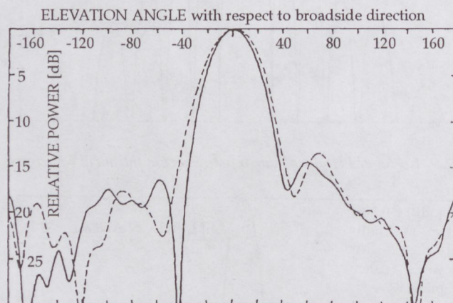
Fig. 14. Measured E-plane radiation characteristics of the four element frequency agile MSA (Fig. 2.), at the frequency of f_{\min} (dotted line, varactor bias: +0.4 V) and f_{\max} (varactor bias: -16 V).
