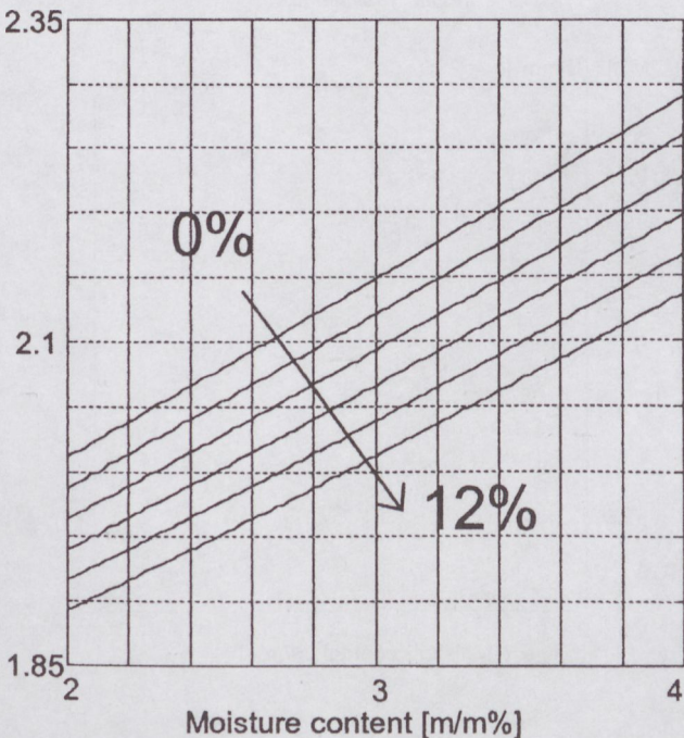
Fig. 8. \epsilon' versus MC. Volumetric ratio of air changes 0 % and 12 % in 2 % steps.
