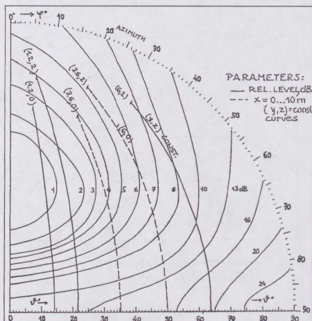
Fig. 9. Extrapolated pattern from measurement (shown in Fig. 8). These results are used to create S.3 values in Fig. 3.
