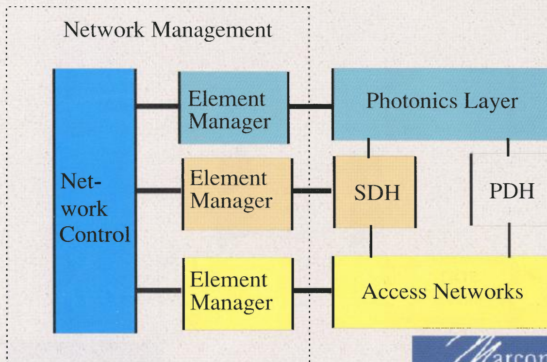
Figure 8. Network management architecture
