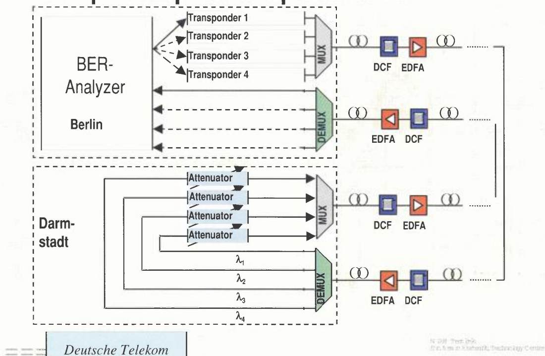
12. Setup of loop back experiment II.
