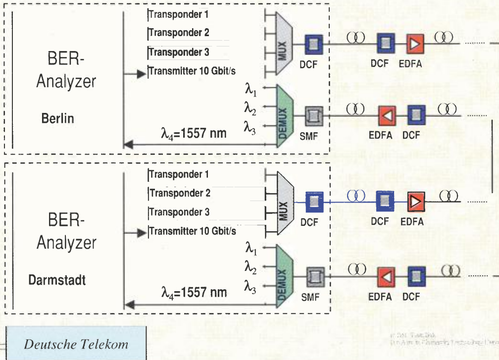
15. 10 Gbit/s transmission experiment
