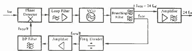
Fig. 2. Block diagram of MMW PLO
