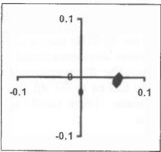
Fig. 9. Phase constellation of I/Q signal
