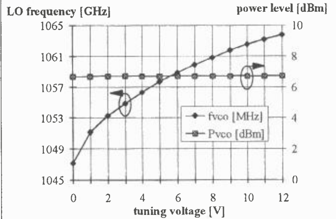
Fig. 5. Frequency and power dependence
