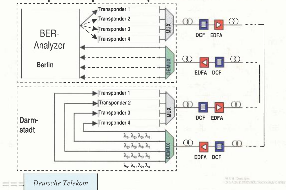
11. Setup of loop back experiment I.
