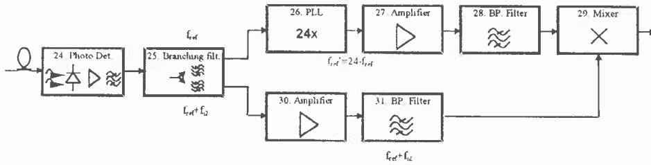
Fig. 4. Block diagram of the optical receiver
