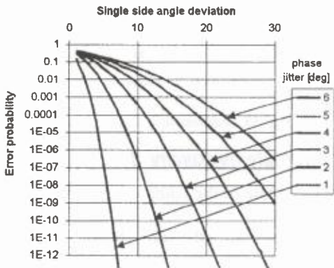
Fig. 10. Error probability versus allowable phase deviation
