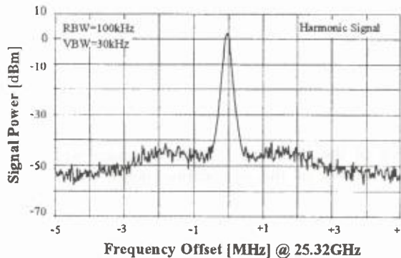
Fig. 7. Spectrum of the MMW signal
