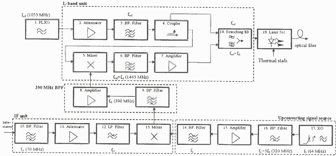
Fig. 3. The block diagram of the optical transmitter
