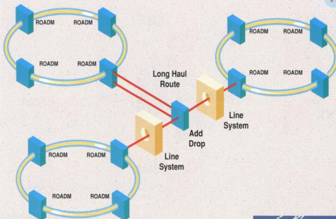
Figure 7. WDM ring based systems
