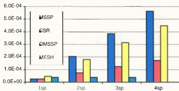
Down time ratio of single STM-1 demand routes in a 8 node network
