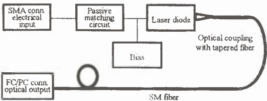
Fig. 11. The modulated laser source
