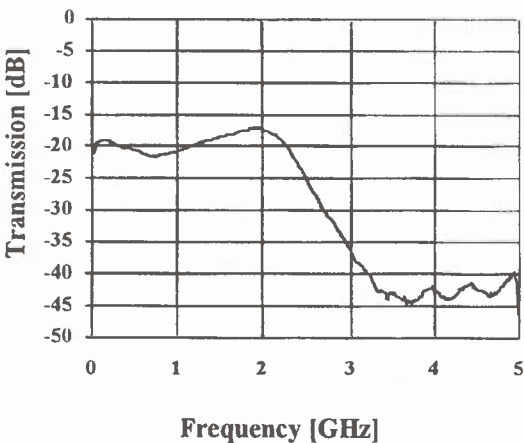
Fig. 12. Overall transfer characteristics of the direct modulated laser
