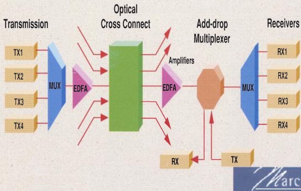
Figure 2. All-optical network
