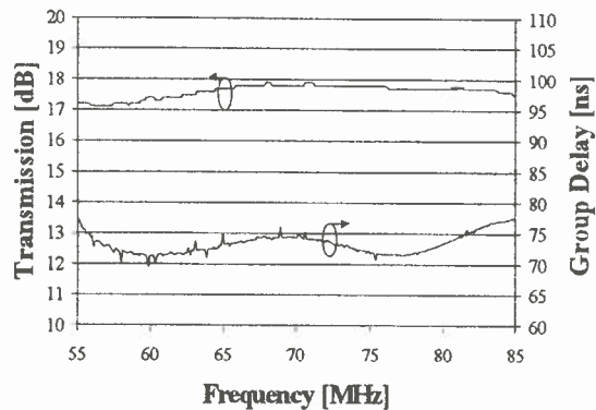
Fig. 13. Transmission measurement
