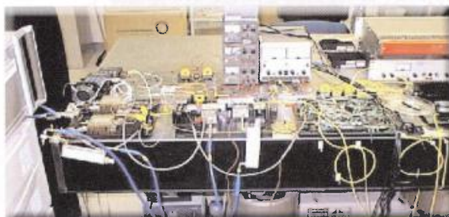
40 Gb/s OTDM Transmitter
