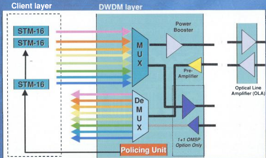
17. Embedded DWDM System
