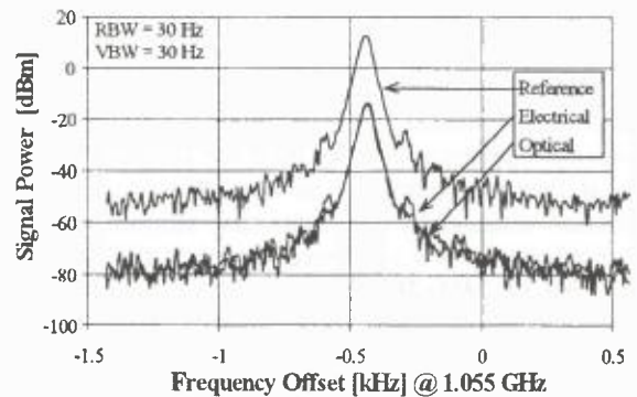
Fig. 6. Spectrum of the reference signal
