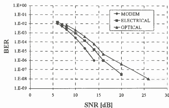
Fig. 14. Bit error rate as a function of the signal-to-noise ratio
