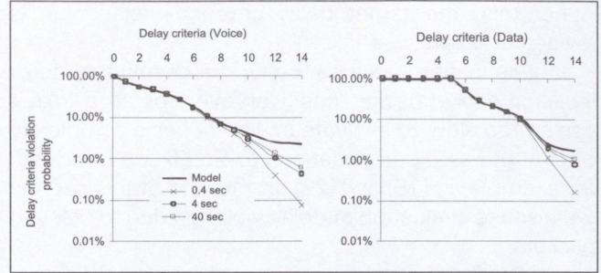
Figure 5. Simulation of delays on a link of capacity C=520 kbps with 15 ms long buffer fed by 30 voice ( TTI_1 = 20 ms, b_1 = 40 bytes, \alpha_1 = 0.6 ) and 2 data ( TTI_2 = 40 ms, b_2 = 360 bytes, \alpha_2 = 1 ) connections
