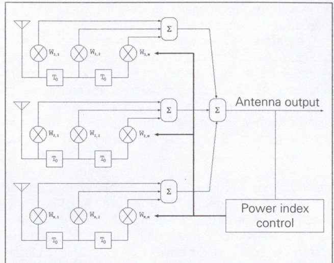
Figure 3. Smart antenna model
