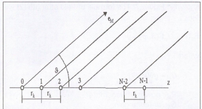
Figure 6. Antenna row
