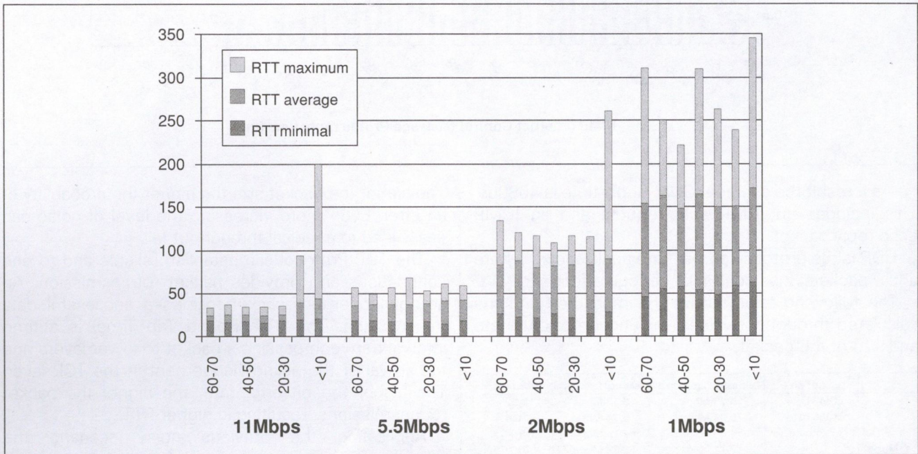
Round Trip Time versus different SNR and data rate
