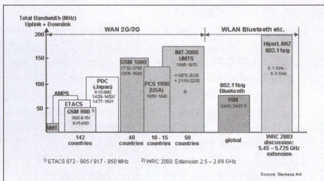
Figure 7. Available Spectrum for 2G/3G Services and WLANs
