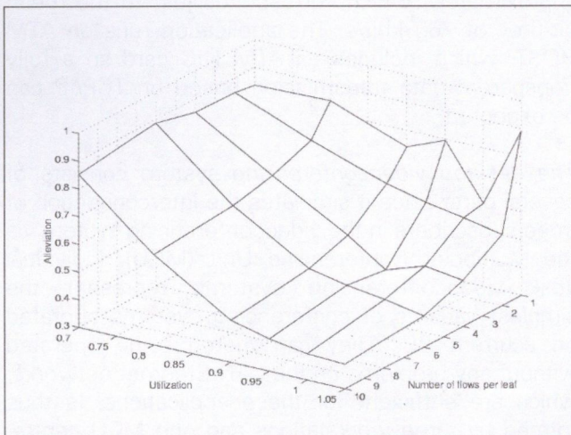
Figure 7. The alleviation versus utilisation.
