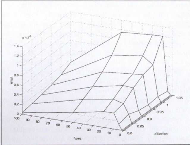
Figure 4. The estimation error of fluid simulation
