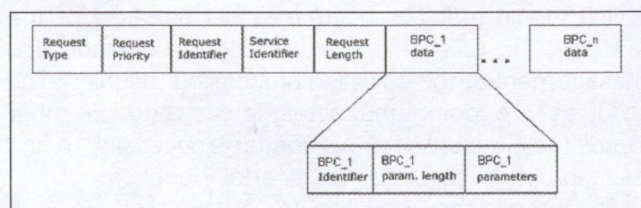
Figure 5. A reconfiguration request
