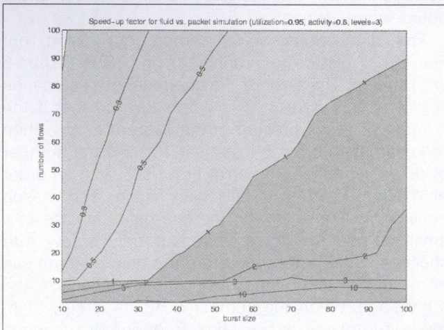
Figure 5. Contour plot of the speed-up factor
