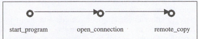
Figure 2. Graph representation of a must precede relation
