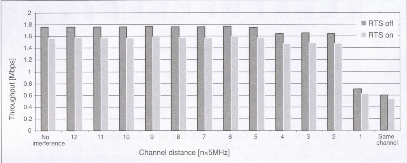
Throughput vs. Interference at 2Mbps
