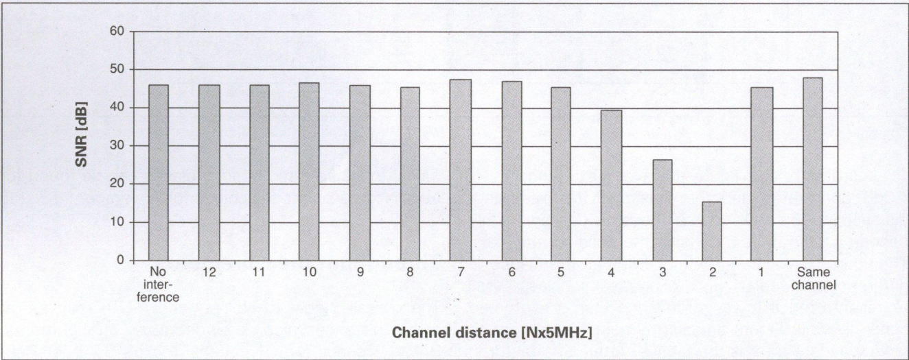
SNR vs Interference
