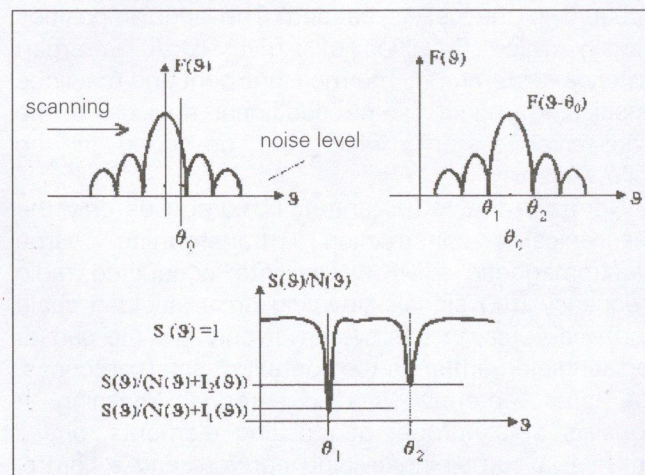
Figure 5. DoA estimating methods
