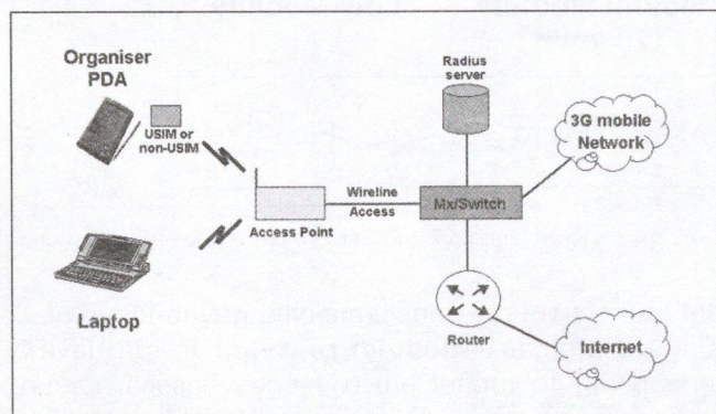
Figure 6. WLAN Connection to Backbone Networks
