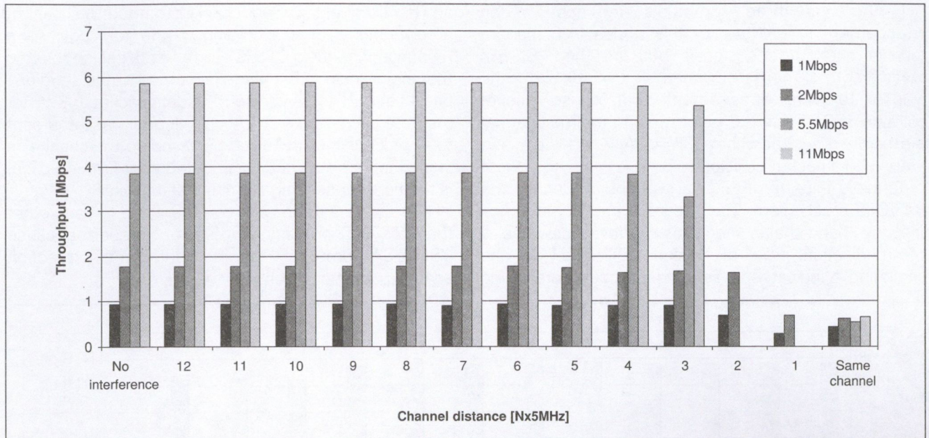
Throughput vs. interference
