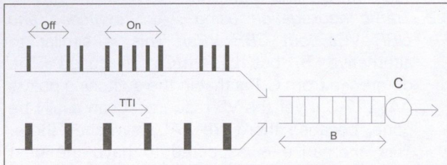
Figure 4. System fed by two periodic ON-OFF connections with different TTIs and packet sizes
