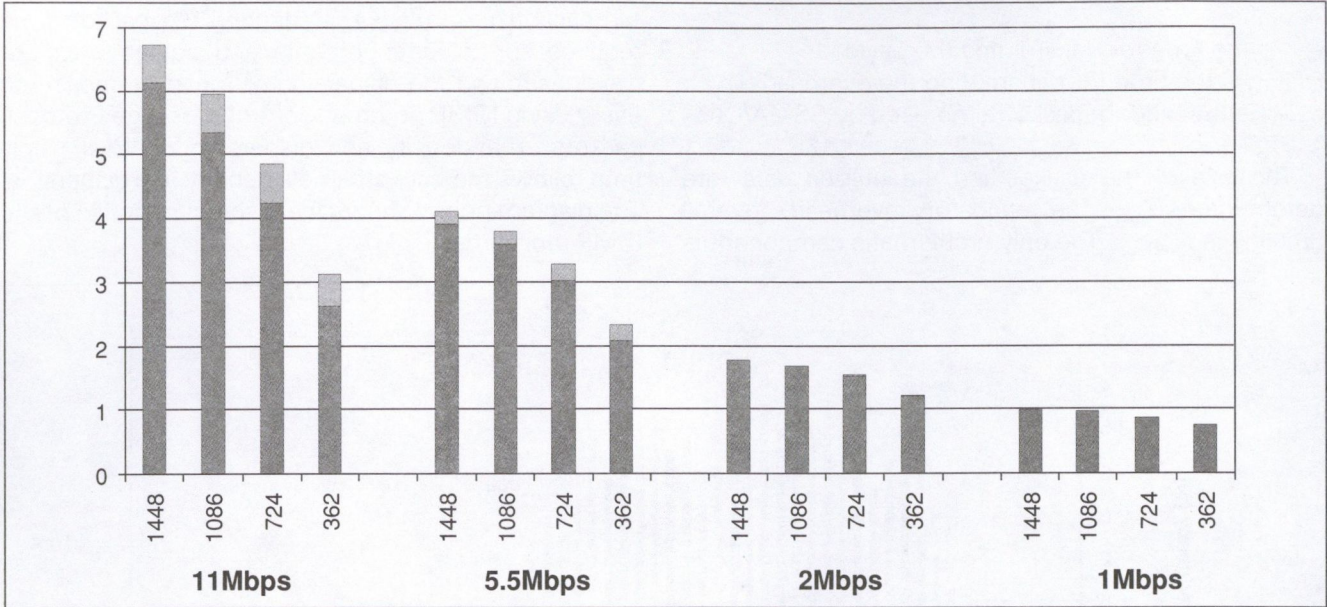
UDP throughput versus different packet size and data rate
