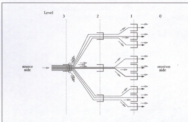
Figure 3. Rate updates in a tree topology network
