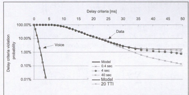
Figure 6. Simulation of delays. Model parameters are the same as in Figure 5, s = 47 bytes, voice has higher priority than data
