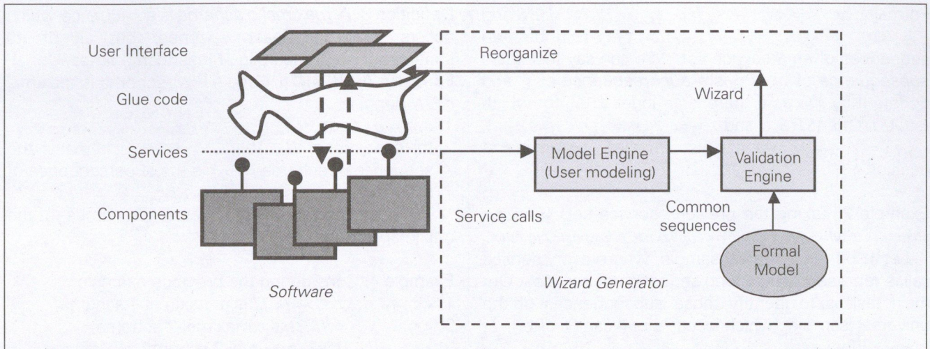
Figure 1. Basic Architecture of Automatic Wizard Generation
