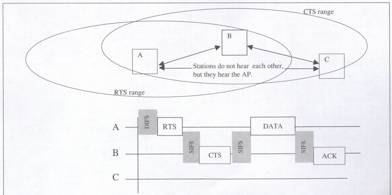
Hidden terminal problem and RTS-CTS mechanism
