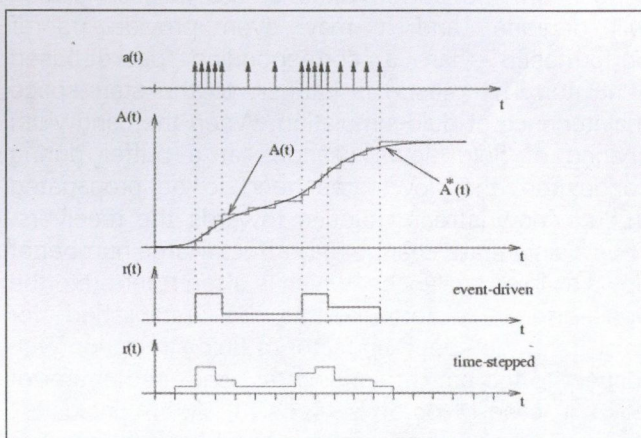
Figure 1. The origin and the description of fluid models
