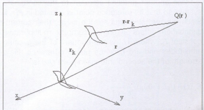
Figure 7. Model for calculations
