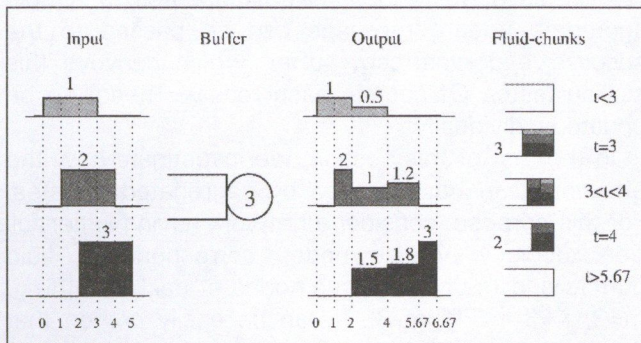
Figure 2. Visualisation of buffer dynamics
