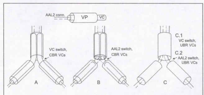
Figure 3. ATM/AAL2 switching alternatives in UTRAN
