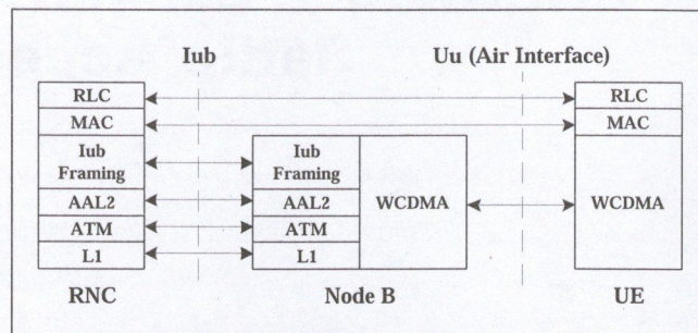
Figure 2. ATM/AAL2 based UTRAN protocol stack
