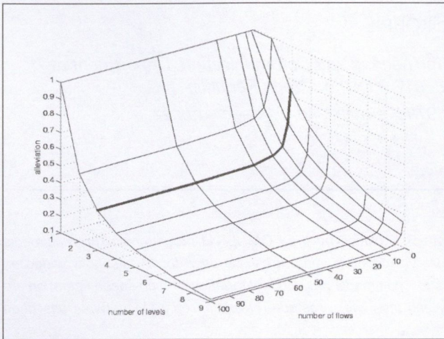
Figure 6. The alleviation of the aggregated updates
