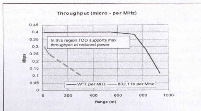
Figure 5. Throughput for Single Cell – Micro Deployment UMTS/TDD vs. 802.11b
