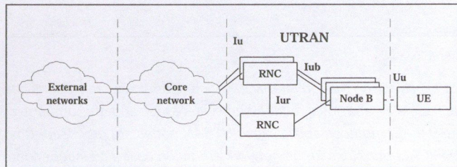
Figure 1. UMTS network architecture
