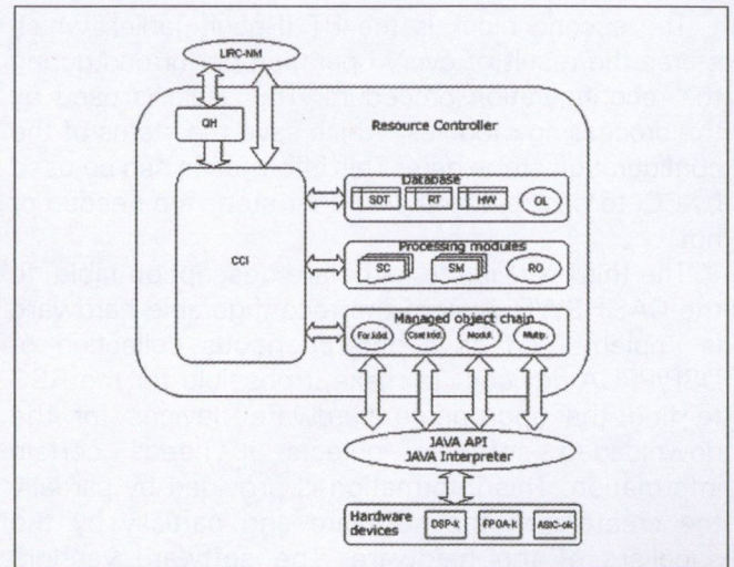
Figure 3. The CAST Resource Controller
