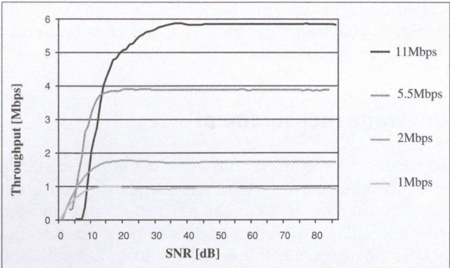
Throughput vs SNR
