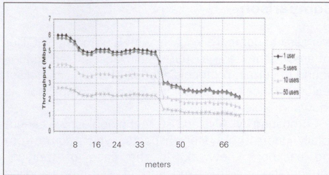
Figure 4. Performance of 802.11b in Hot Spot (Nomadic/Non-Contiguous Coverage)
