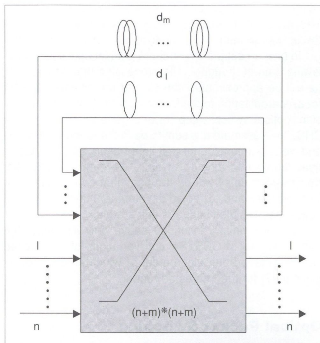
Figure 5. Single-stage, feedback optical storage
