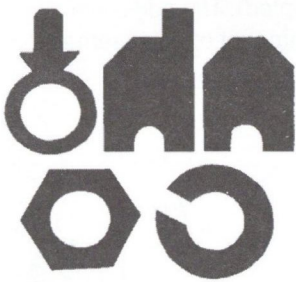
Figure 9. Image thresholding
