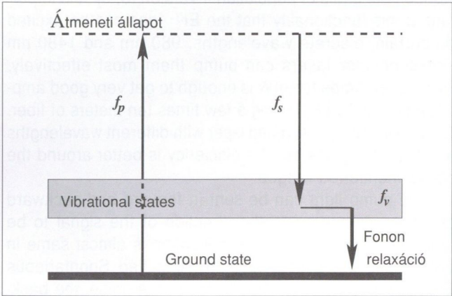
Figure 3. Energy-level diagram of Raman scattering
