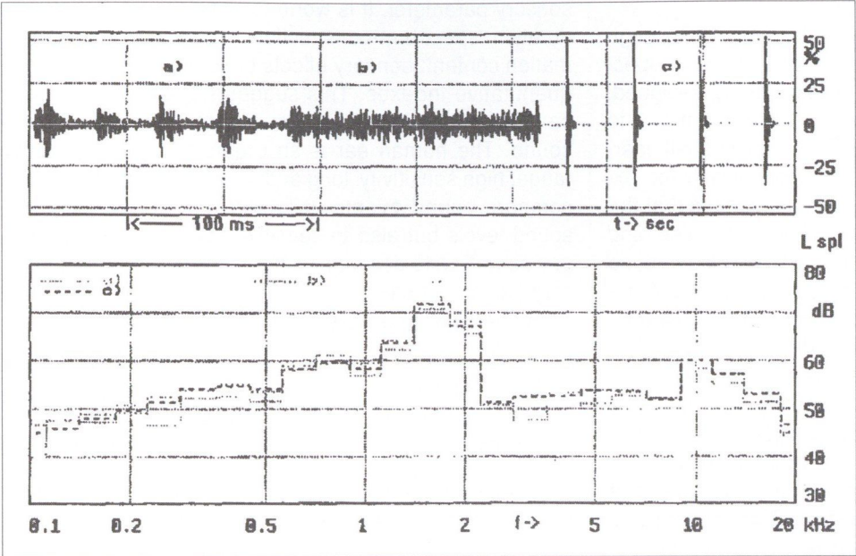
Figure 1. Three different sound signal: dies engine noise (a), pink noise (b) and series of square pulse (c) and their 1/3 octave spectrum producing nearly identical LA levels [7]
