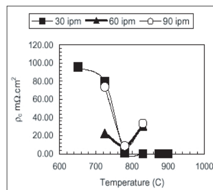
Firing temperature and belt speed effect to the contact resistivity
