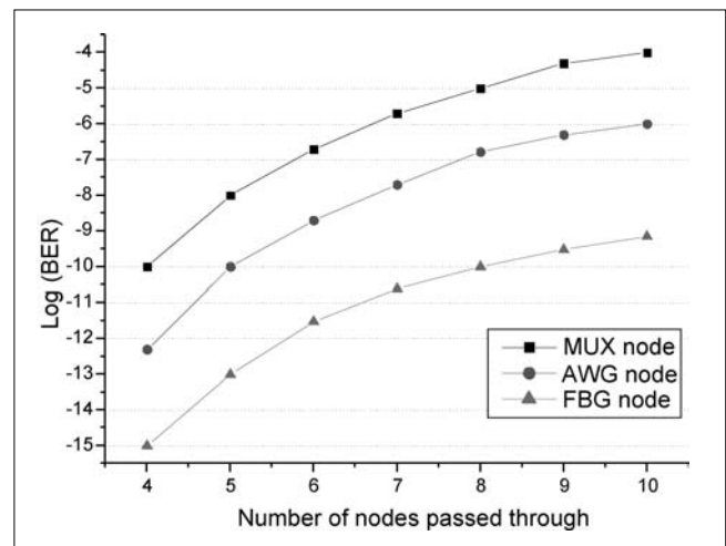
Fig. 5. Number of crossed optical nodes vs. BER foreseen: a. mux/demux based, b. AWG based, c. FBG based
