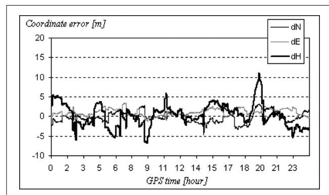
Fig. 3. Errors of single point positioning at BUTE station (16th June, 2002, local ionosphere models)
