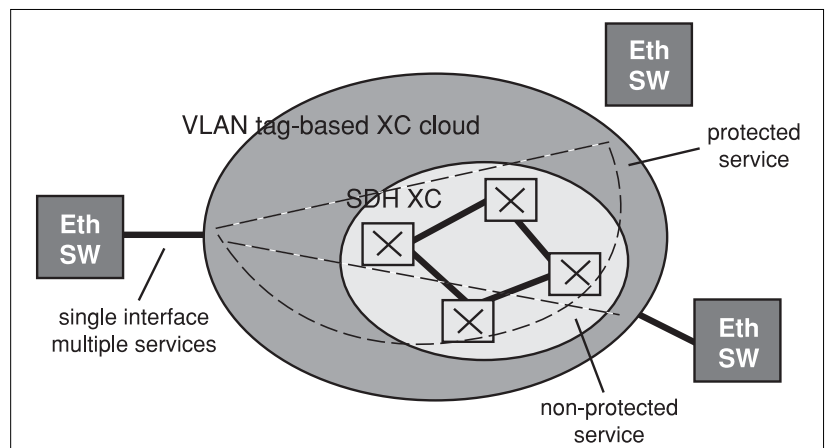
Fig. 1. Network architecture
