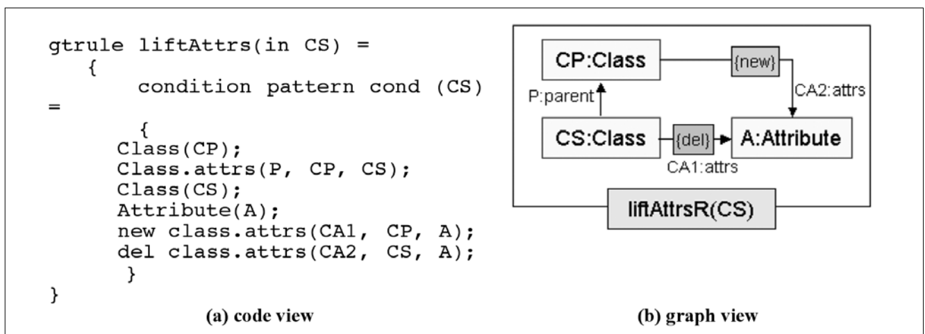
Figure 3. The GT rule liftAttrs
