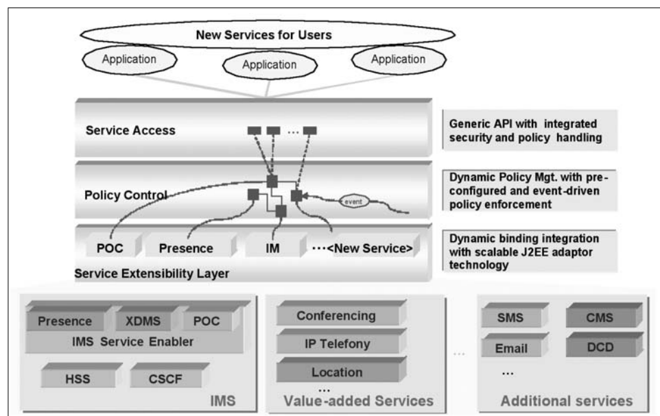
Figure 5. Architecture of the Service Integration Environment (SIE)
