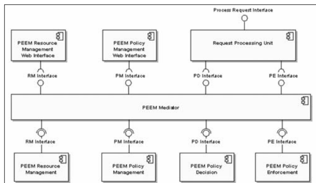
Figure 7. Policy Control Component overview
