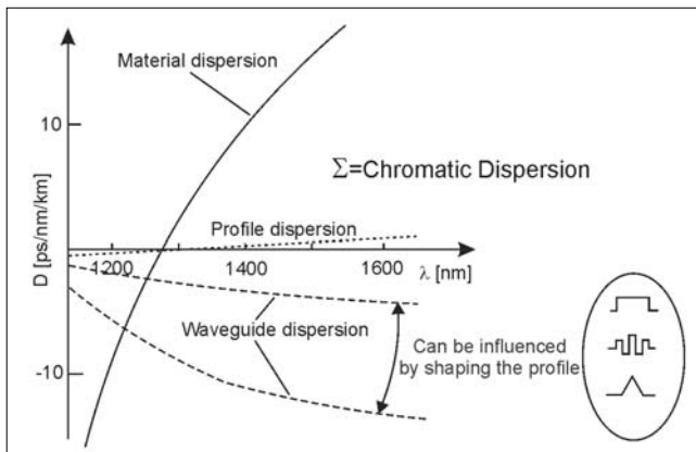
Figure 3. Chromatic dispersion
