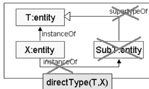
Figure 5. The directType GT pattern
