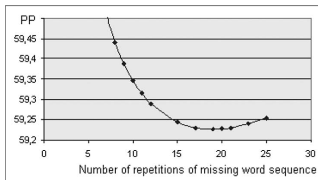
Figure 2.2. Perplexity for control set depending on the number of repetition of missing word sequences
