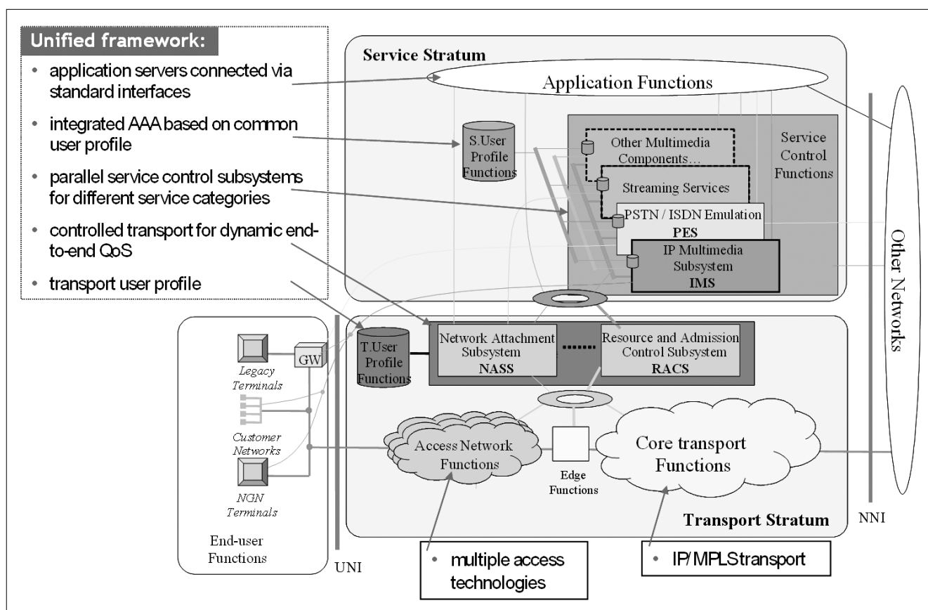
Figure 2. Overall NGN architecture
