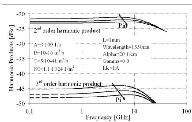
Figure 3. Second and third order harmonics
