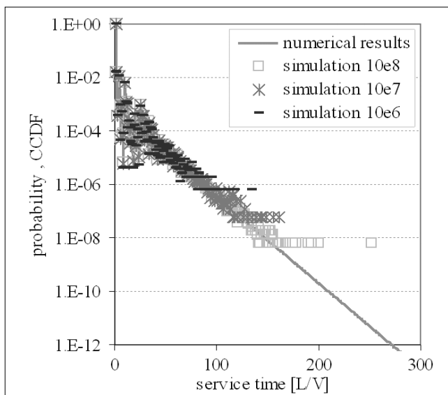
Figure 3. The numerical and simulation results of the service time
