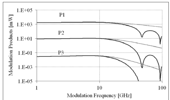
Figure 5. Mismatch between the microwave and the light propagation velocities
