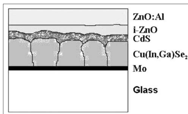
Figure 3. Schematic cross-section of a \text{CuInGaSe}_2 solar cell structure
