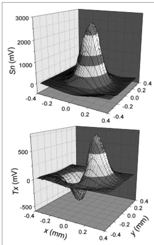
Figure 6. Two components of the stress profile inside the elastic cover at a given depth, generated by the simplest point load on the surface. The measurement results correlate well with the theoretical predictions.
