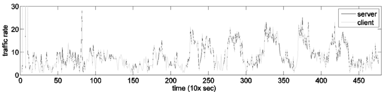
Figure 3. Eve Online measured traffic intensity (packets/10 sec), selected interval: 50-450
