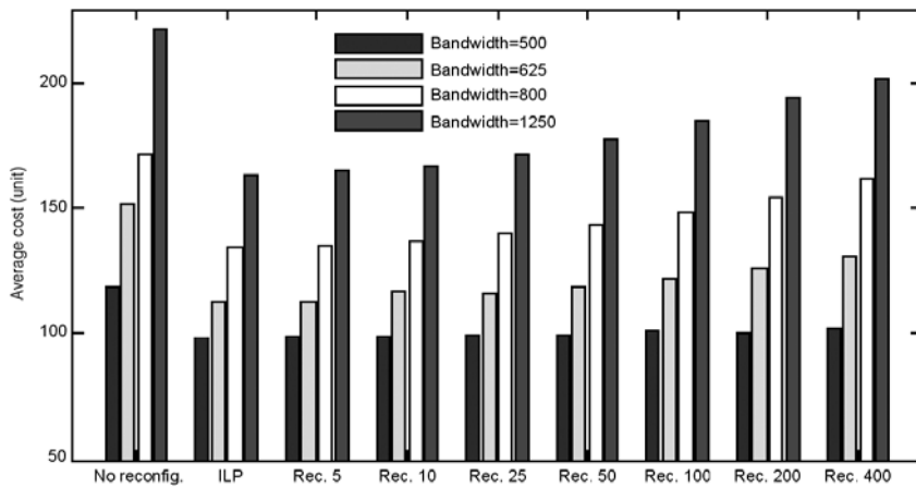
Figure 9. Average routing cost for different bandwidth of demands
