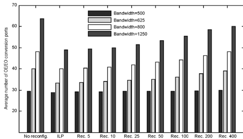
Figure 10. Average number of converter ports (O/E, E/O) for different bandwidth of demands
