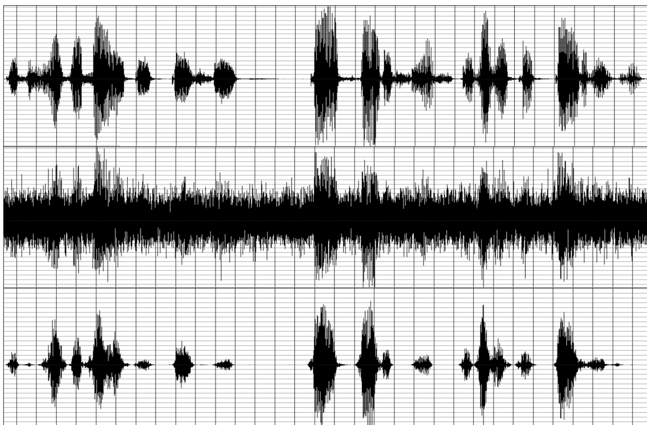
Figure 1. Noise suppression in case of -3 dB and white noise in case of the same parameters as in Table 1. (upper trace: original utterance, middle trace: noise speech, lower trace: enhanced speech)
