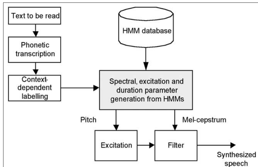
Figure 3. Speech generation with HMMs
