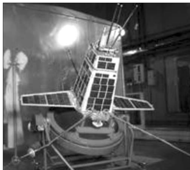
Figure 1. The Compass-2 during the final phase of the ground tests
