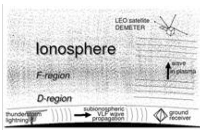
Figure 9. The generation mechanism and propagation path of spiky whistlers (SpW) [5]
