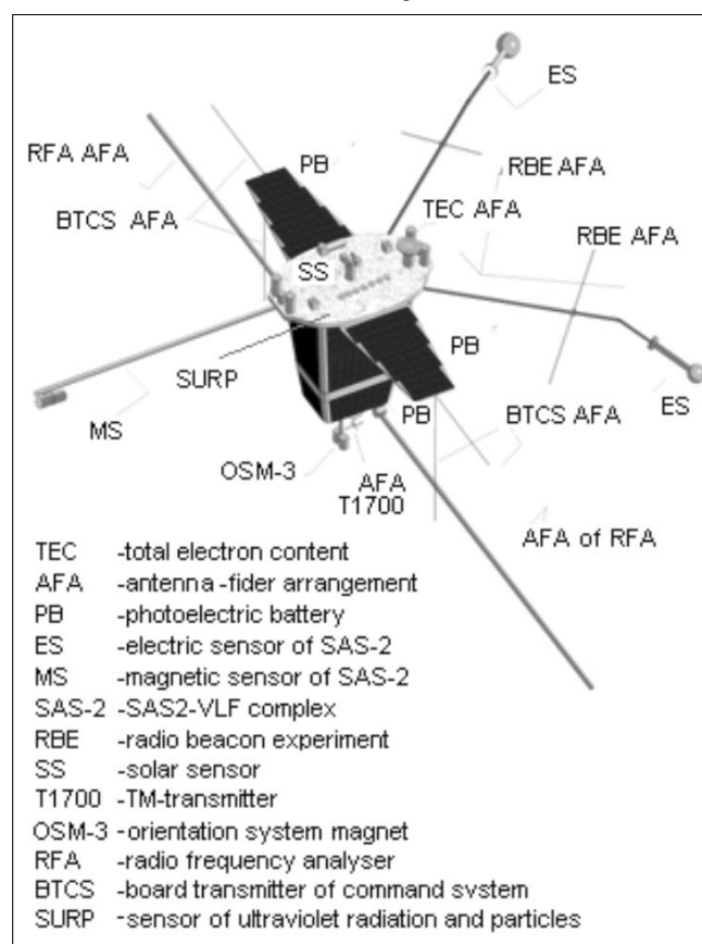
Figure 2. The sketch of the Compass-2 satellite. The sensors of the SAS2-K2 are the two ES electric and the MS magnetic Ukrainian sensors.
