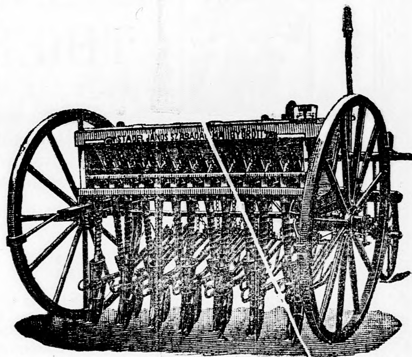
Győri Drill.
