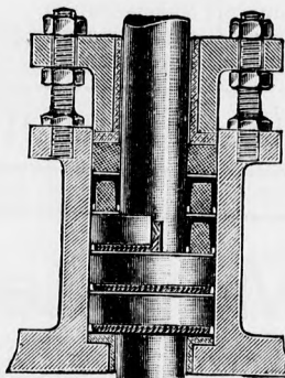
Goetze-Metall-Manschetten-Packung.
